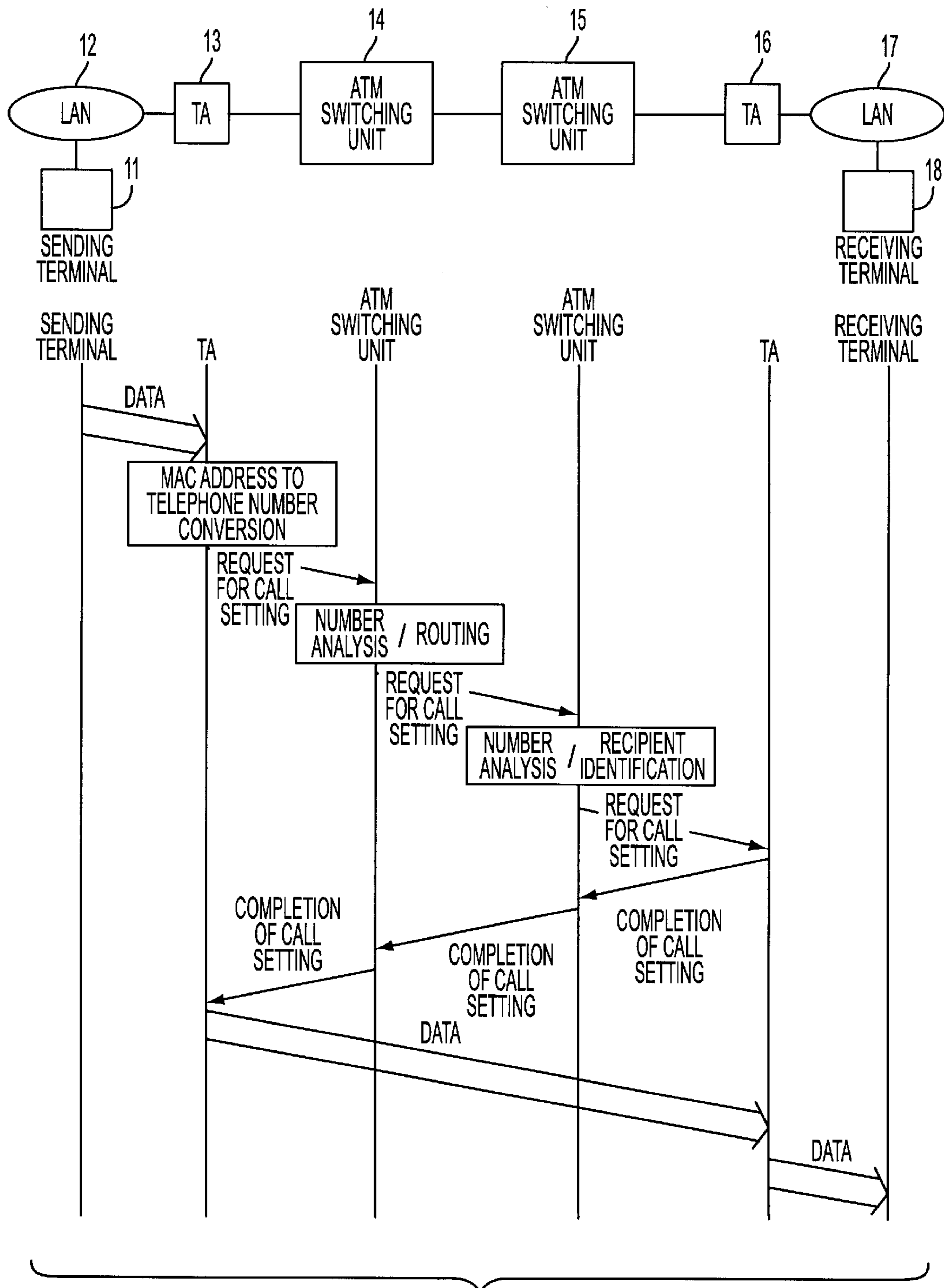
FIG. 3 (PRIOR ART)
