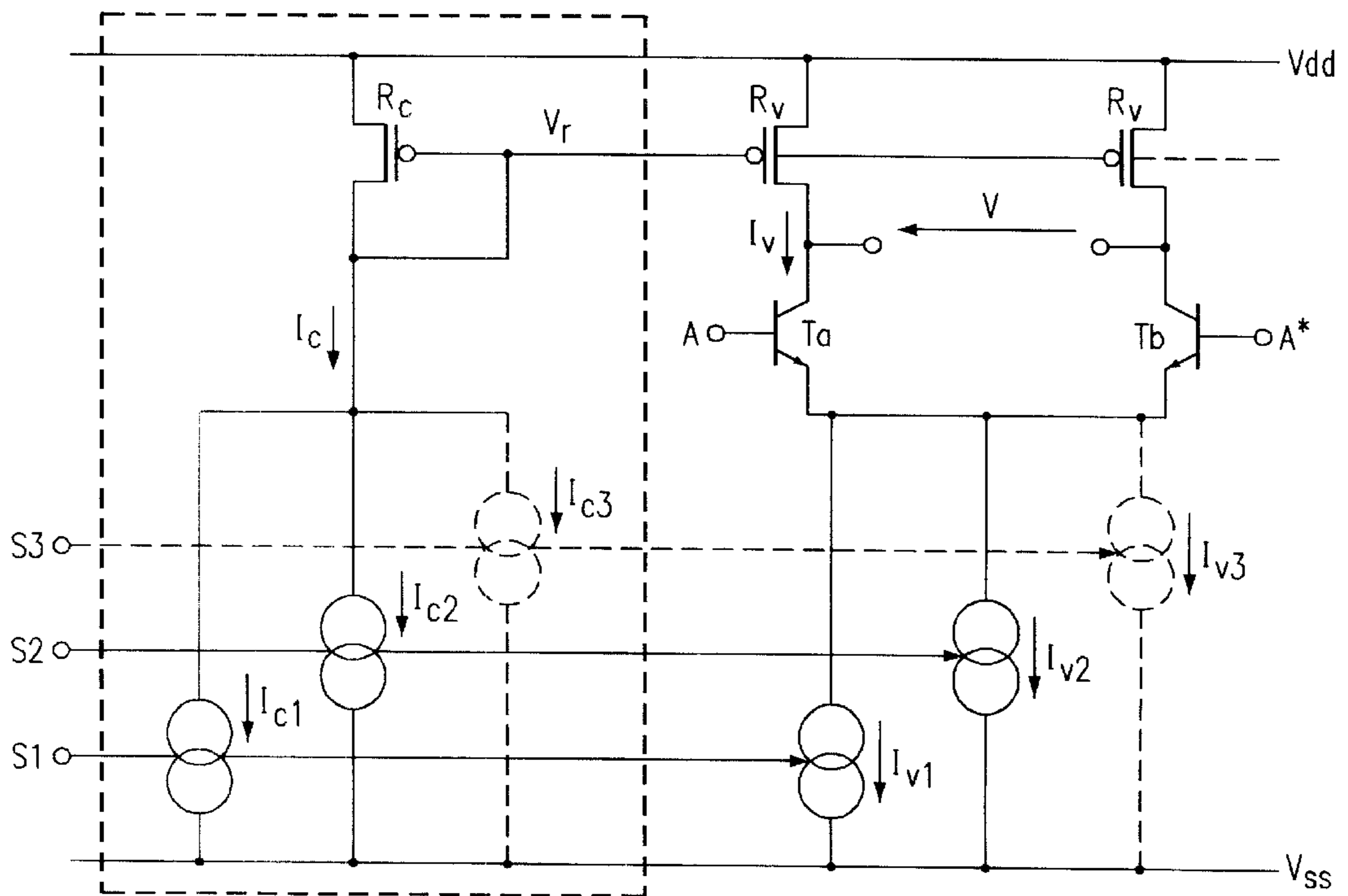
FIG. 2 (PRIOR ART)
