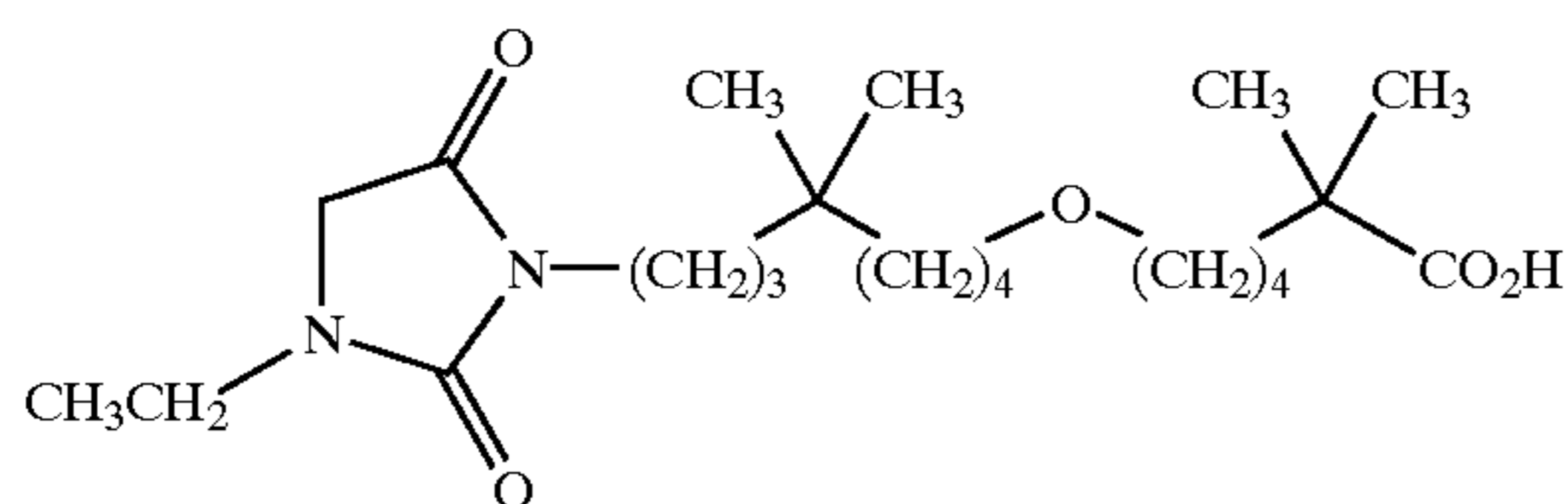
6-[8-(3-ethyl-2,5-dioxo-imidazolidin-1-yl)-5,5-dimethyloctyloxy]-2,2-dimethyl-hexanoic acid;
