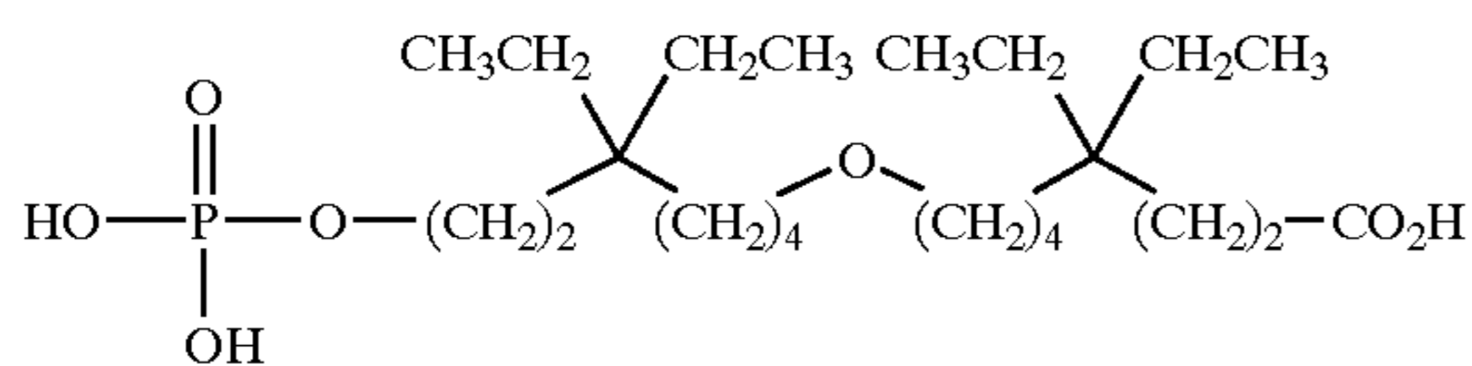
8-(5,5-diethyl-7-phosphonoxy-heptyloxy)-4,4-diethyl-octanoic acid;
