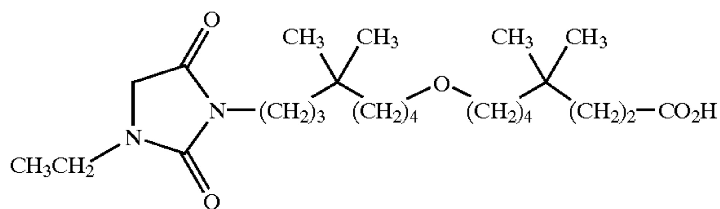
8-[8-(3-ethyl-2,5-dioxo-imidazolidin-1-yl)-5,5-dimethyloctyloxy]-4,4-dimethyl-octanoic acid;
