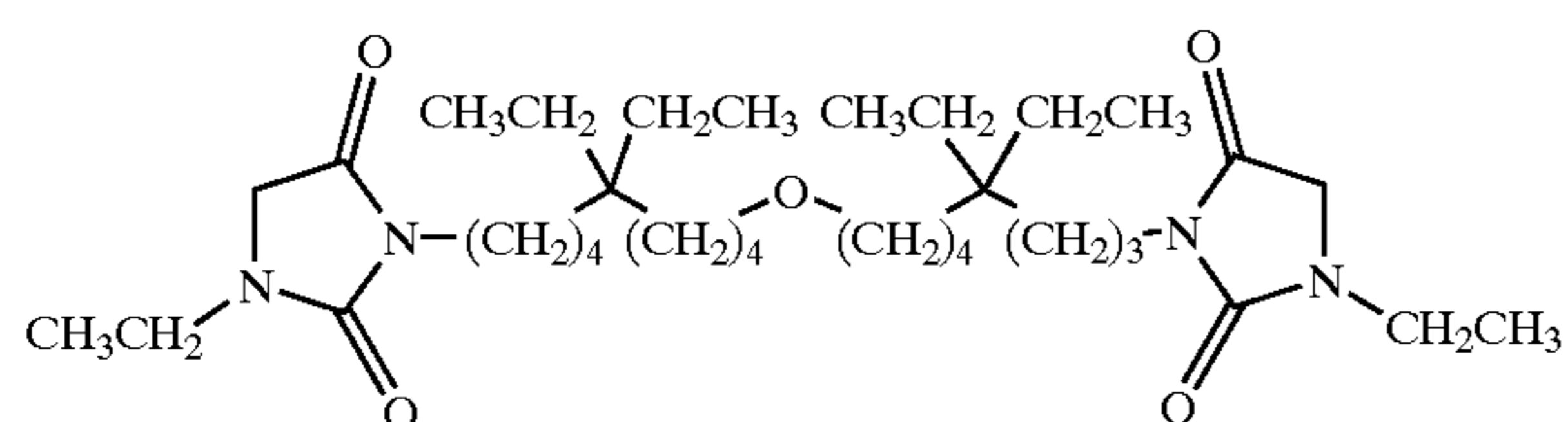
3-[8-(9-(3-ethyl-2,5-dioxo-imidazolidin-1-yl)-5,5-diethyl-nonyloxy)-4,4-diethyl-octyl]-1-ethyl-imidazolidine-2,4-dione;
