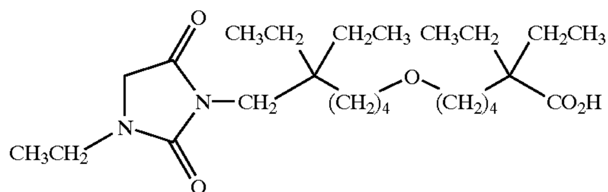
2,2-diethyl-6-[5-ethyl-5-(3-ethyl-2,5-dioxo-imidazolidin-1-ylmethyl)-heptyloxy]-hexanoic acid;
