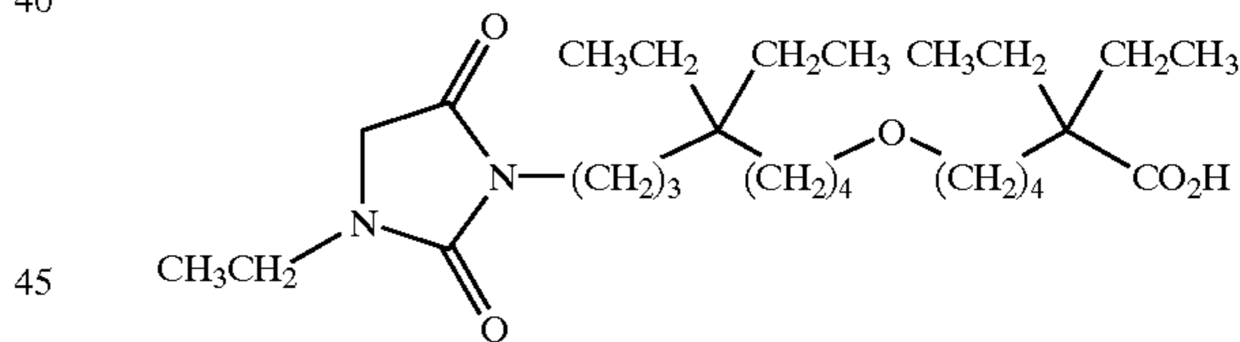
6-[5,5-diethyl-8-(3-ethyl-2,5-dioxo-imidazolidin-1-yl)-octyloxy]-2,2-diethyl-hexanoic acid;
