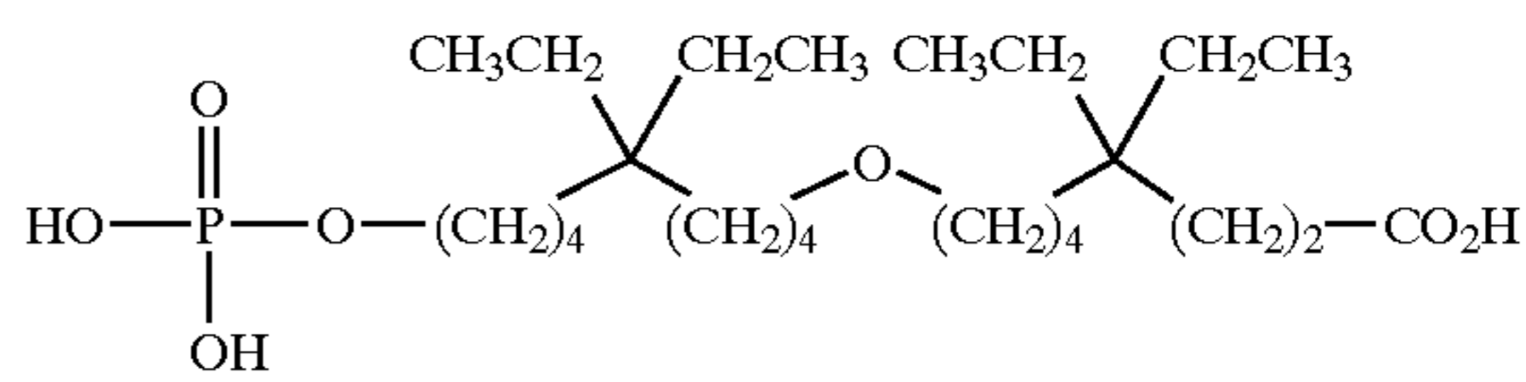
8-(5,5-diethyl-9-phosphonoxy-nonyloxy)-4,4-diethyl-octanoic acid;
