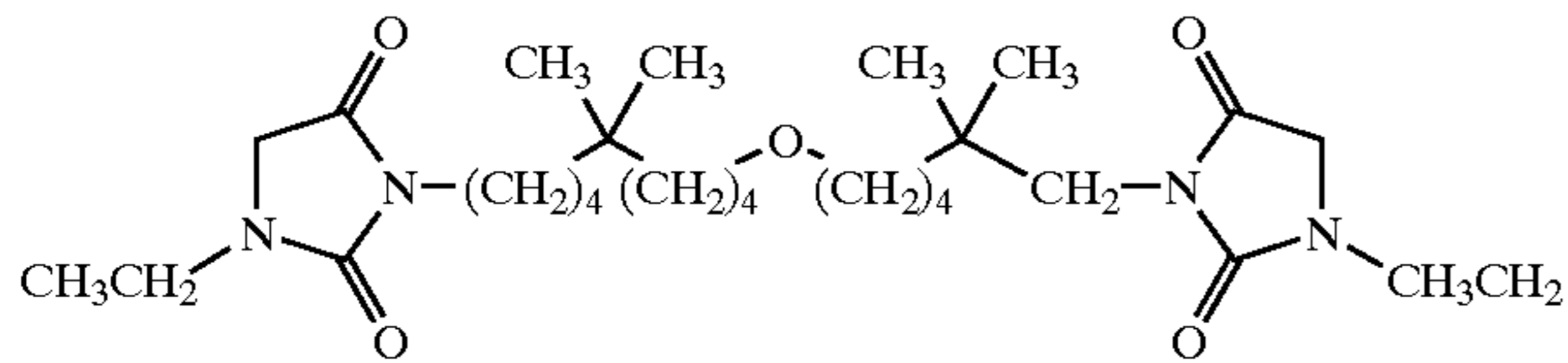
3-[6-(9-(3-ethyl-2,5-dioxo-imidazolidin-1-yl)-5,5-dimethyl-octyloxy)-2,2-dimethyl-hexyl]-1-ethyl-imidazolidine-2,4 dione;
