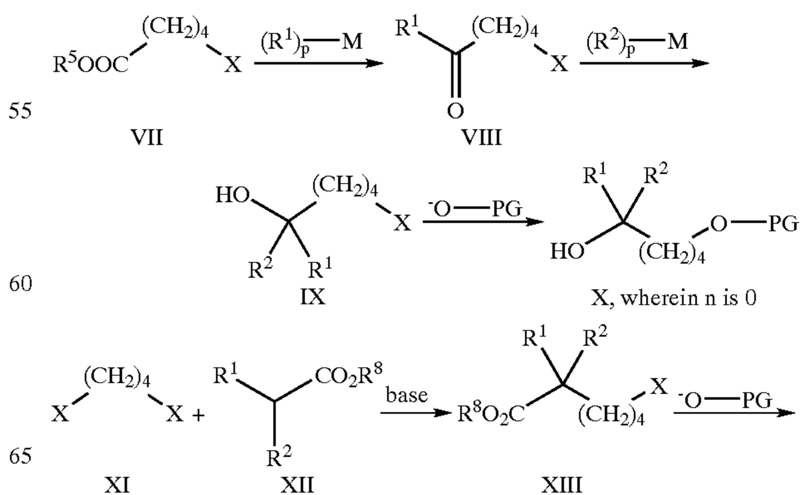
SCHEME 1: Synthesis of compounds of formula X
