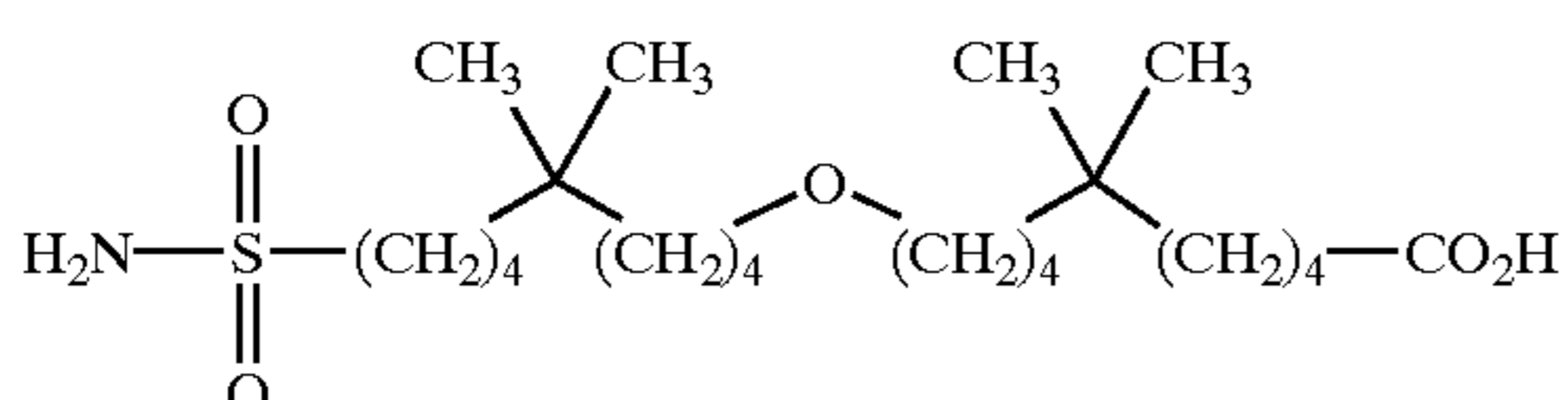
10-(5,5-dimethyl-9-sulfamoyl-nonyloxy)-6,6-dimethyl-decanoic acid;
