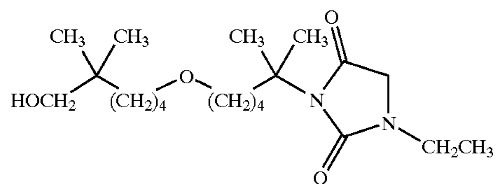
1-ethyl-3-[5-(6-hydroxy-5,5-dimethyl-hexyloxy)-1,1-dimethyl-pentyl]-imidazolidine-2,4-dione;
