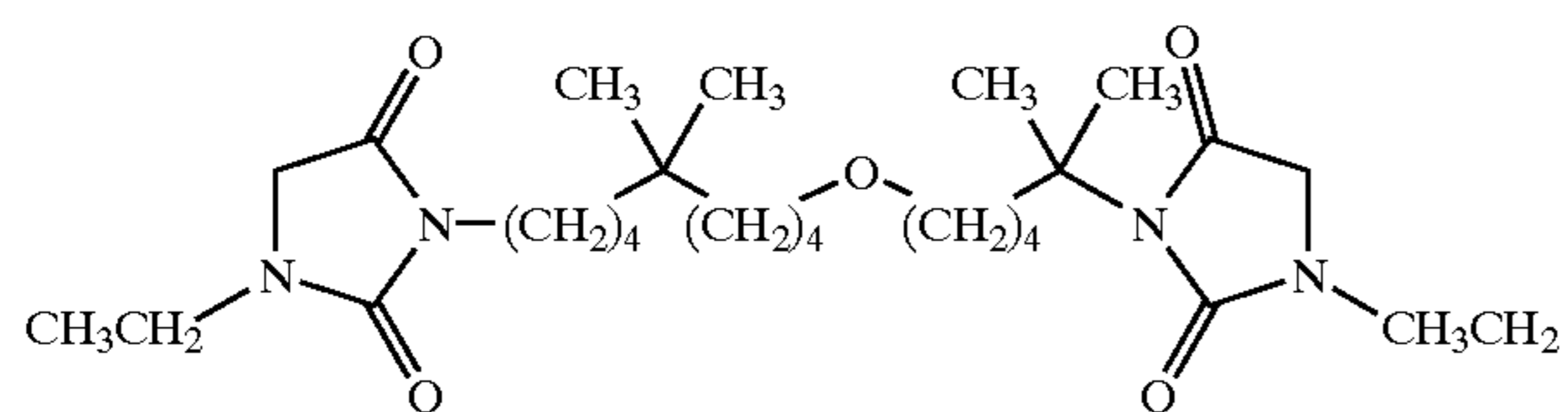
3-[5-(9-cyclopentyl-5,5-dimethyl-nonyloxy)-1,1-dimethyl-pentyl]-1-ethyl-imadazolidine-2,4-dione;
