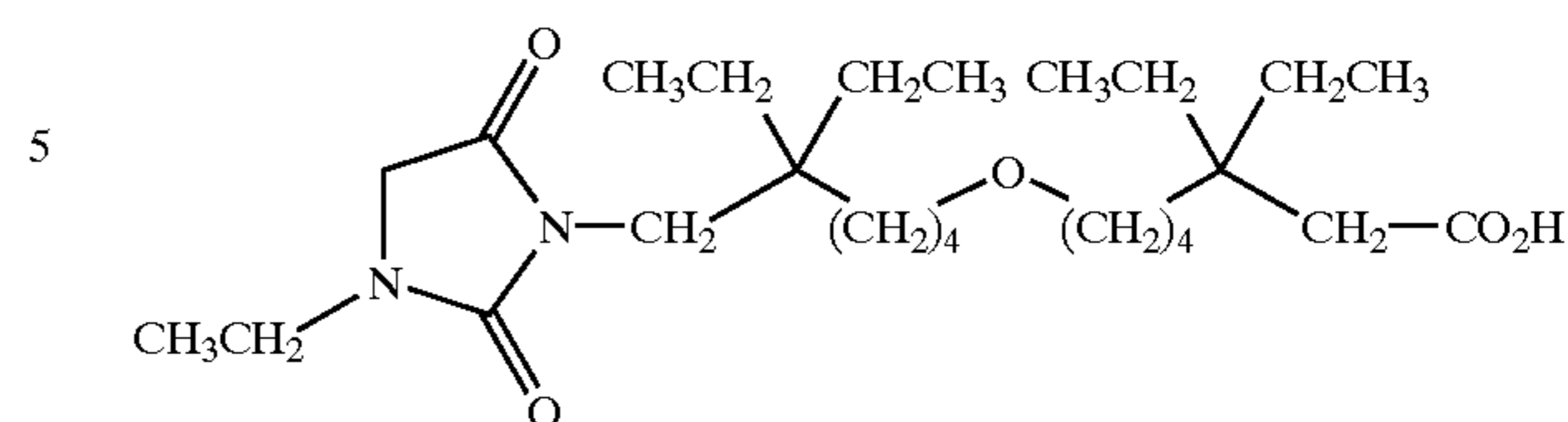
2,3-diethyl-7-[5-ethyl-5-(3-ethyl-2,5-dioxo-imidazolidin-1-ylmethyl)-heptyloxy]-heptanoic acid;
