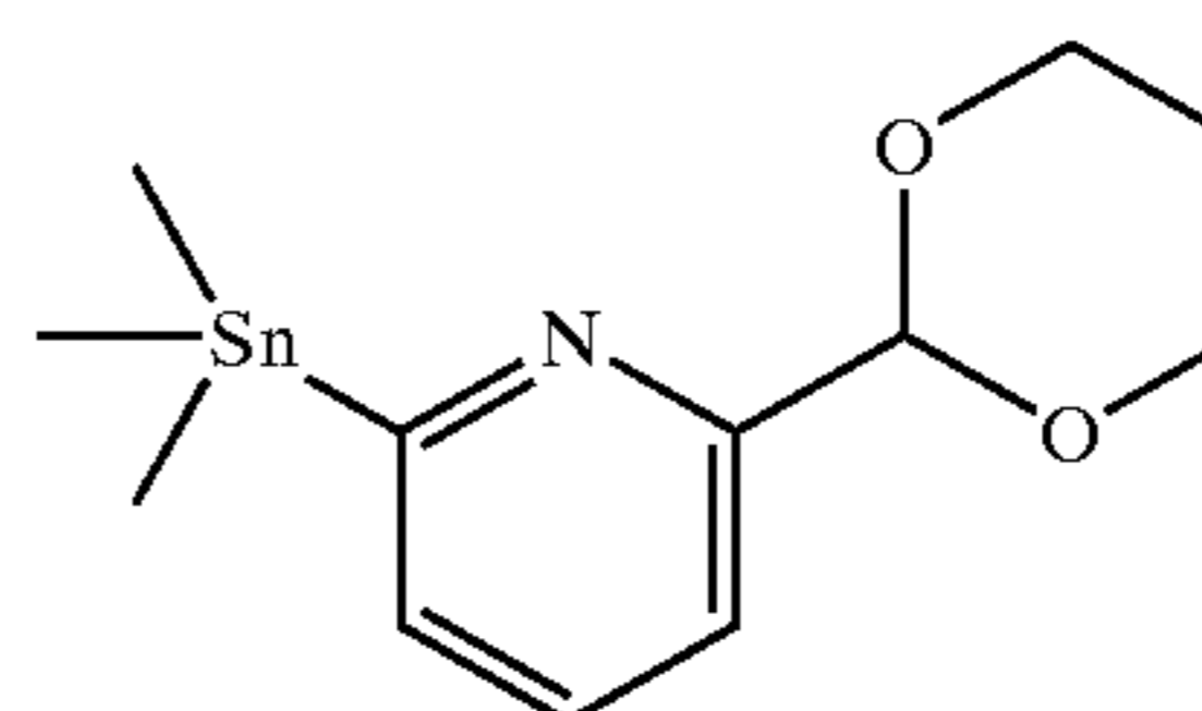
2-(1,3-Dioxan-2-yl)-6-trimethylstannylpyridine
