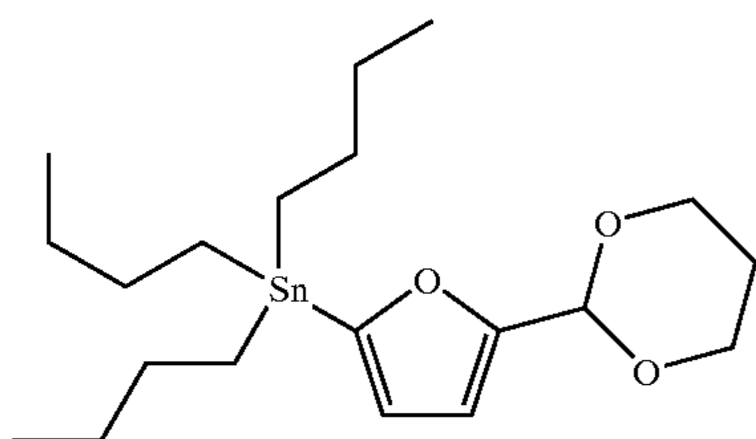
5-(1,3-Dioxan-2-yl)-2-tributylstannyl-furan
