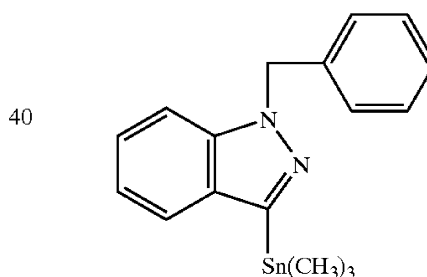
1-Benzyl-3-trimethylstannylindazole
