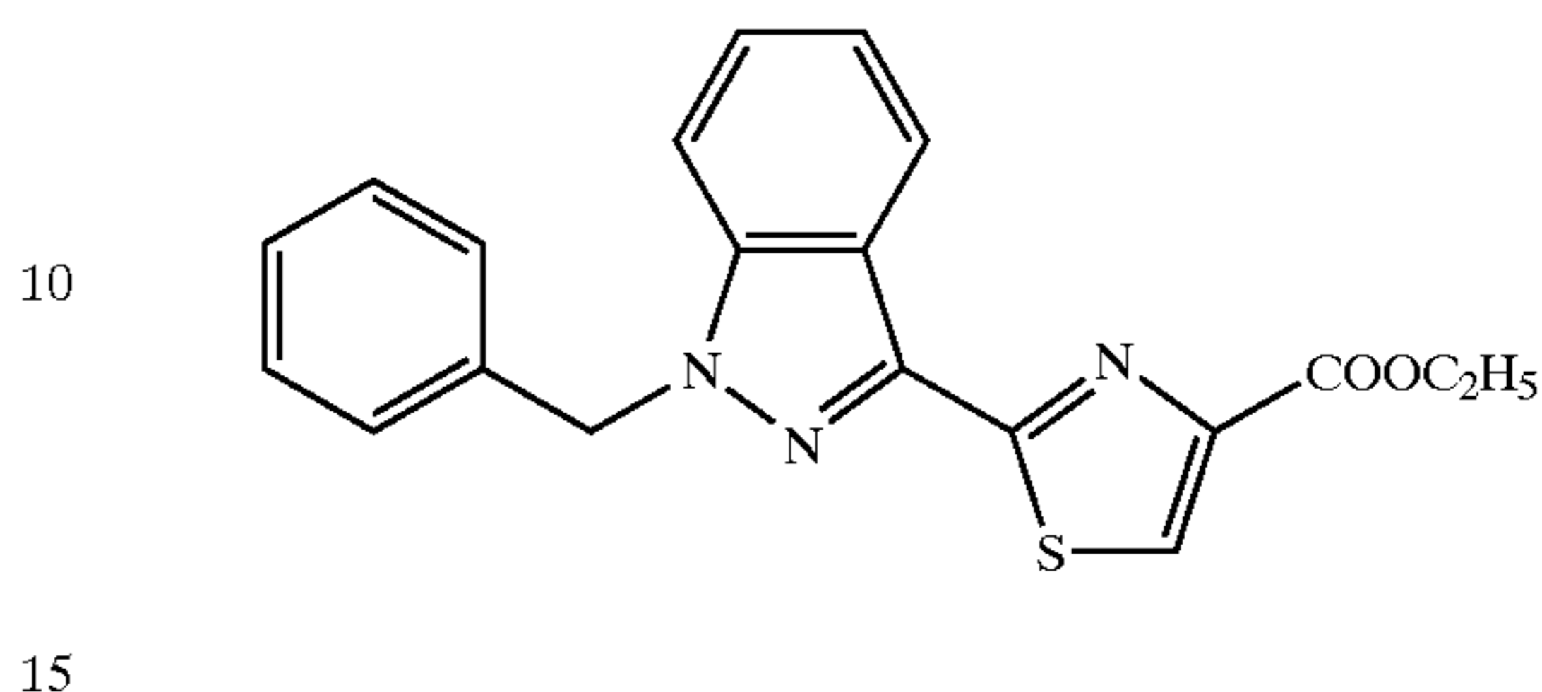
Ethyl 2-(1-benzyl-indazol-3-yl)-thiazole-4-carboxylate
