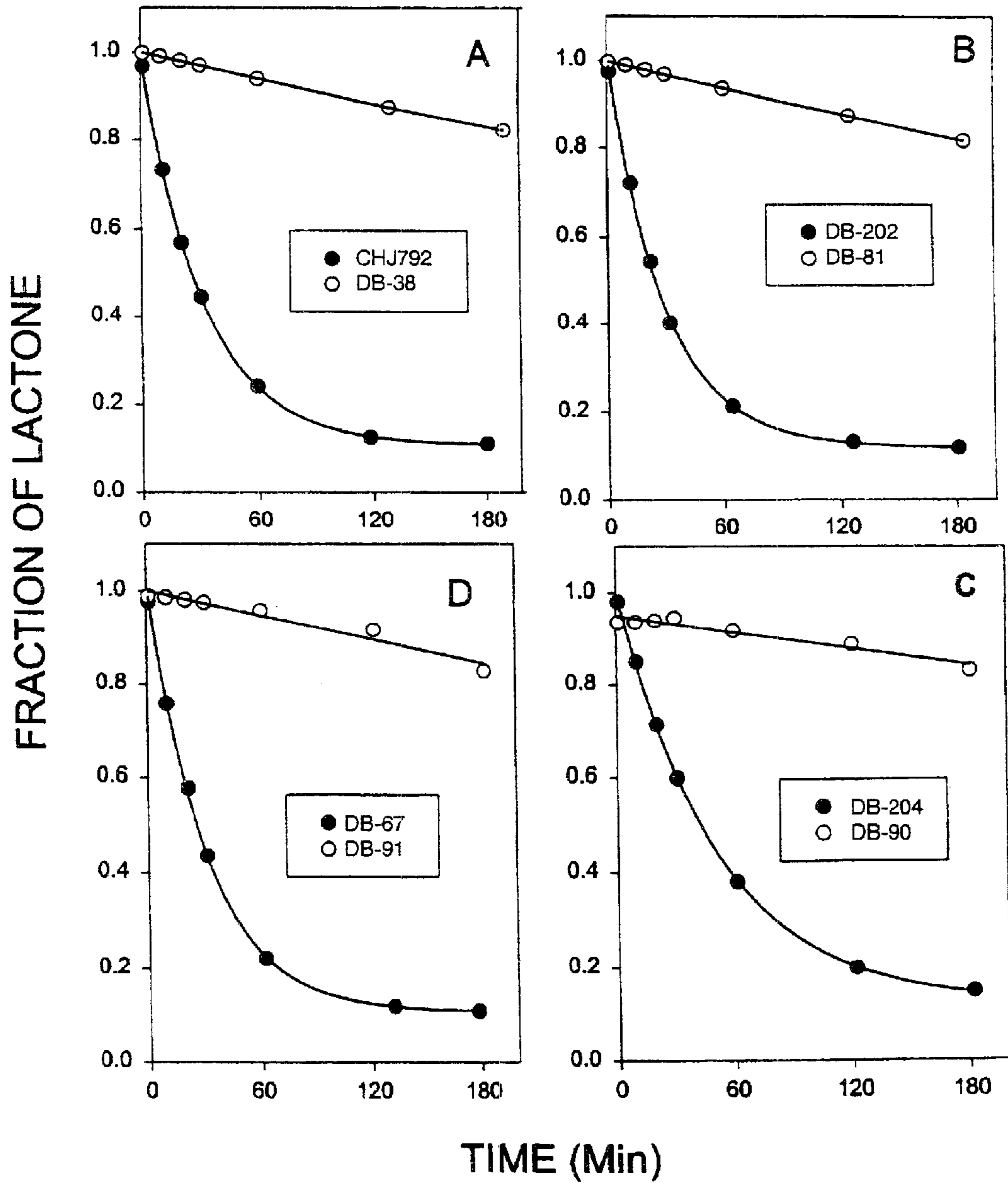
Comparison of the Stabilities of \alpha -Lactone Silatecans with their corresponding Homosilatecans in PBS Buffer at 37°C
