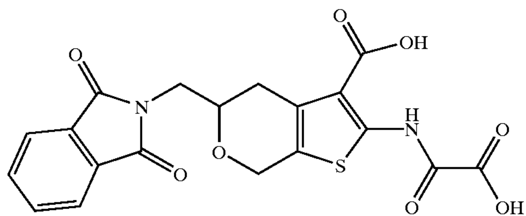
5-(1,3-Dioxo-1,3-dihydro-isoindol-2-ylmethyl)-2-(oxalyl-amino)-4,7-dihydro-5H-thieno[2,3-c]pyran-3-carboxylic Acid
