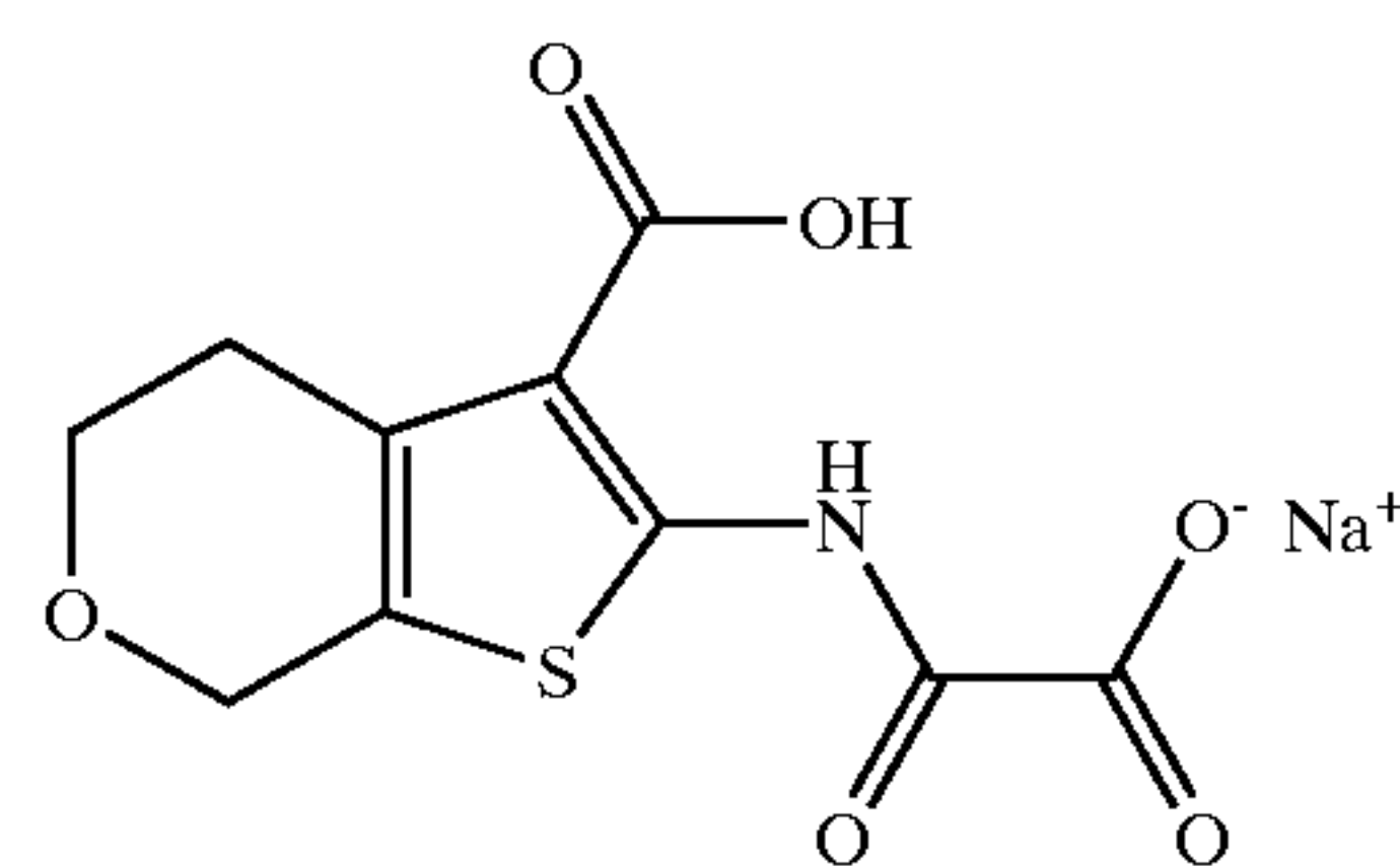
2-(Oxalyl-amino)-4,7-dihydro-5H-thieno[2,3-c]pyran-3-carboxylic Acid, Mono Sodium Salt
