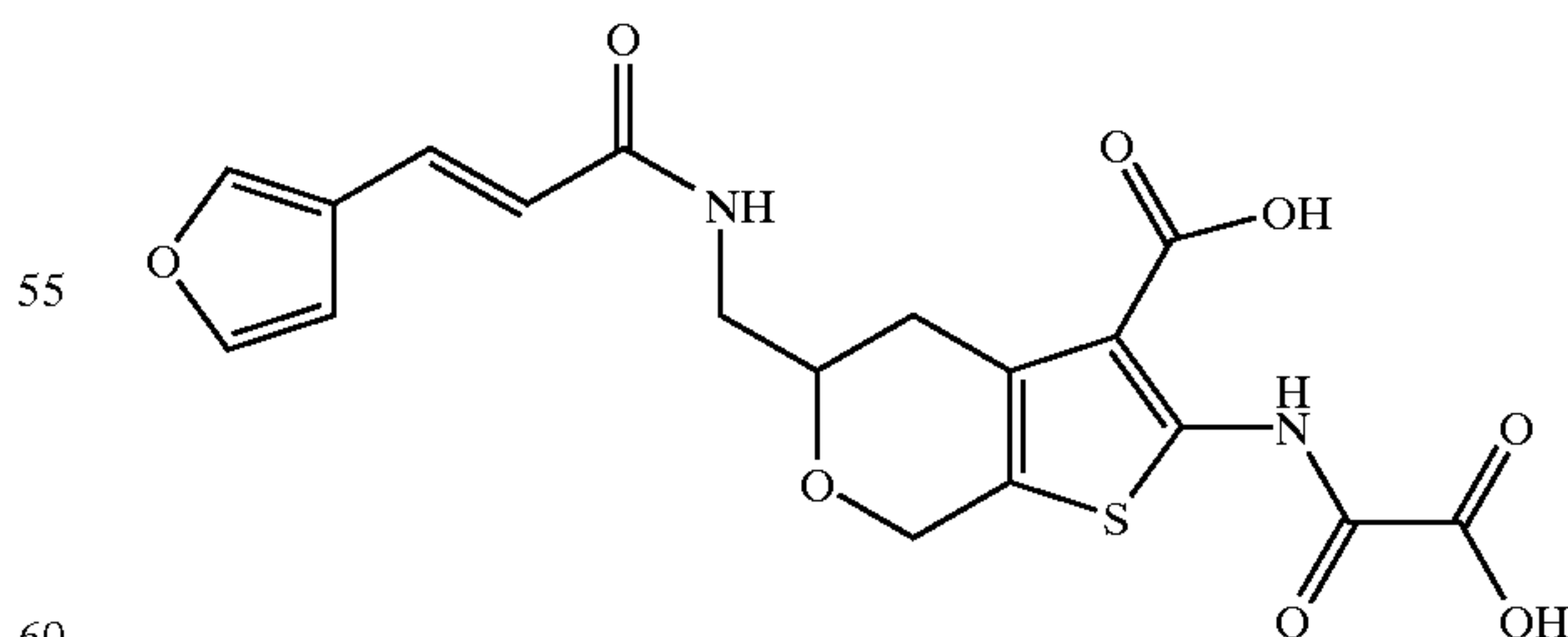
5-(((3-Furan-3-yl-acryloylamino)-methyl)-2-(oxalyl-amino)-4,7-dihydro-5H-thieno[2,3-c]pyran-3-carboxylic Acid
