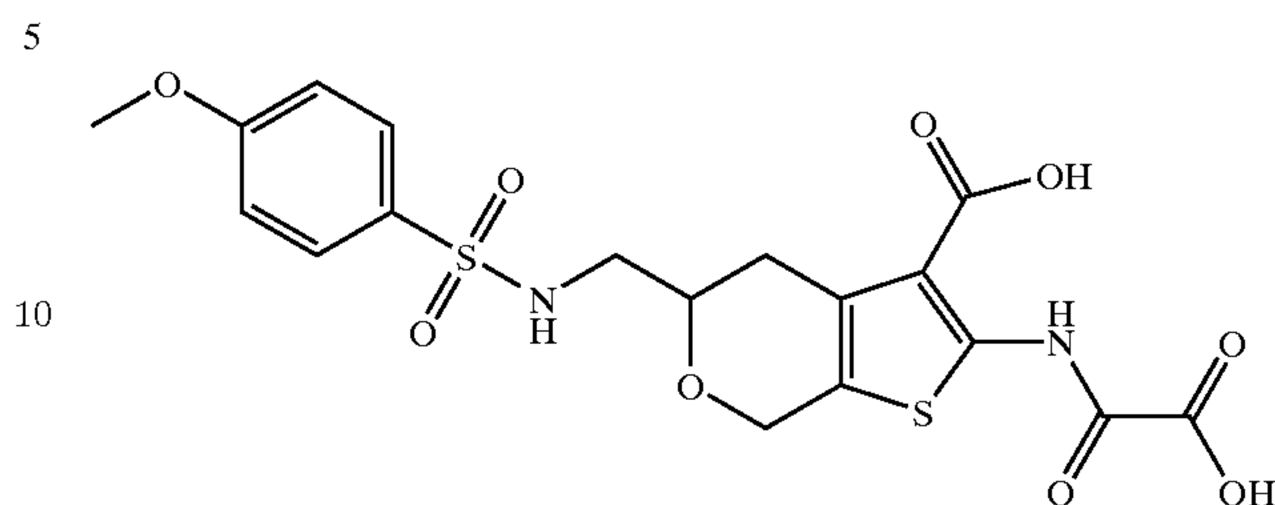
5-[(4-Methoxy-benzenesulfonylamino)-methyl]-2-(oxalyl-amino)-4,7-dihydro-5H-thieno[2,3-c]pyran-3-carboxylic Acid
