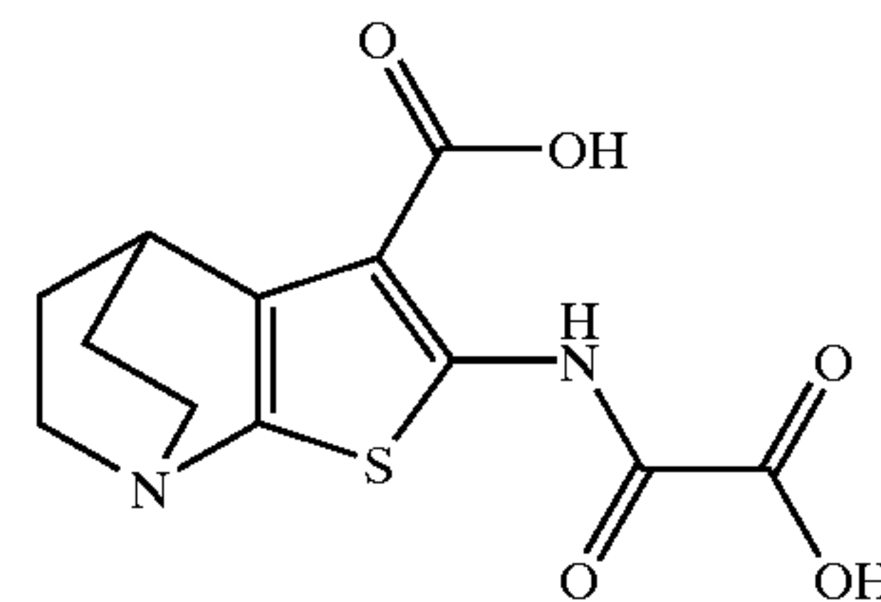
2-(Oxalyl-amino)-4,5,6,7-tetrahydro-4,7-ethano-thieno[2,3-b]pyridine-3-carboxylic Acid
