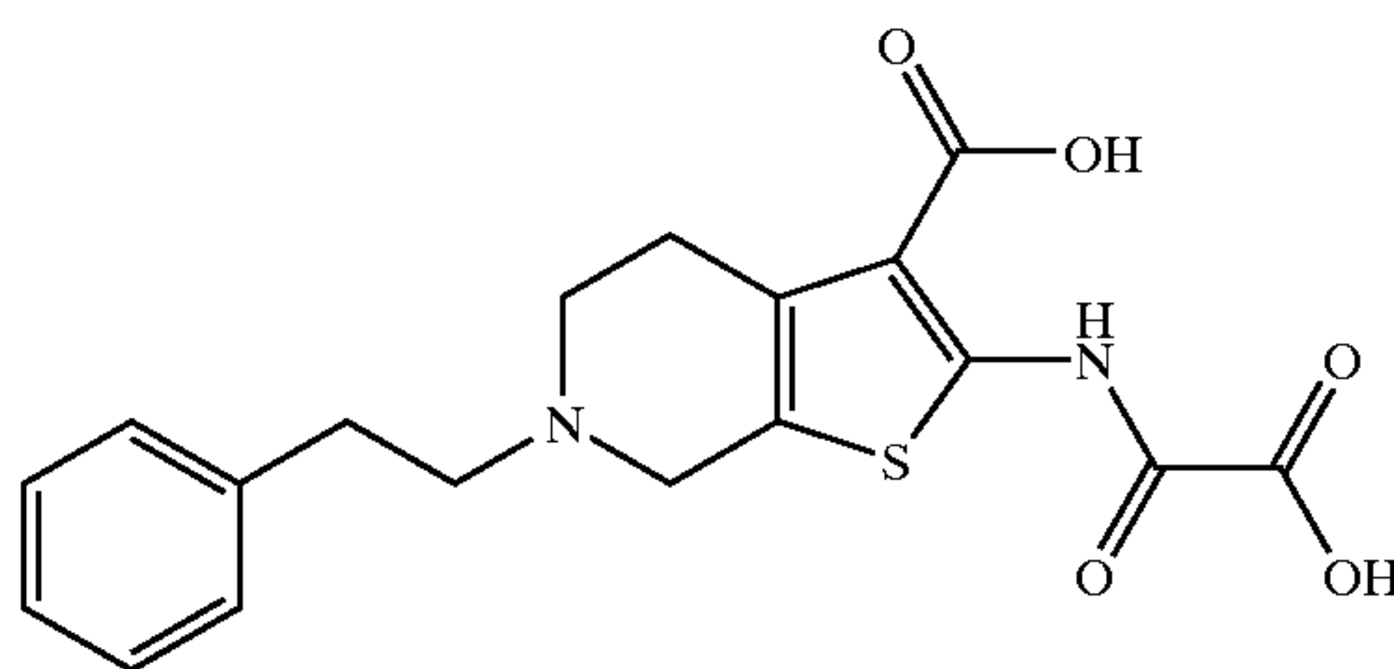
2-(Oxalyl-amino)-6-phenethyl-4,5,6,7-tetrahydro-thieno[2,3-c]pyridine-3-carboxylic Acid
