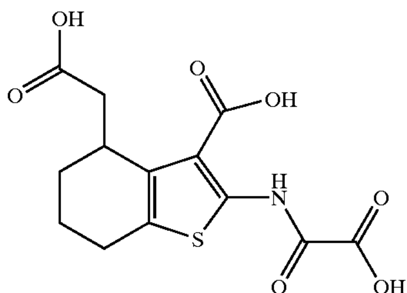
4-Carboxymethyl-2-(oxalyl-amino)-4,5,6,7-tetrahydro-benzo-[b]thiophene-3-carboxylic Acid
