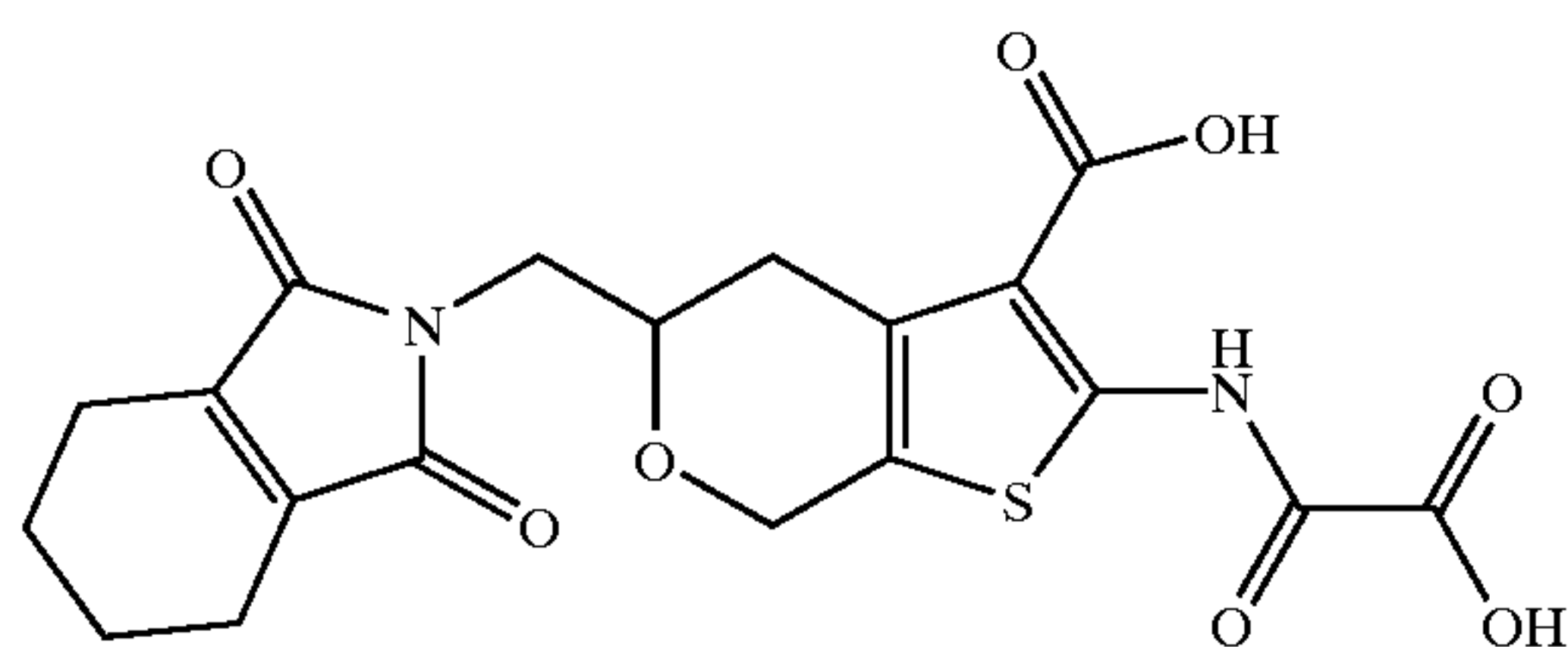
5-(1,3-Dioxo-1,3,4,5,6,7-hexahydro-isoindol-2-ylmethyl)-2-(oxalyl-amino)-4,7-dihydro-5H-thieno[2,3-c]pyran-3-carboxylic Acid
