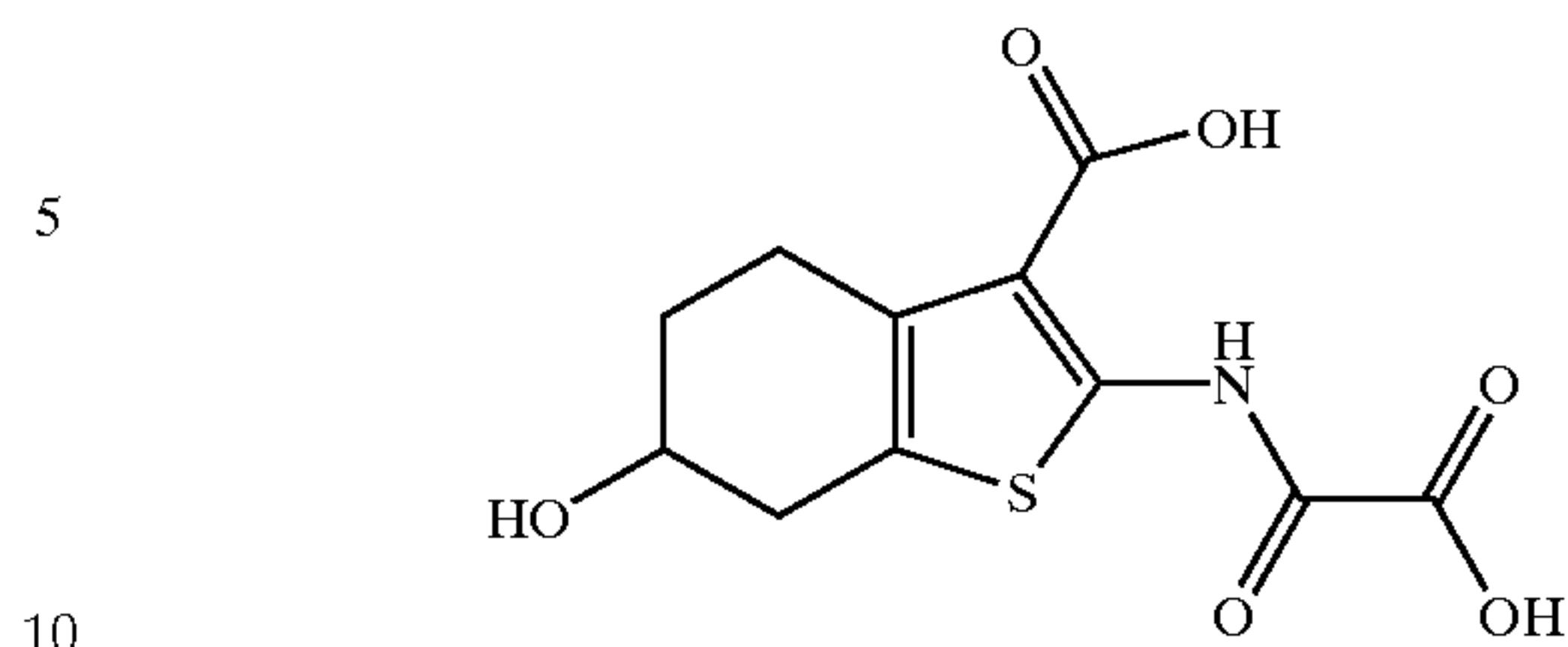
6-Hydroxy-2-(oxalyl-amino)-4,5,6,7-tetrahydro-benzo[b]thiophen-3-carboxylic Acid
