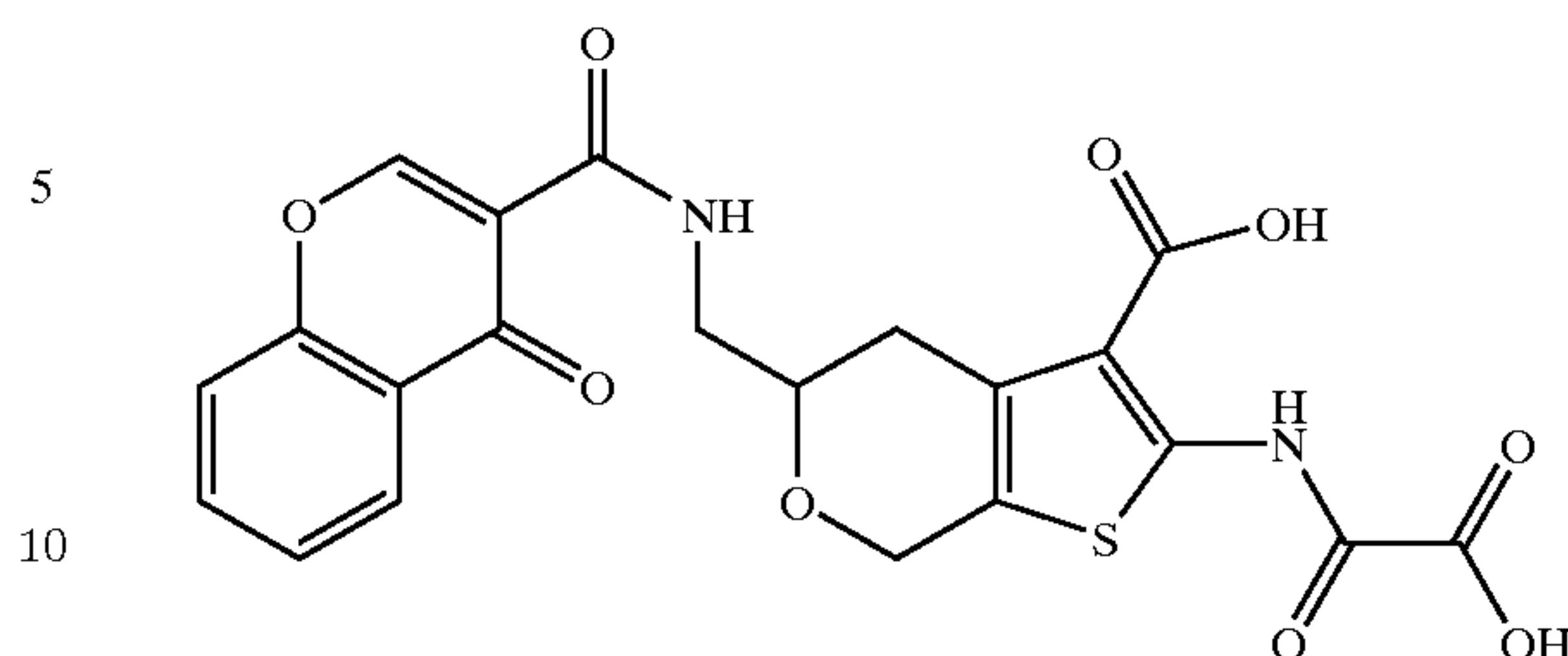
2-(Oxalyl-amino)-5-(((4-oxo-chromene-4H-3-carbonyl)amino)methyl)-4,7-dihydro-5H-thieno[2,3-c]pyran-3-carboxylic Acid
