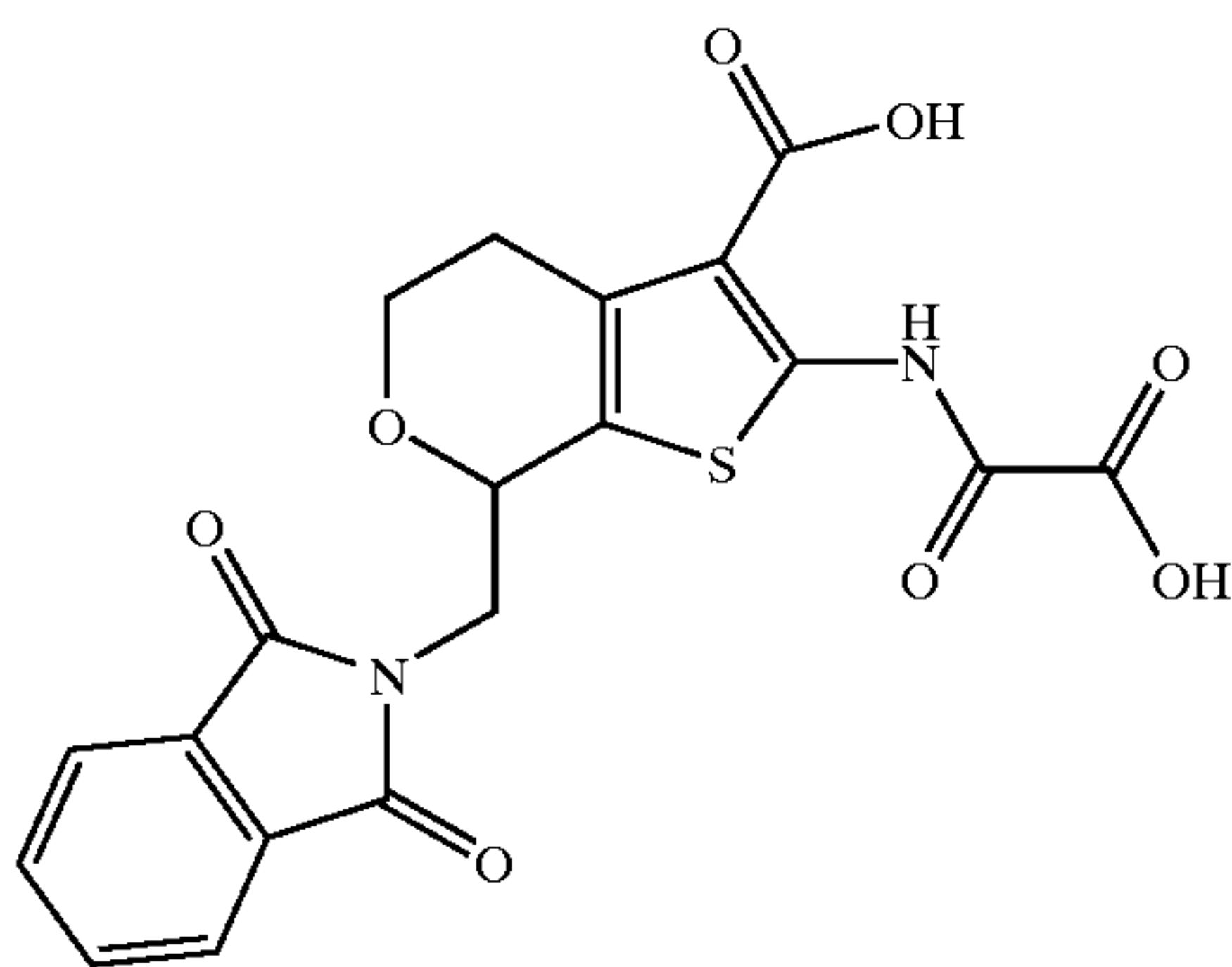
7-(1,3-Dioxo-1,3-dihydro-isoindol-2-ylmethyl)-2-(oxalyl-amino)-4,7-dihydro-5H-thieno[2,3-c]pyran-3-carboxylic Acid
