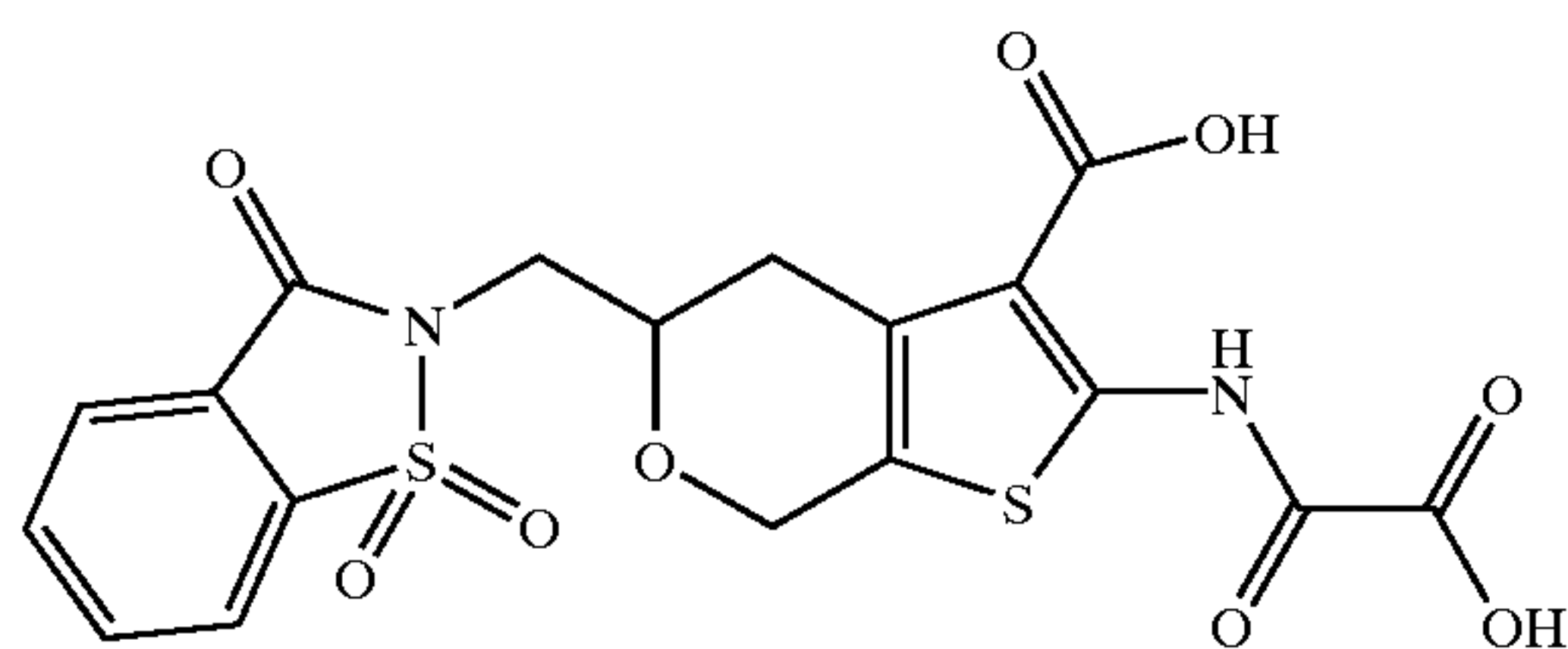
2-(Oxalyl-amino)-5-(1,1,3-trioxo-1,3-dihydro-1H-benzo[d]isothiazol-2-ylmethyl)-4,7-dihydro-5H-thieno[2,3-c]pyran-3-carboxylic Acid
