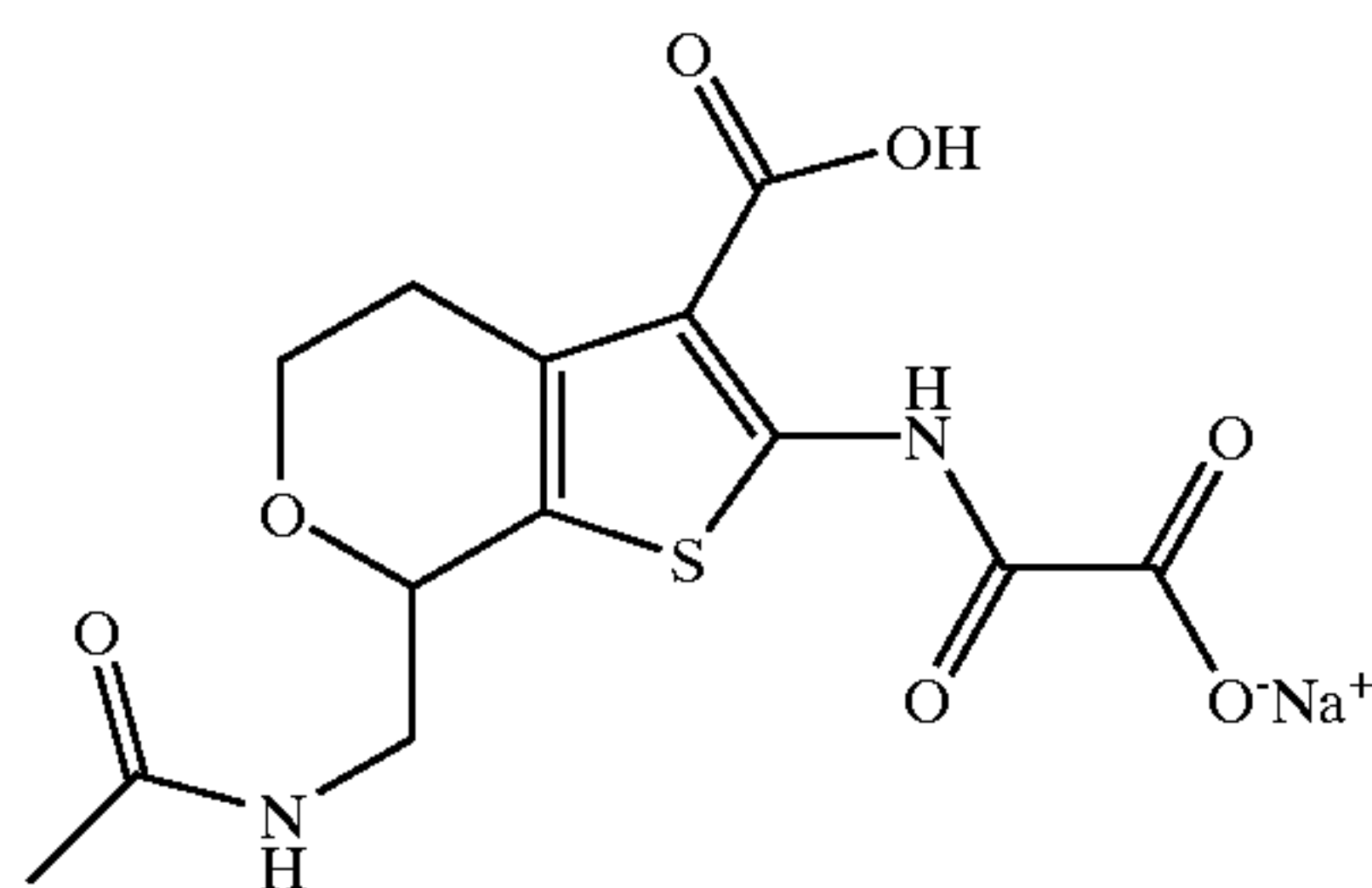
7-(Acetylamino-methyl)-2-(oxalyl-amino)-4,7-dihydro-5H-thieno[2,3-c]pyran-3-carboxylic Acid, Mono Sodium Salt
