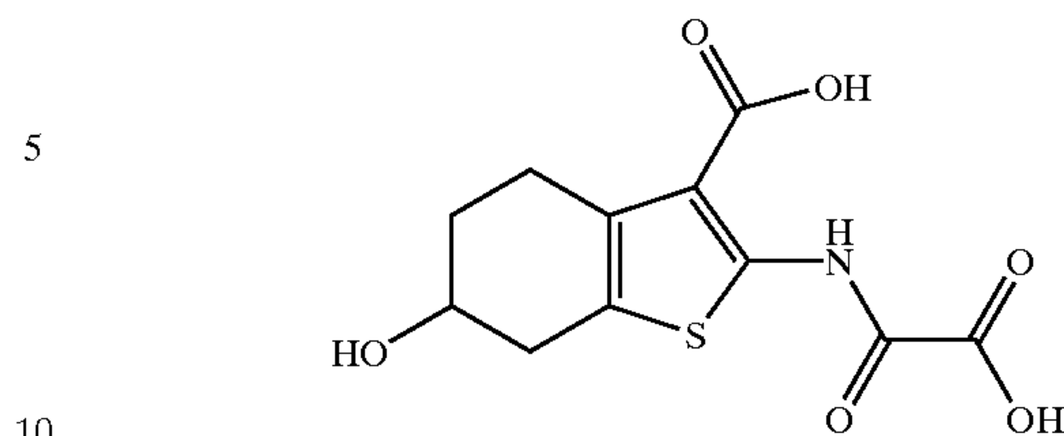
6-Hydroxy-2-(oxalyl-amino)-4,5,6,7-tetrahydro-benzo[b]thiophen-3-carboxylic Acid
