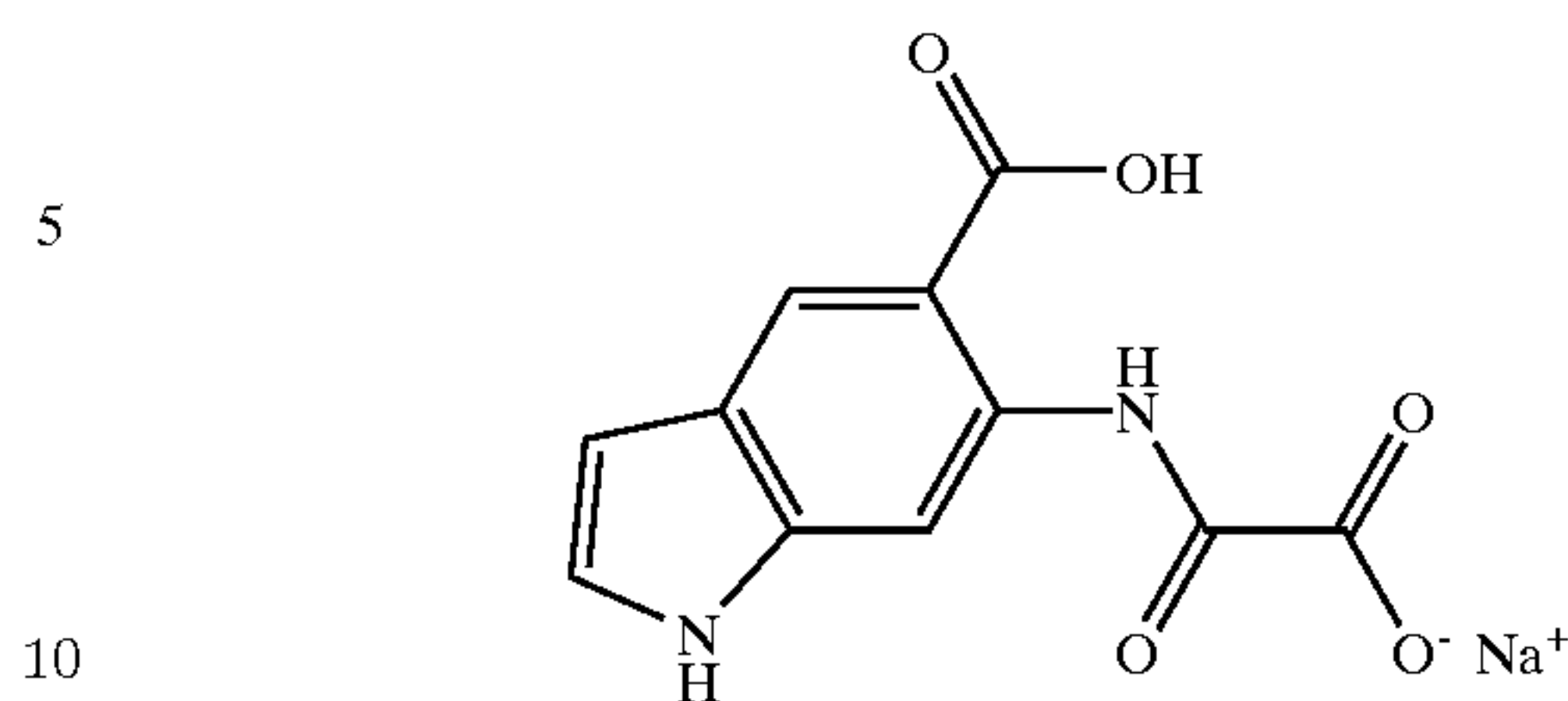
6-(Oxalyl-amino)-1H-indole-5-carboxylic Acid, Mono Sodium Salt
