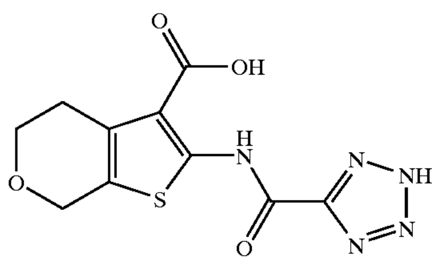
2-((2-H-Tetrazol-5-carbonyl)amino)-4,7-dihydro-5H-thieno[2,3-c]pyran-3-carboxylic Acid
