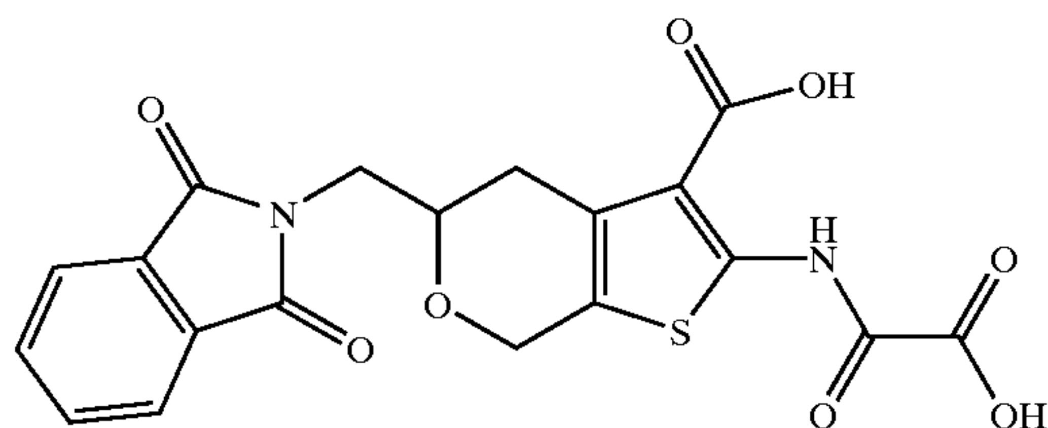
5-(1,3-Dioxo-1,3-dihydro-isoindol-2-ylmethyl)-2-(oxalyl-amino)-4,7-dihydro-5H-thieno[2,3-c]pyran-3-carboxylic Acid
