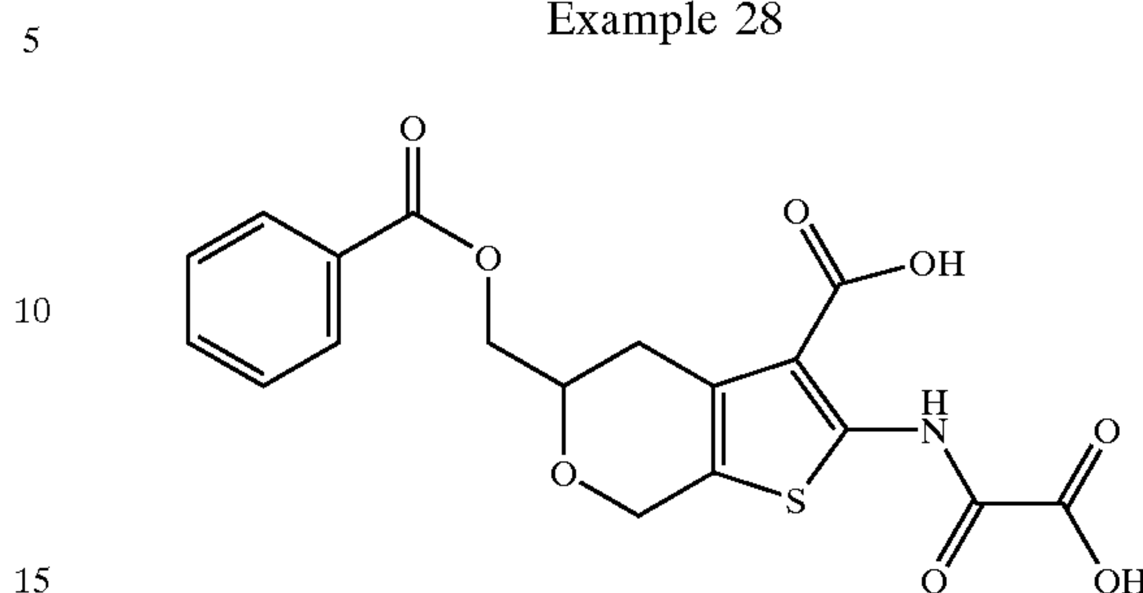
5-Benzoyloxymethyl-2-(oxalyl-amino)-4,7-dihydro-5H-thieno[2,3-c]pyran-3-carboxylic Acid
