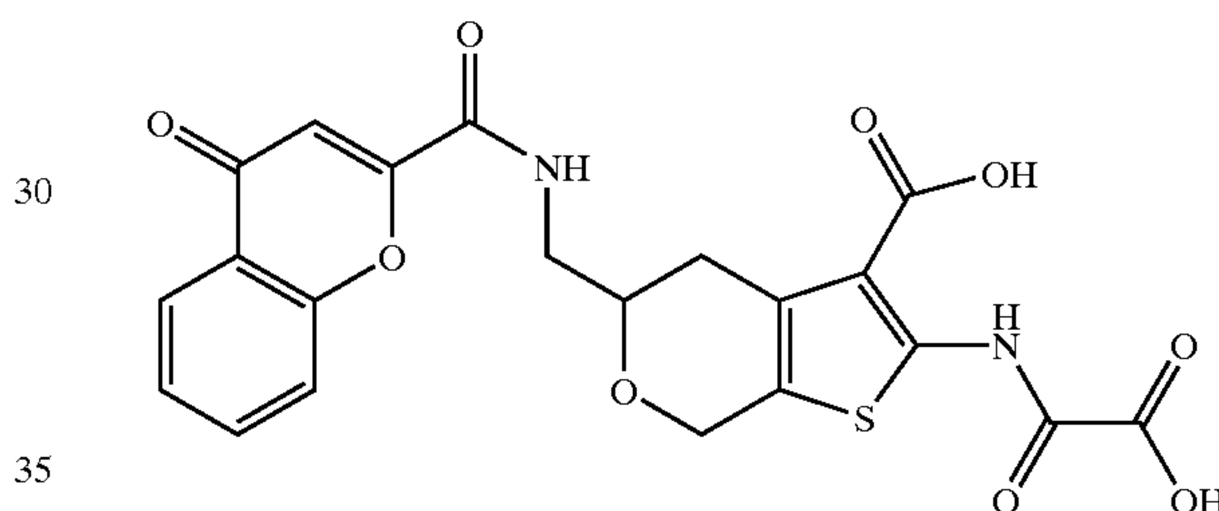
2-(Oxalyl-amino)-5-(((4-oxo-chromene-4H-2-carbonyl)amino)methyl)-4,7-dihydro-5H-thieno[2,3-c]pyran-3-carboxylic Acid
