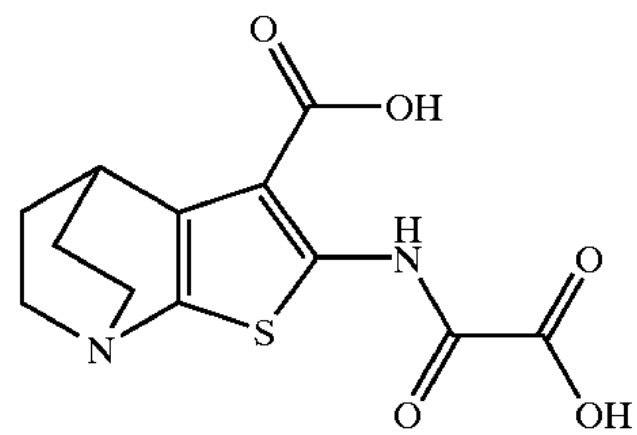
2-(Oxalyl-amino)-4,5,6,7-tetrahydro-4,7-ethano-thieno[2,3-b]pyridine-3-carboxylic Acid
