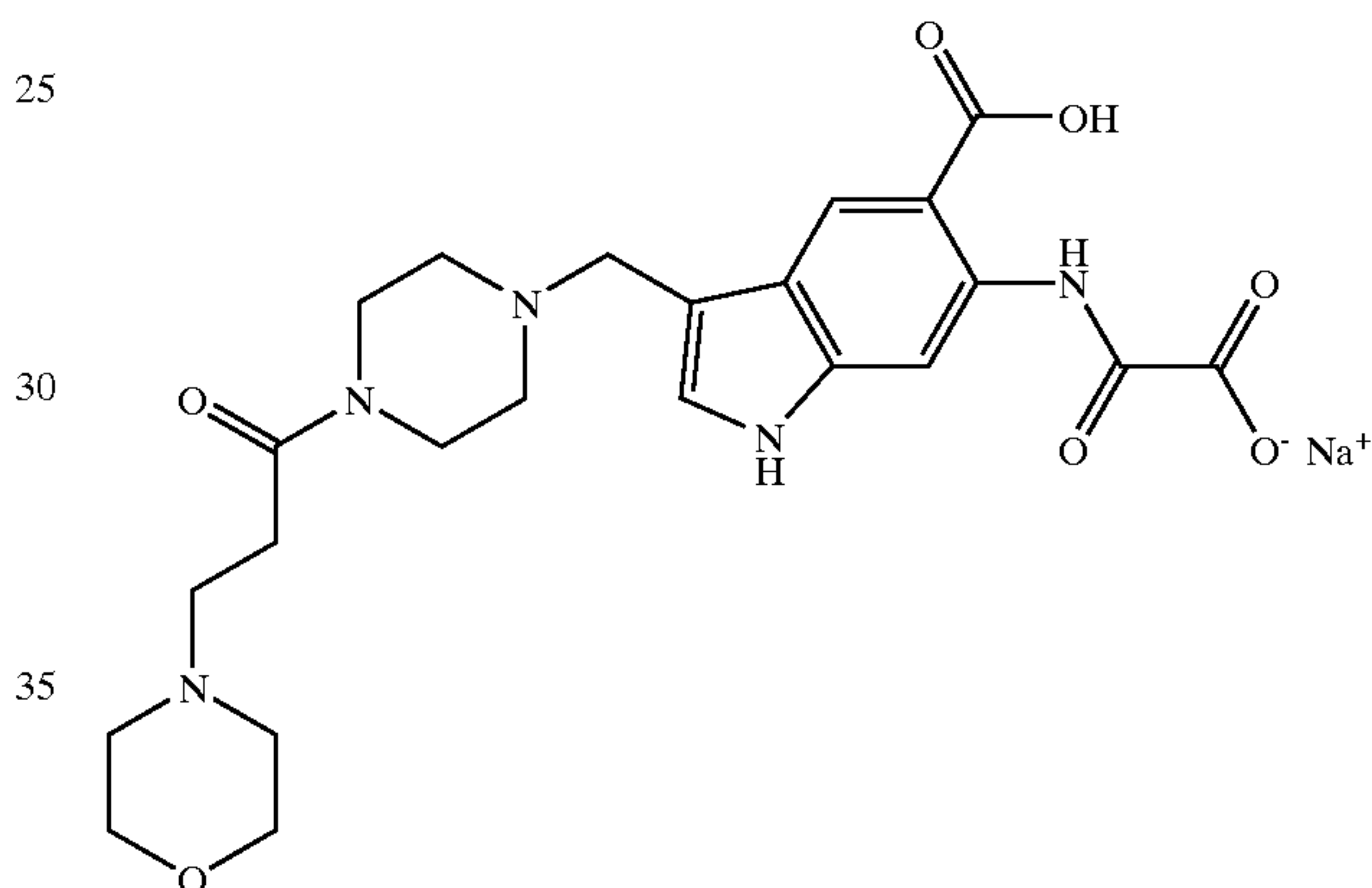
3-[4-(3-Morpholin-4-yl-propionyl)-piperazin-1-ylmethyl]-6-(oxalyl-amino)-1H-indole-5-carboxylic Acid, Mono Sodium Salt
