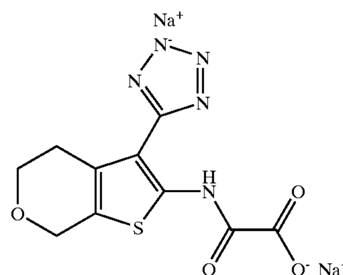
N-(3-(2H-Tetrazol-5-yl)-4,7-dihydro-5H-thieno[2,3-c]pyran-2-yl)oxalamic Acid, Di Sodium Salt
