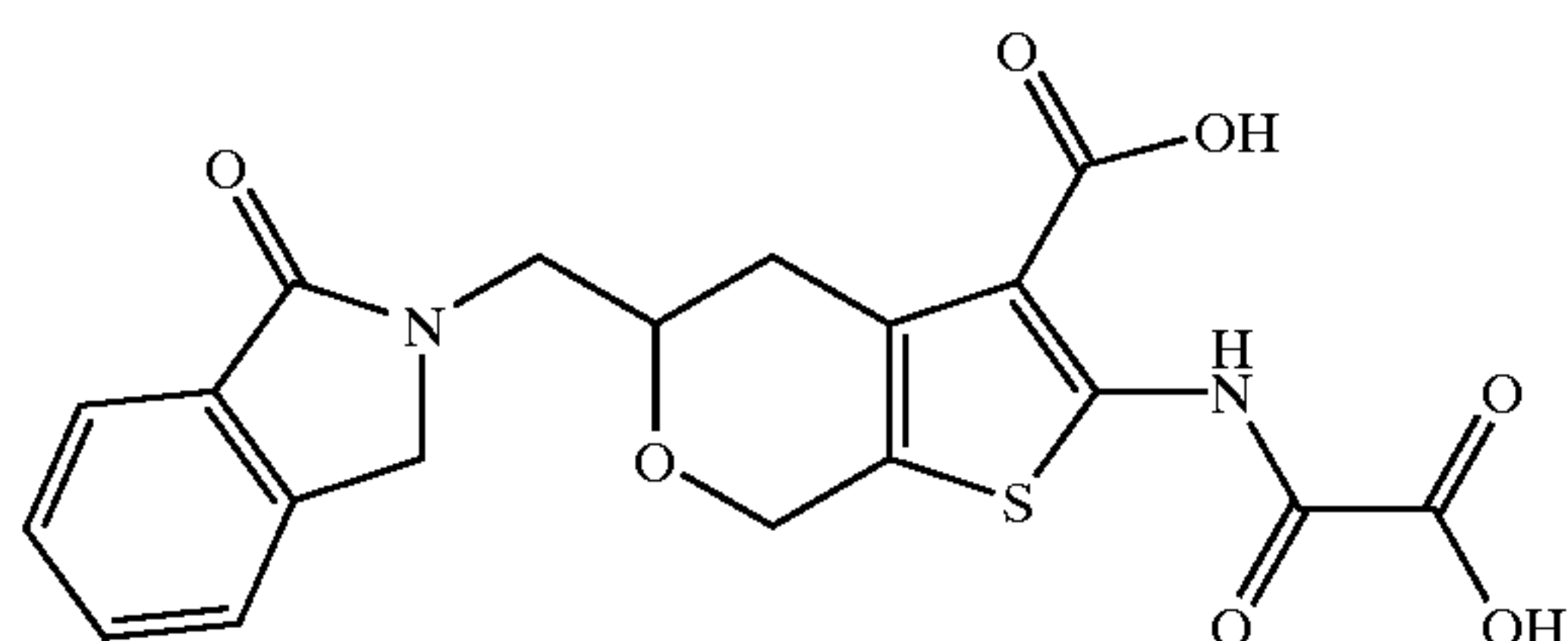
2-(Oxalyl-amino)-5-(1-oxo-1,3-dihydro-isoindol-2-ylmethyl)-4,7-dihydro-5H-thieno[2,3-c]pyran-3-carboxylic Acid
