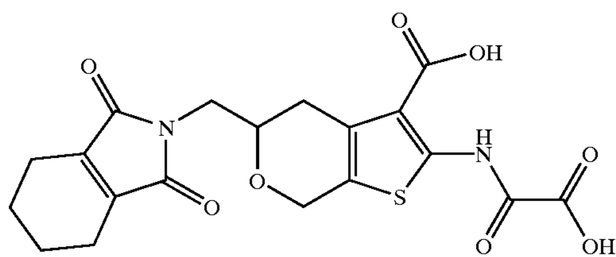
5-(1,3-Dioxo-1,3,4,5,6,7-hexahydro-isoindol-2-ylmethyl)-2-(oxalyl-amino)-4,7-dihydro-5H-thieno[2,3-c]pyran-3-carboxylic Acid
