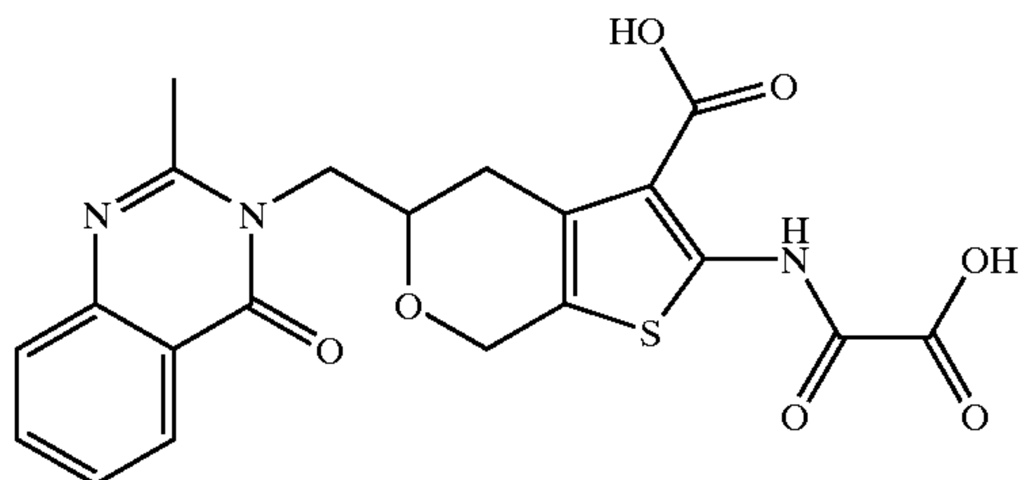
5-(2-Methyl-4-oxo-4H-quinazolin-3-ylmethyl)-2-(oxalyl-amino)-4,7-dihydro-5H-thieno[2,3-c]pyran-3-carboxylic Acid
