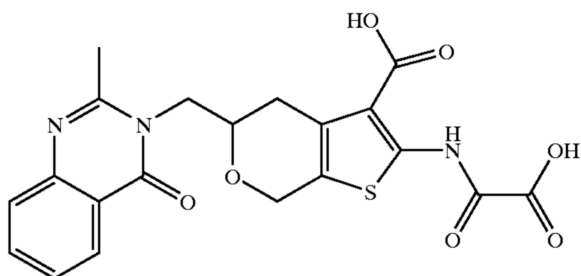
5-(2-Methyl-4-oxo-4H-quinazolin-3-ylmethyl)-2-(oxalyl-amino)-4,7-dihydro-5H-thieno[2,3-c]pyran-3-carboxylic Acid
