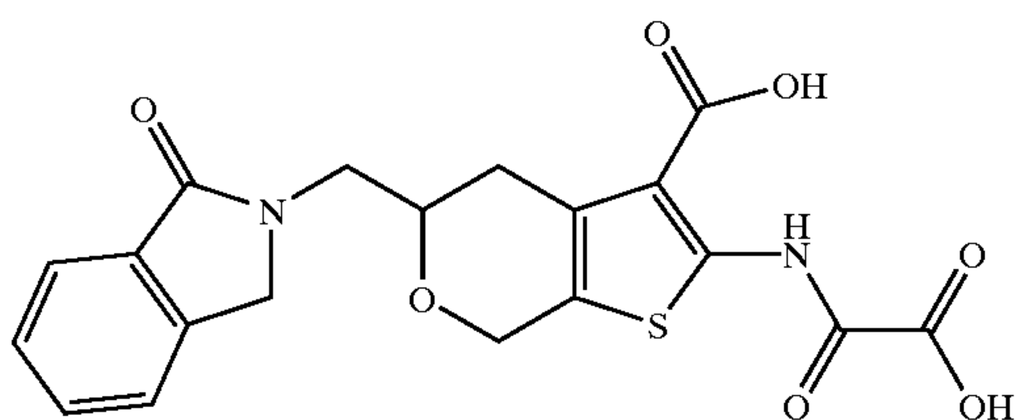
2-(Oxalyl-amino)-5-(1-oxo-1,3-dihydro-isoindol-2-ylmethyl)-4,7-dihydro-5H-thieno[2,3-c]pyran-3-carboxylic Acid
