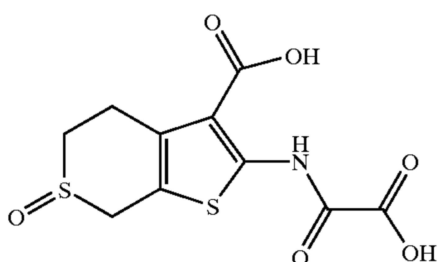
2-(Oxalyl-amino)-6-oxo-4,7-dihydro-5H-thieno[2,3-c]thiopyran-3-carboxylic Acid
