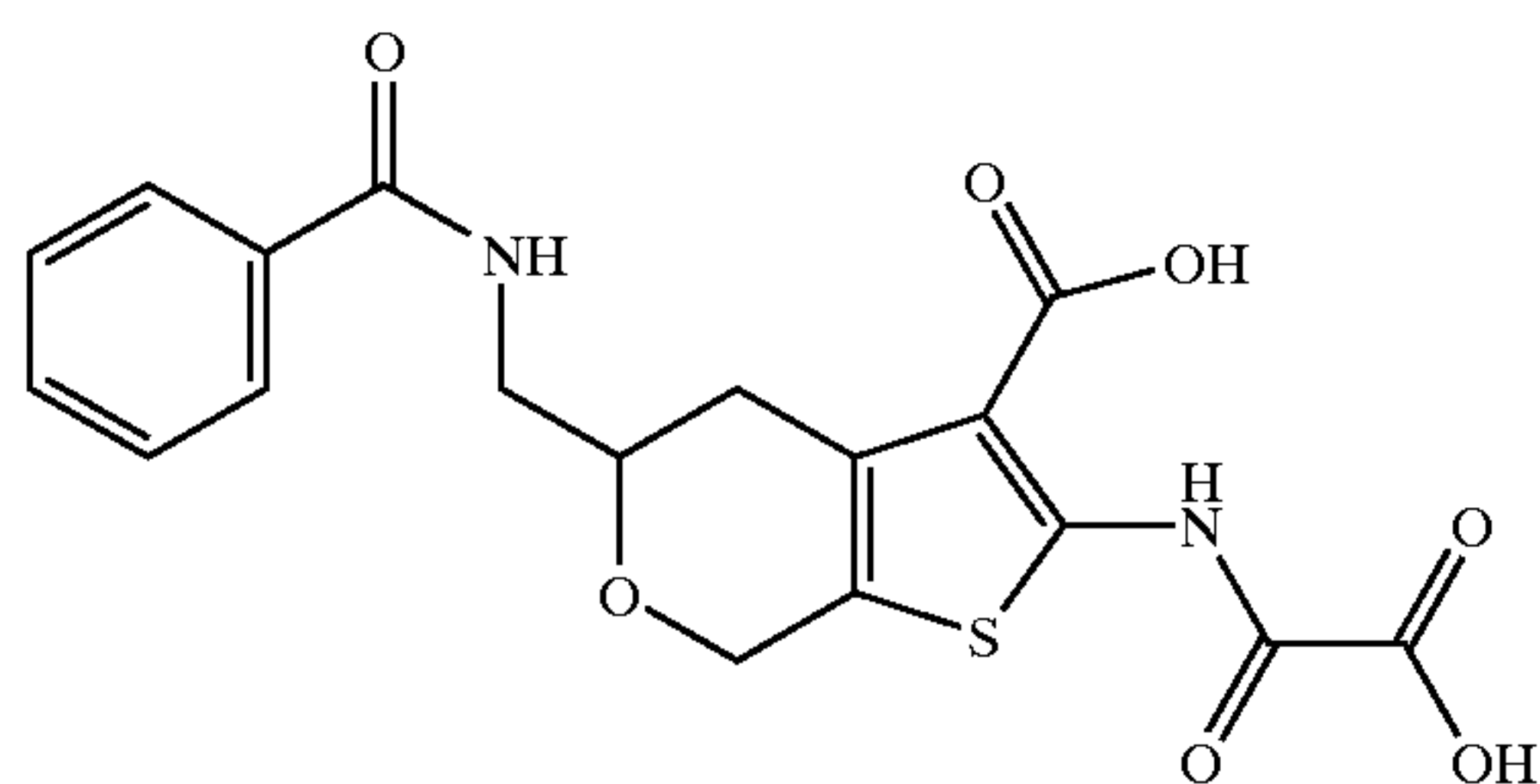
5-(Benzolamino-methyl)-2-(oxalyl-amino)-4,7-dihydro-5H-thieno[2,3-c]pyran-3-carboxylic Acid
