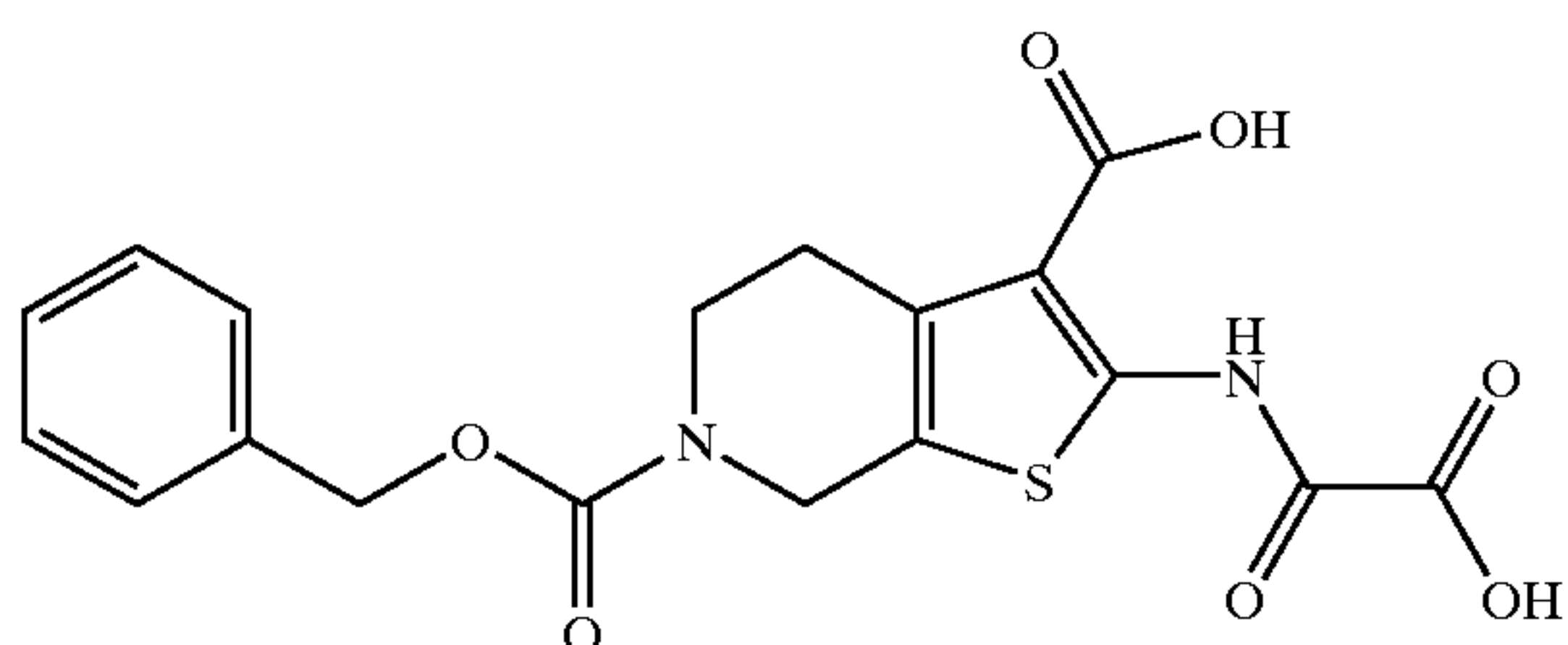
2-(Oxalyl-amino)-4,7-dihydro-5H-thieno[2,3-c]pyridine-3,6-dicarboxylic Acid 6-Benzyl Ester
