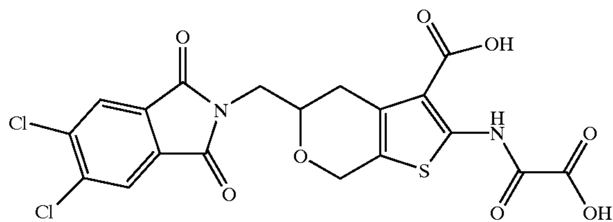
5-(5,6-Dichloro-1,3-dioxo-1,3-dihydro-isoindol-2-ylmethyl)-2-(oxalyl-amino)-4,7-dihydro-5H-thieno[2,3-c]pyran-3-carboxylic Acid
