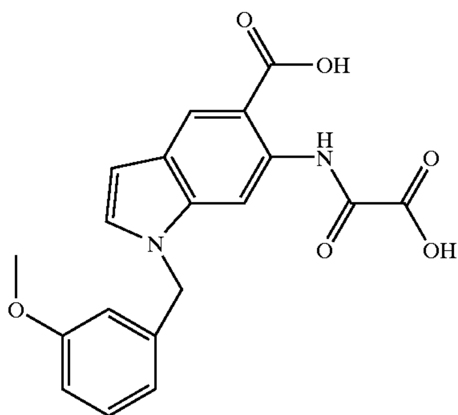
1-(3-Methoxy-benzyl)-6-(oxalyl-amino)-1H-indole-5-carboxylic Acid
