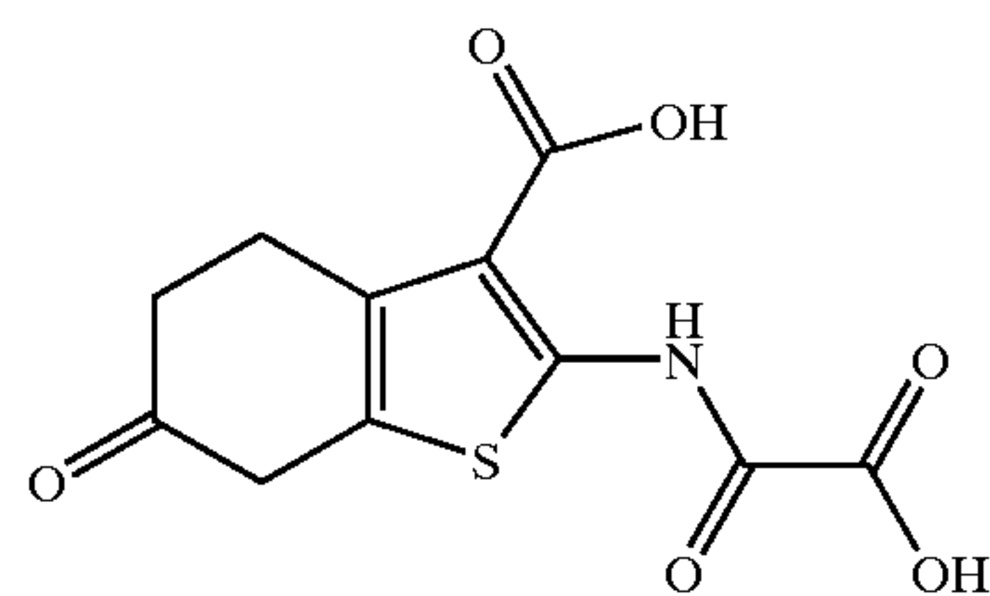
2-(Oxalyl-amino)-6-oxo-4,5,6,7-tetrahydro-benzo[b]thiophene-3-carboxylic Acid
