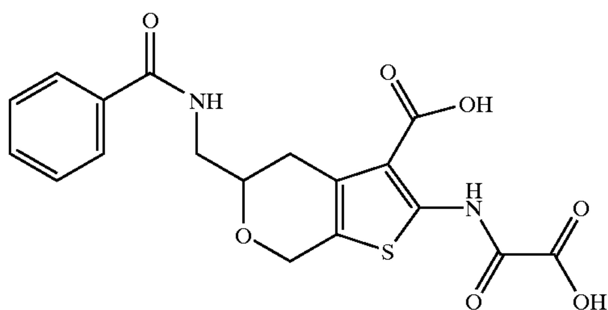
5-(Benzolamino-methyl)-2-(oxalyl-amino)-4,7-dihydro-5H-thieno[2,3-c]pyran-3-carboxylic Acid
