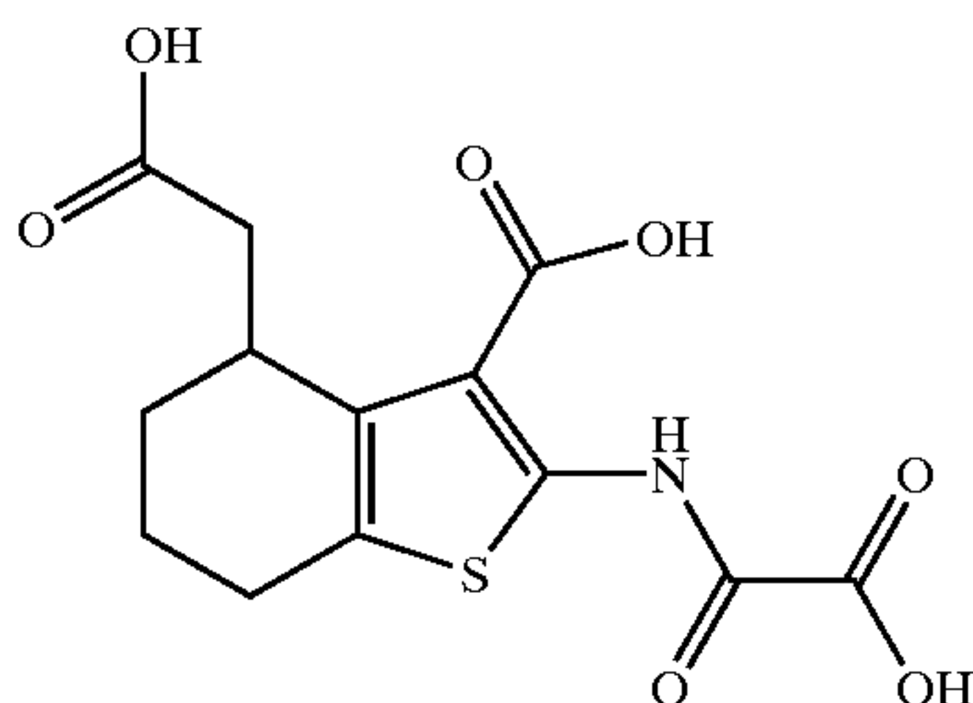
4-Carboxymethyl-2-(oxalyl-amino)-4,5,6,7-tetrahydro-benzo-[b]thiophene-3-carboxylic Acid
