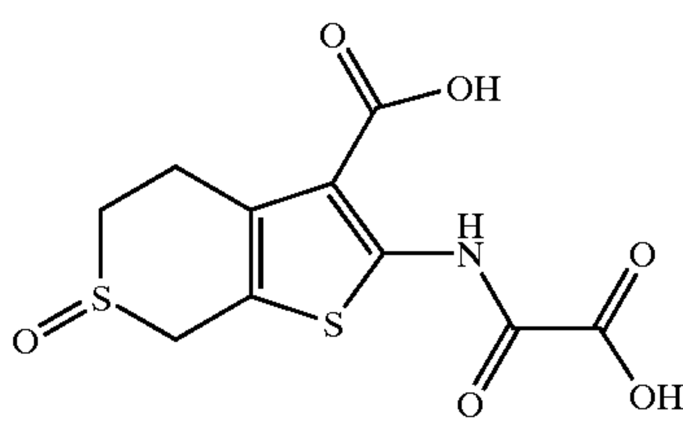
2-(Oxalyl-amino)-6-oxo-4,7-dihydro-5H-thieno[2,3-c]thiopyran-3-carboxylic Acid
