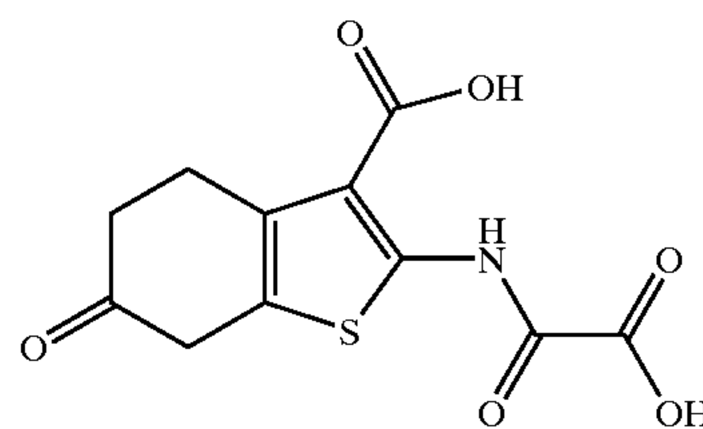
2-(Oxalyl-amino)-6-oxo-4,5,6,7-tetrahydro-benzo[b]thiophene-3-carboxylic Acid
