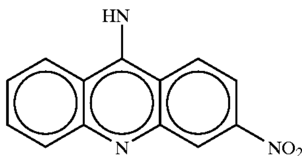
Ring C
