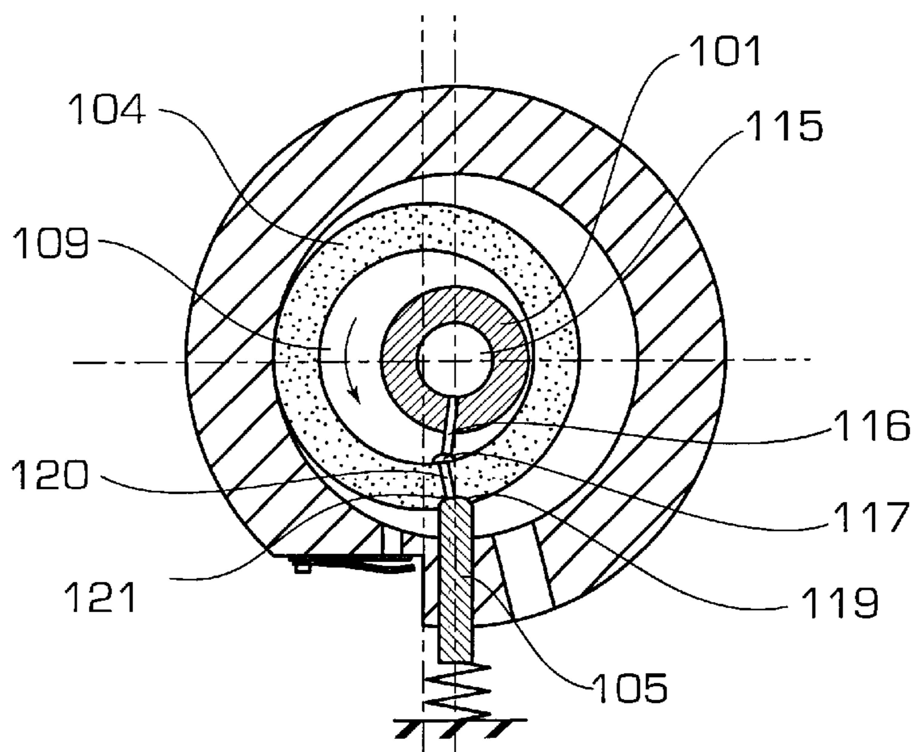
FIG. 7 PRIOR ART
