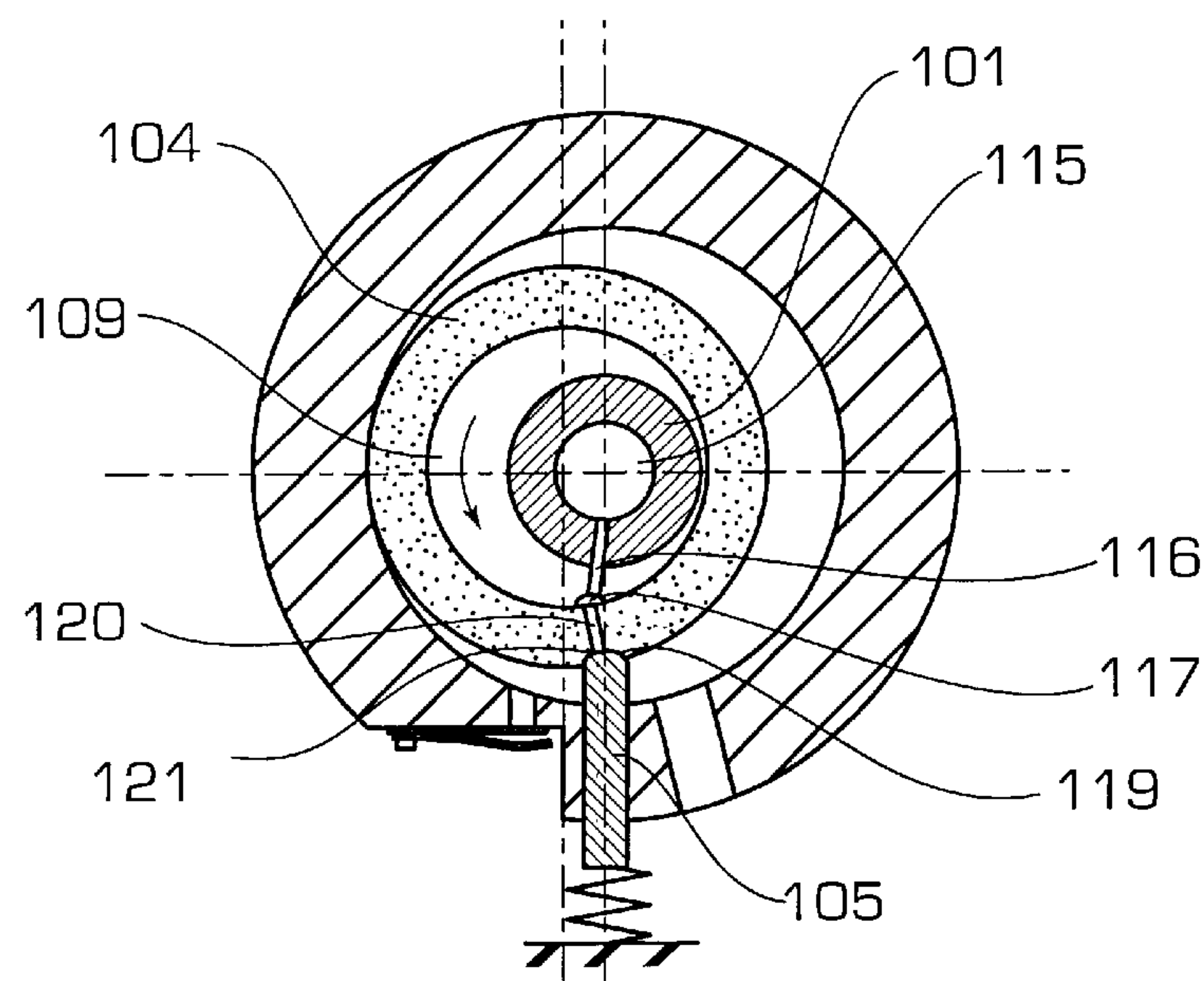
FIG. 7 PRIOR ART
