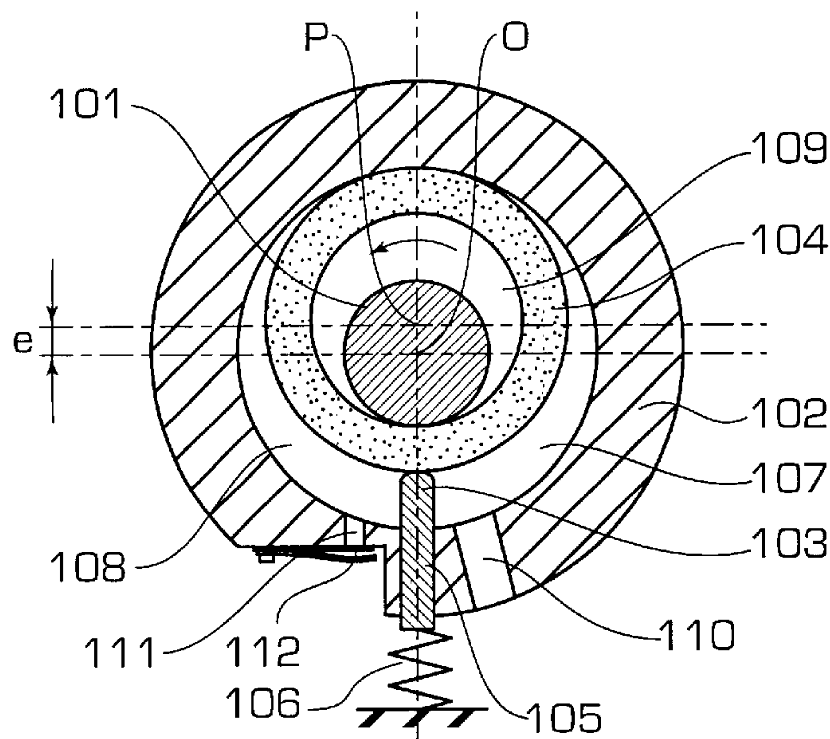
FIG. 6 PRIOR ART
