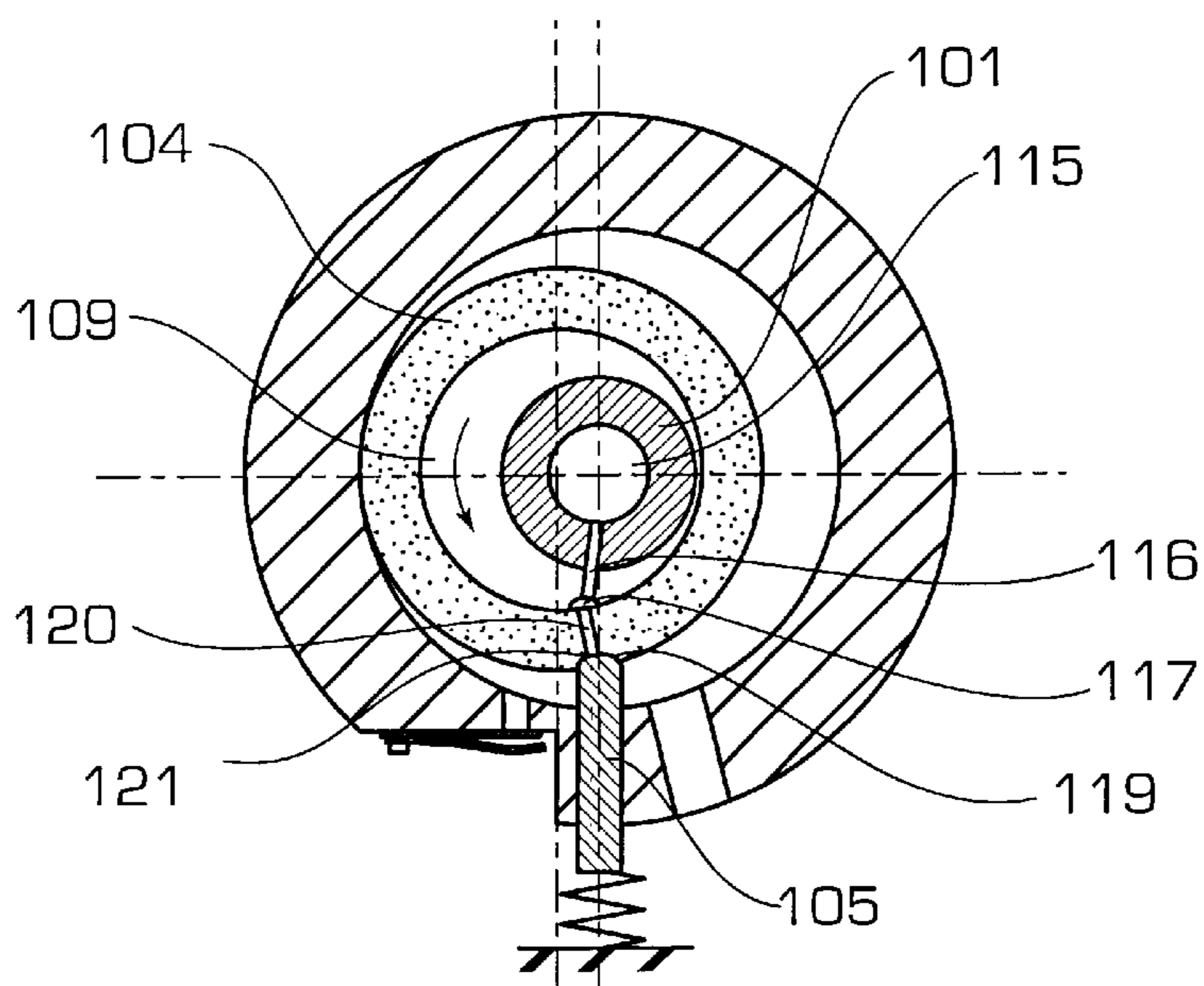
FIG. 7 PRIOR ART
