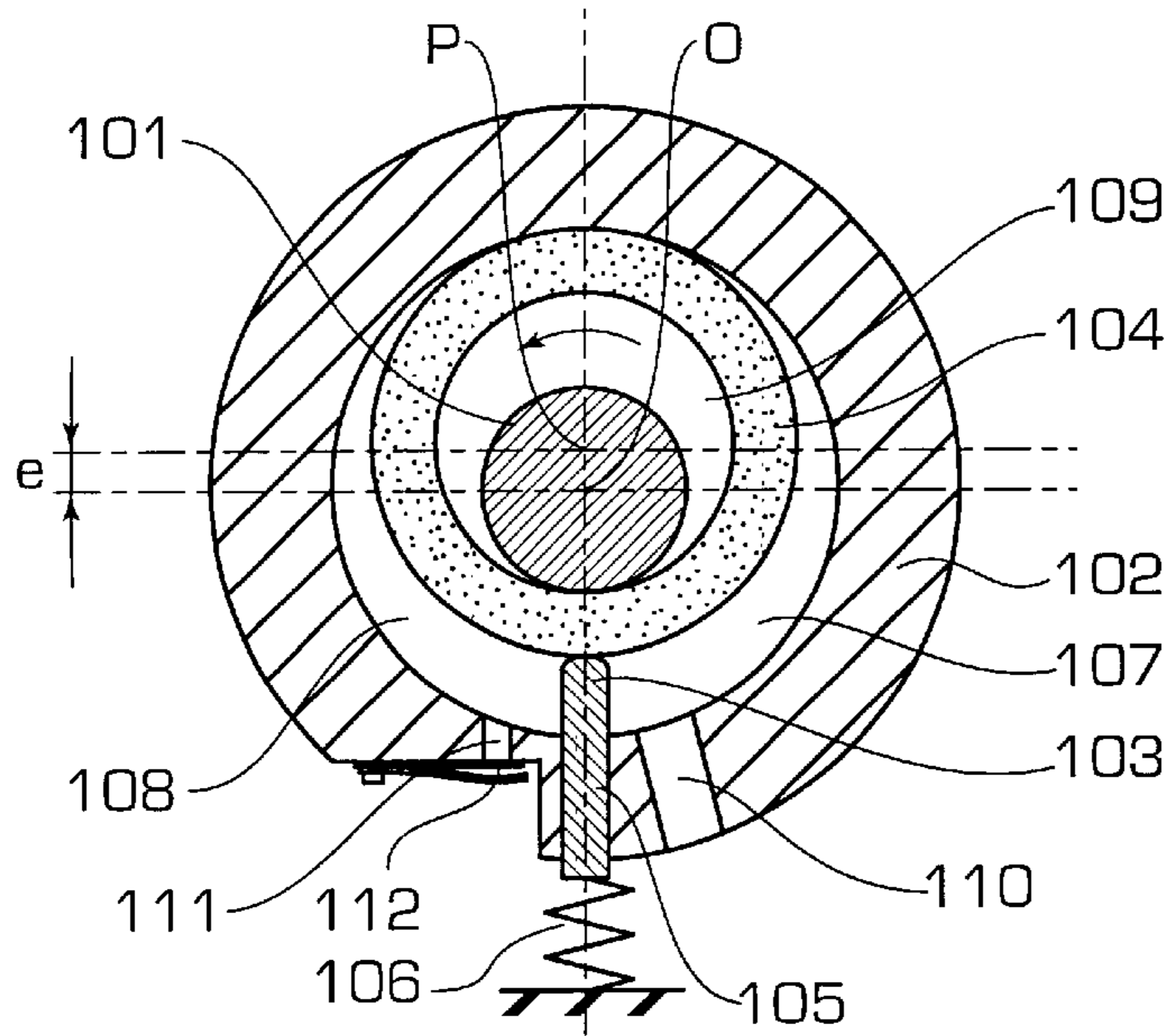
FIG. 6 PRIOR ART
