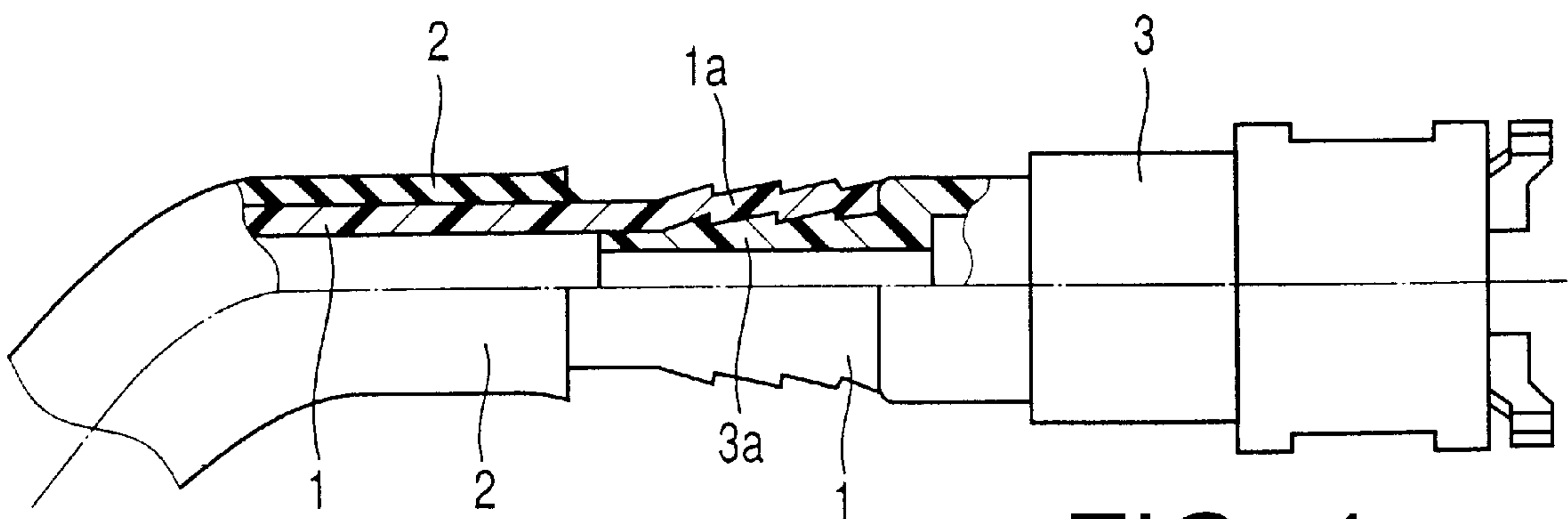
FIG. 4 PRIOR ART
