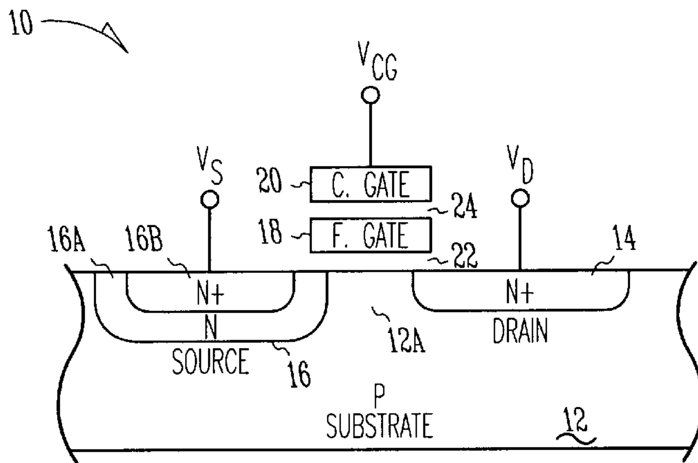
Fig. 1 (PRIOR ART)
