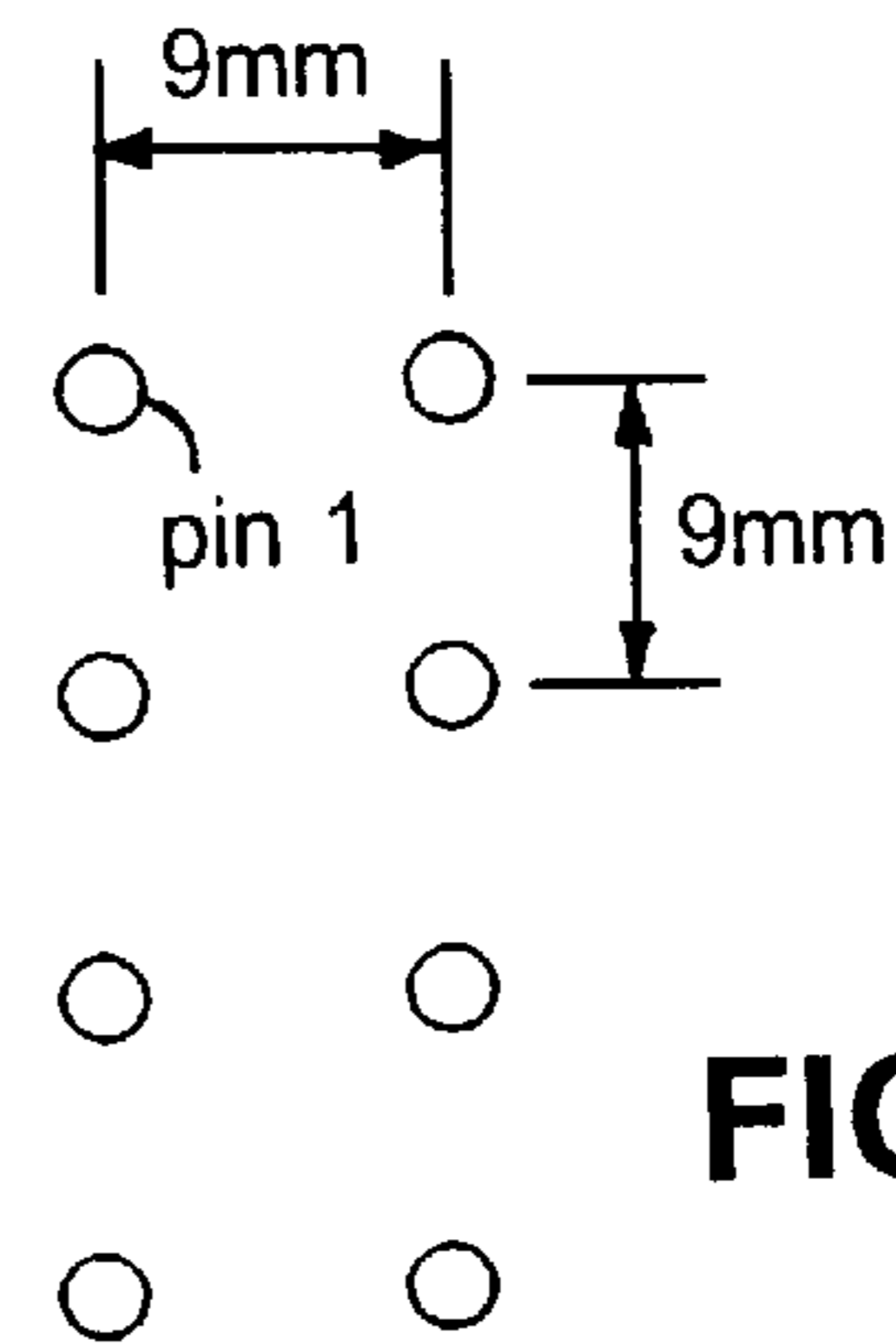
PIN LOCATION
