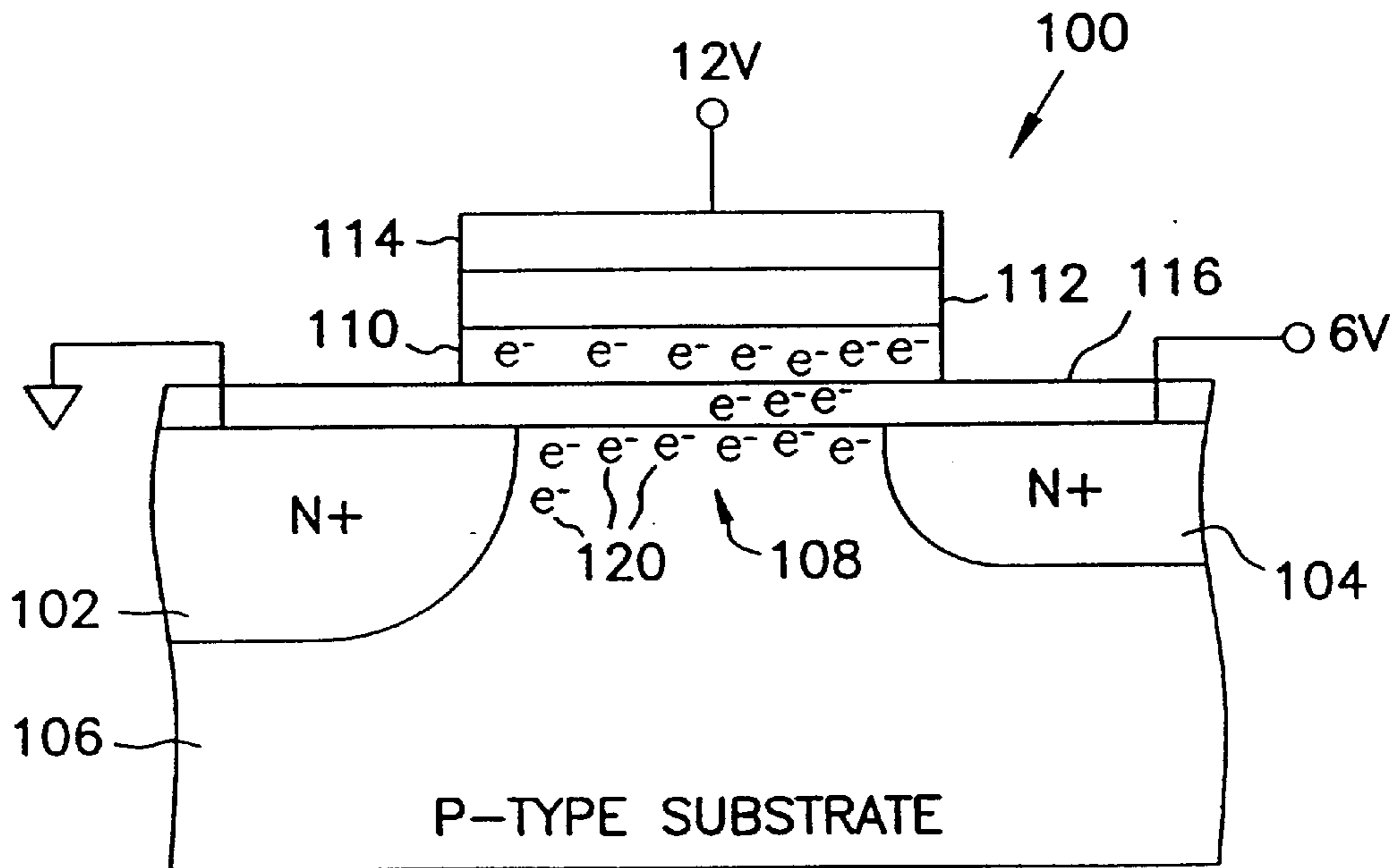
FIG. 2 (PRIOR ART)
