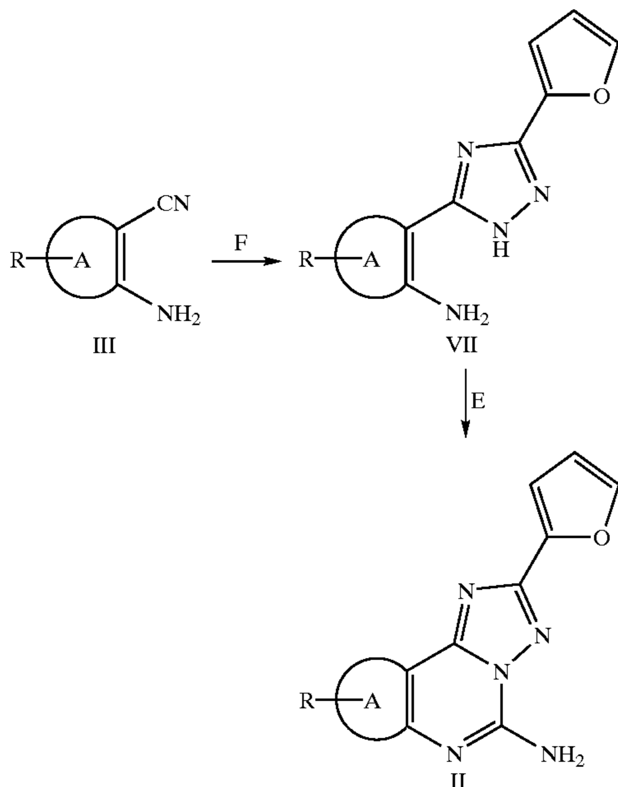
Scheme II
