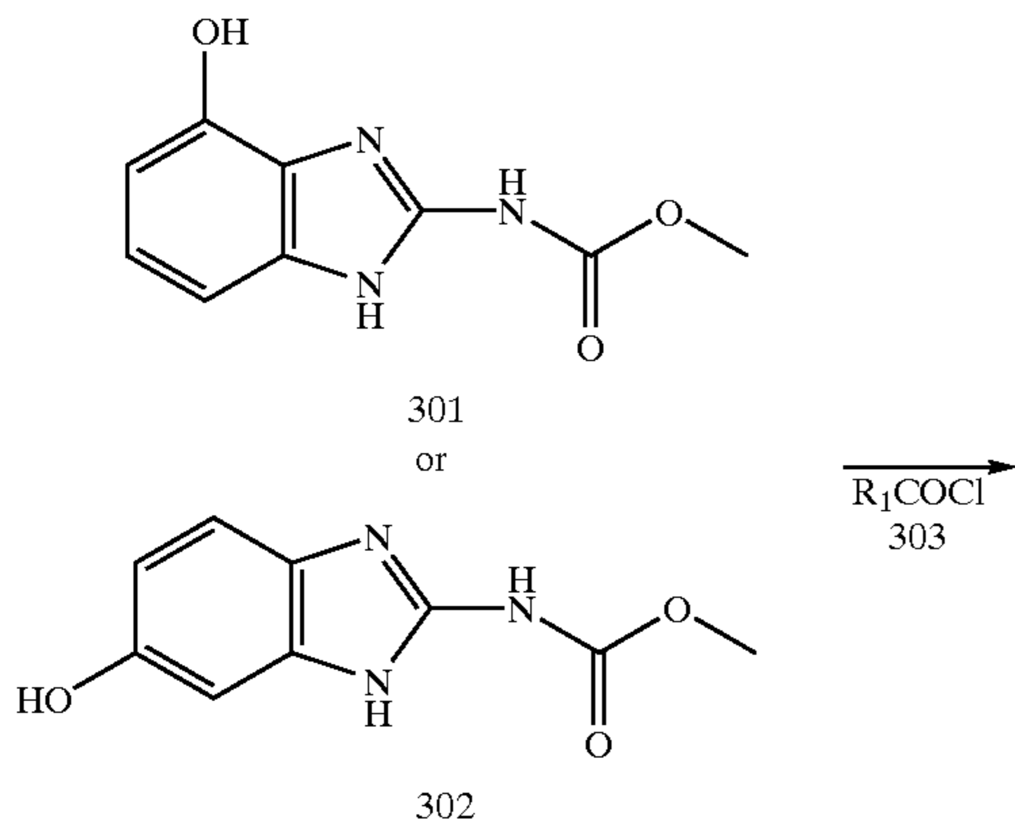
Reaction Scheme 3
