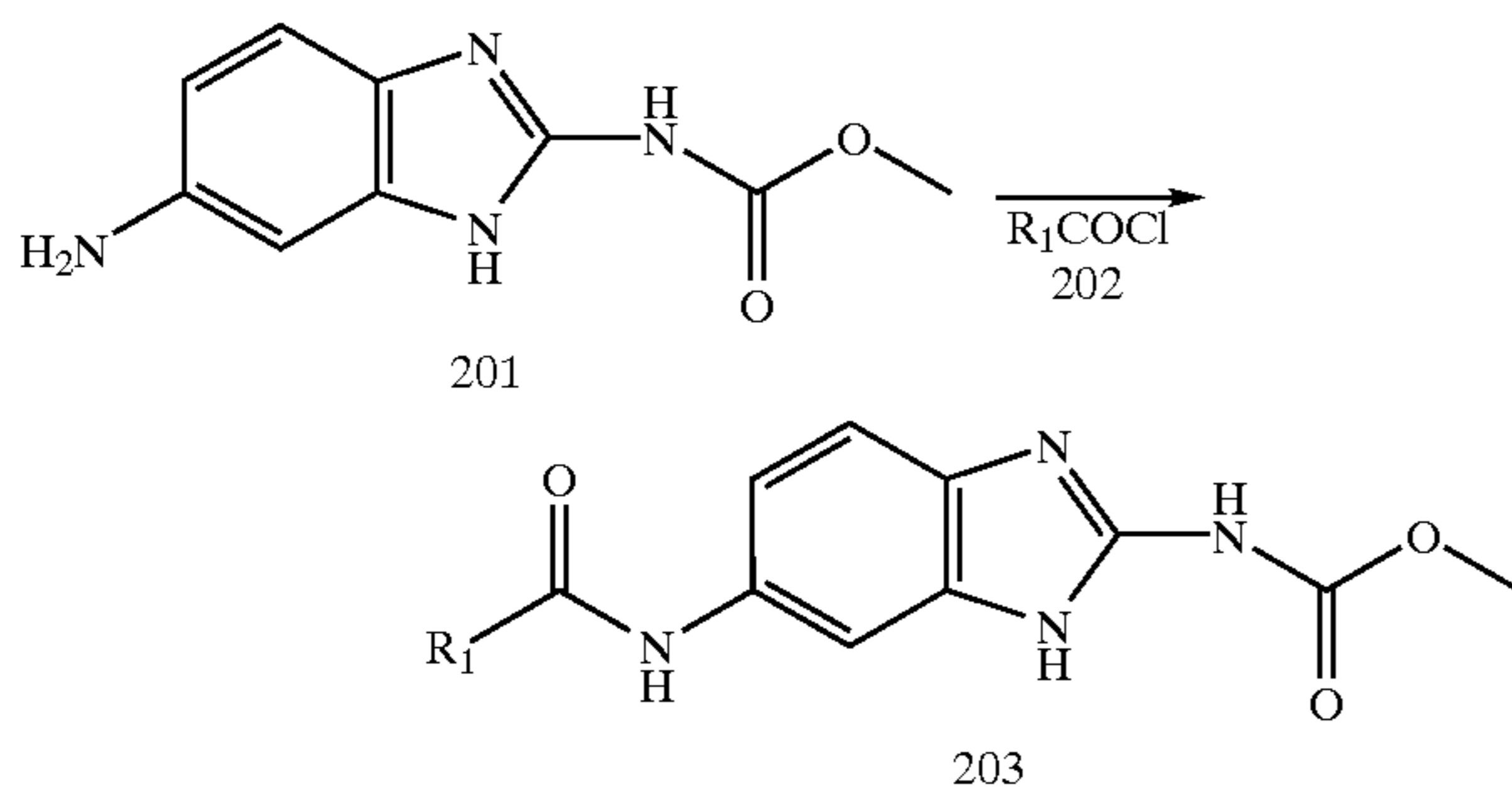
Reaction Scheme 2
