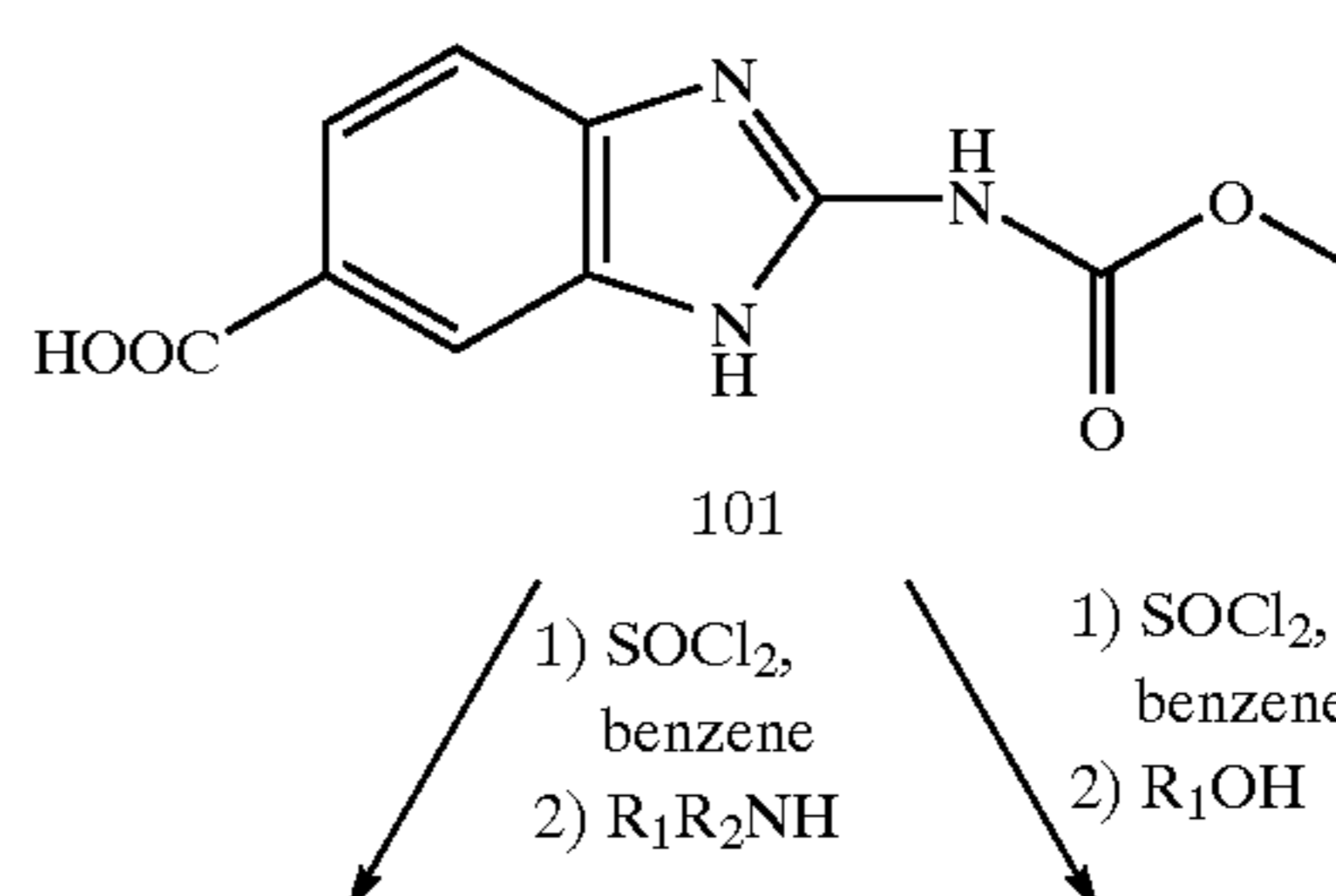
Reaction Scheme 1
