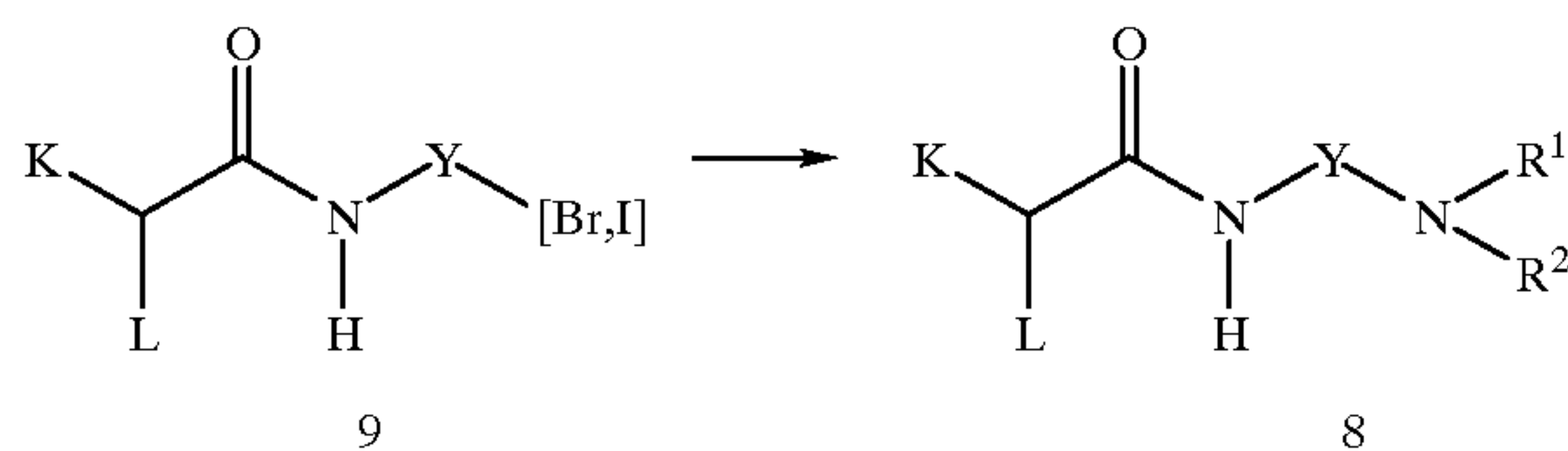
Scheme 4
