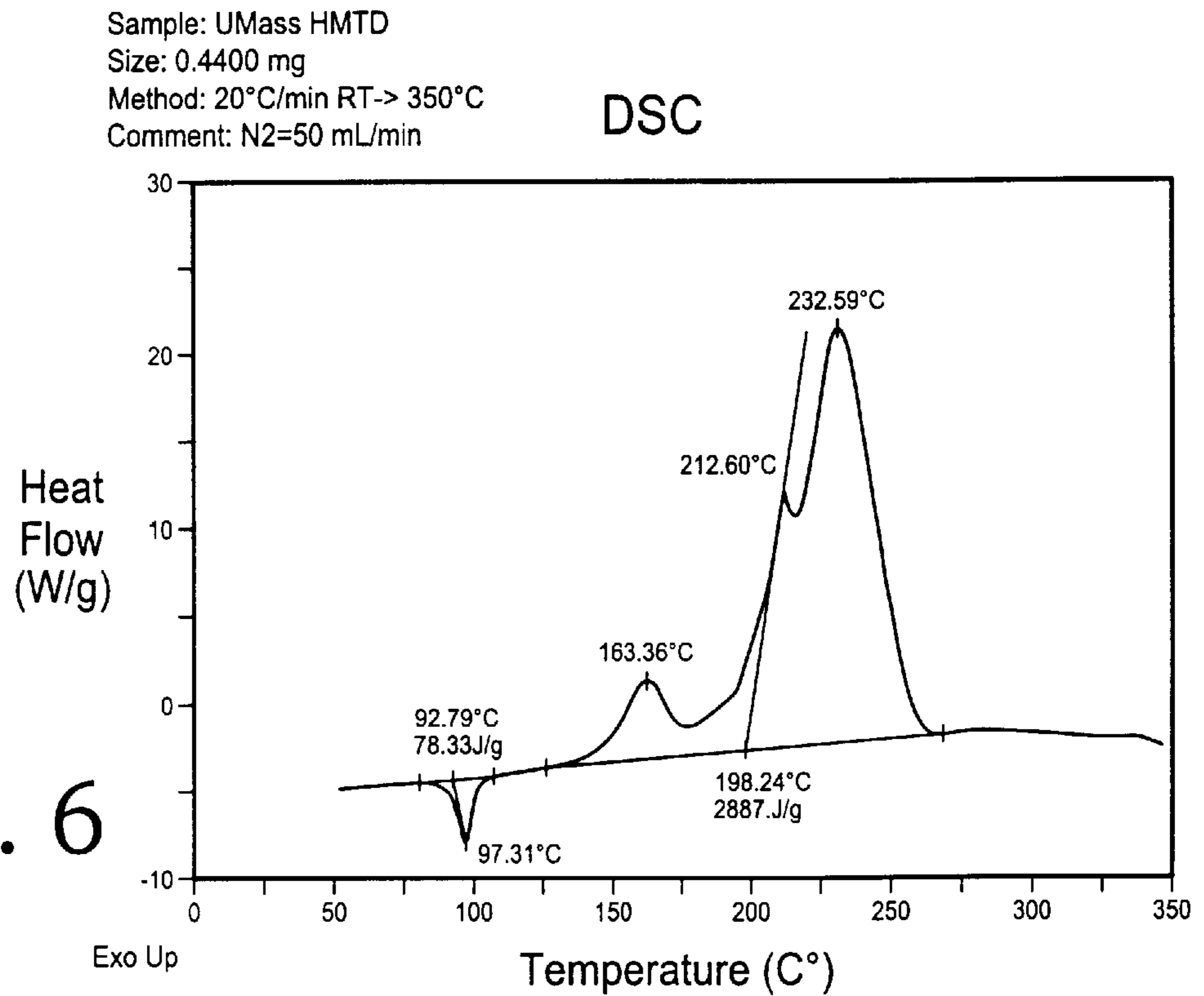
DSC thermogram of HMTD, sample weight is 0.44 mg
