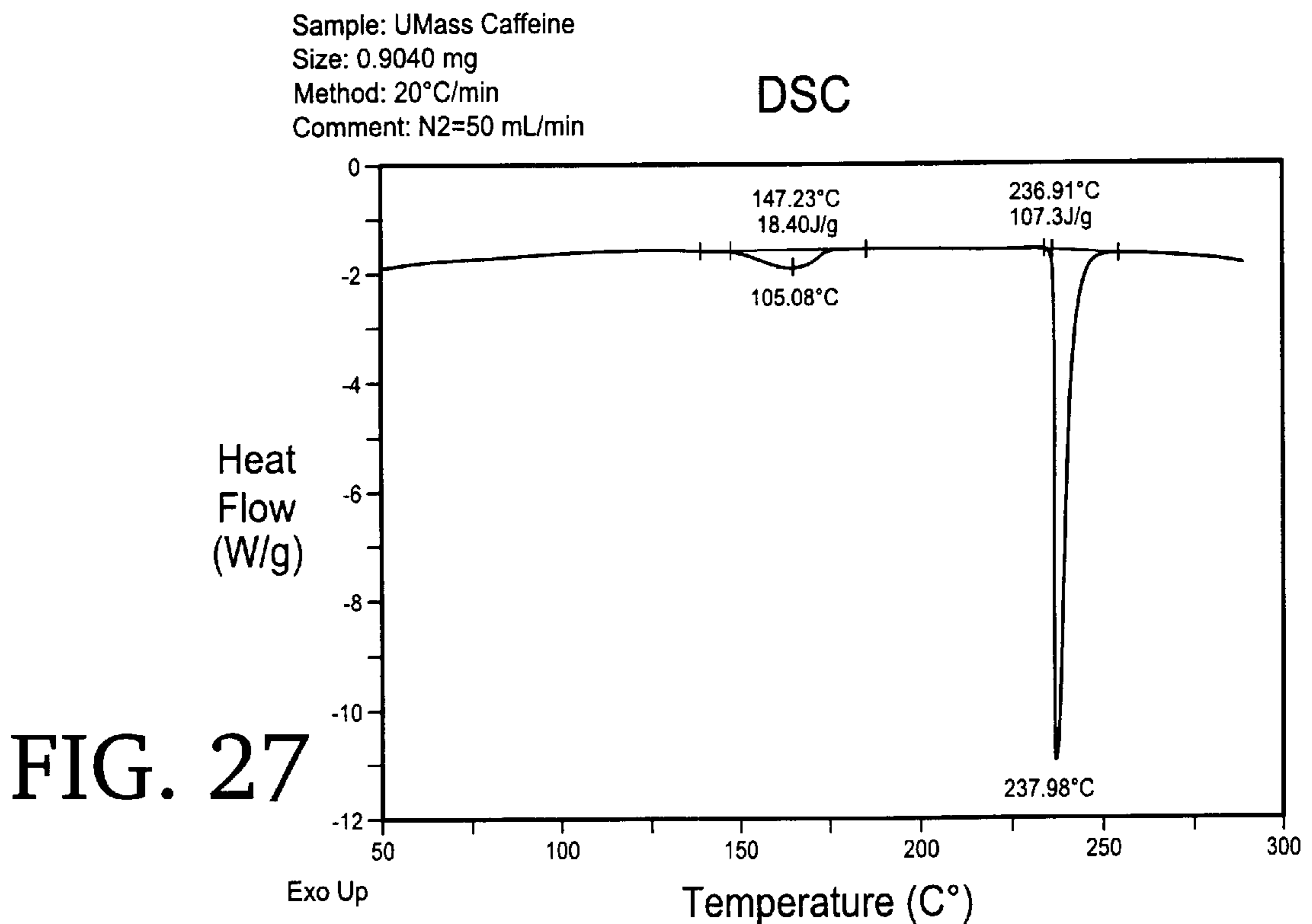
DSC thermogram of caffeine, a non-explosive, sample weight is 0.904 mg
