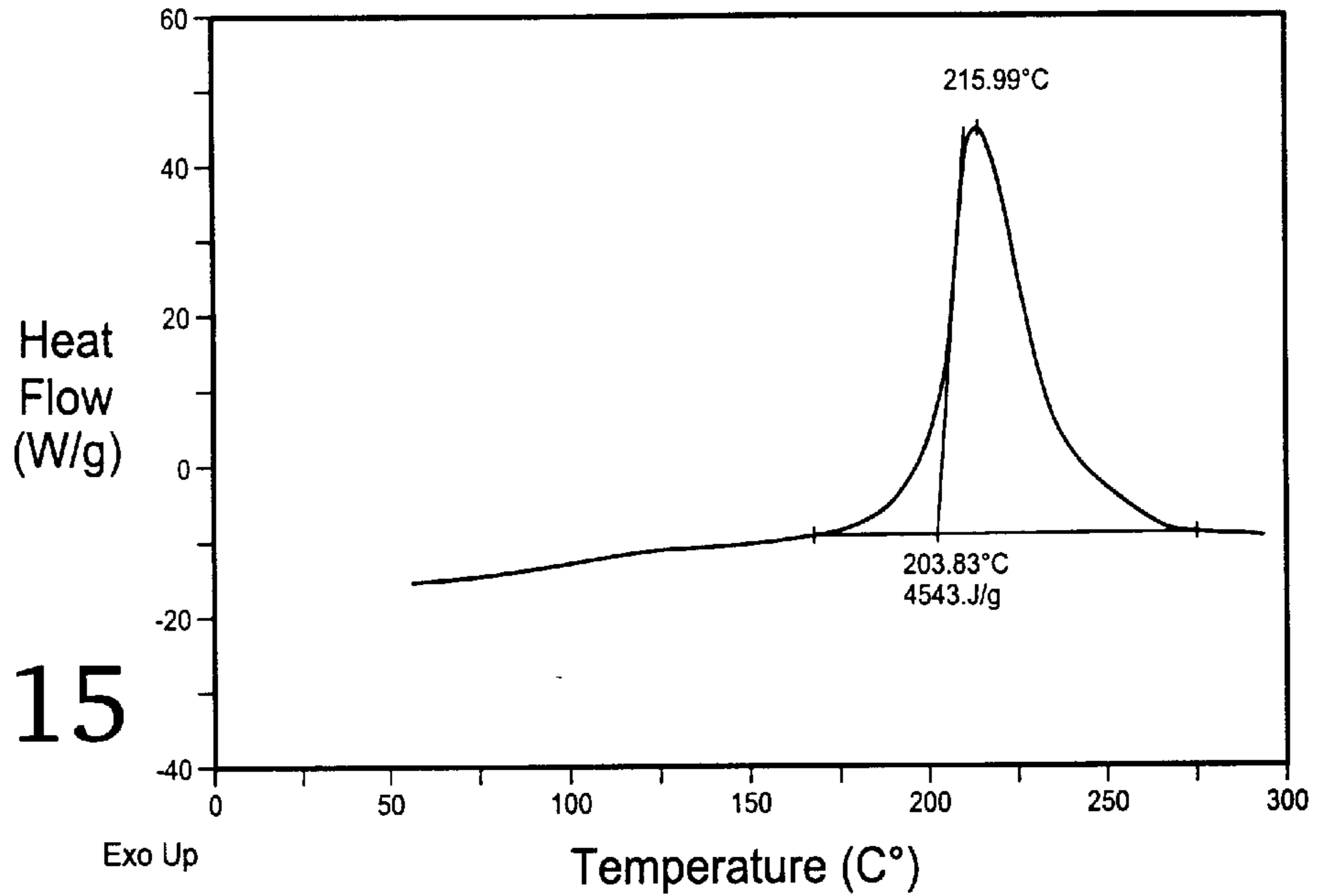
DSC thermogram of Smokeless Remington,, sample weight is 0.071 mg
