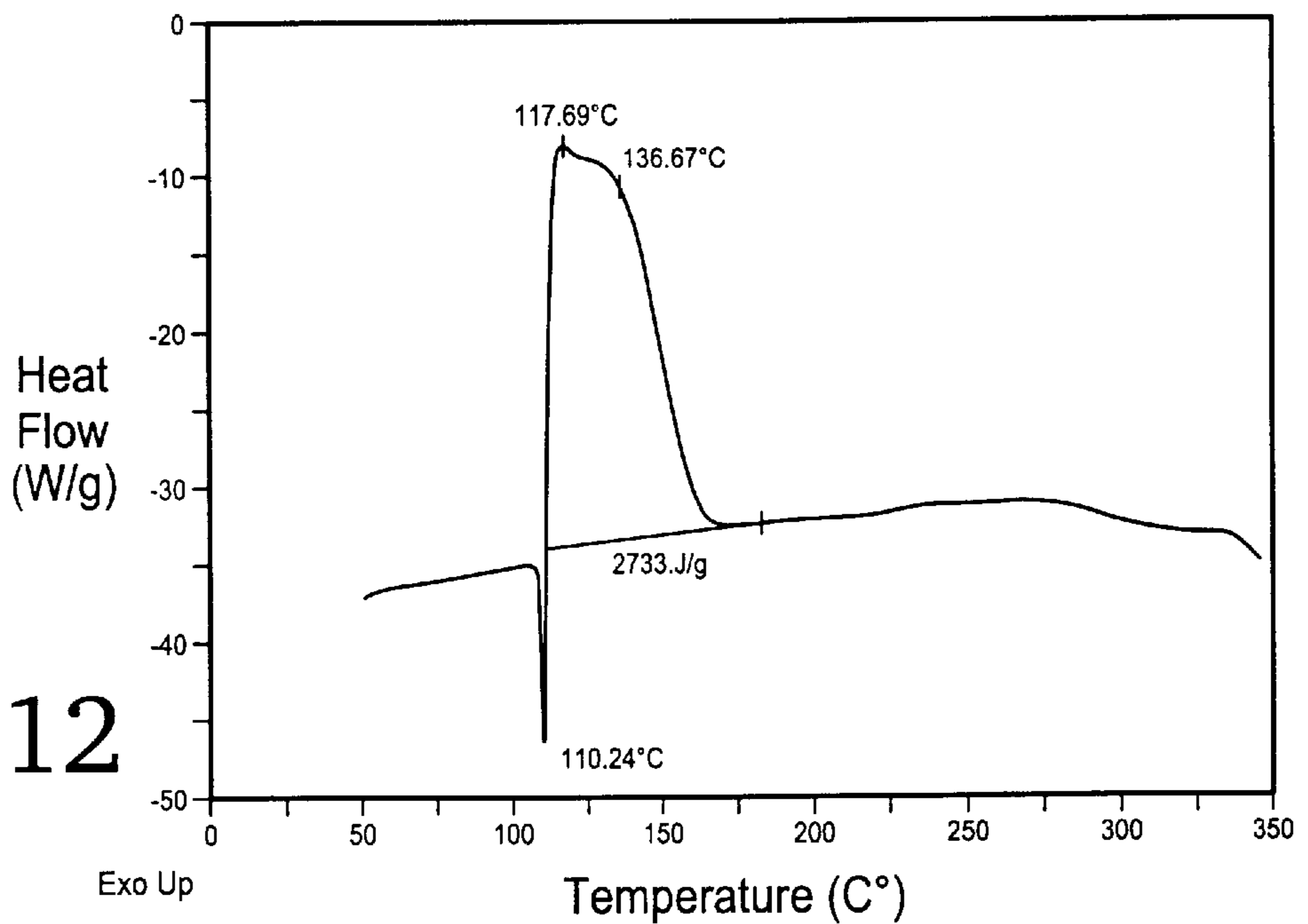
DSC thermogram of Benzoyl Peroxide, sample weight is 0.071 mg
