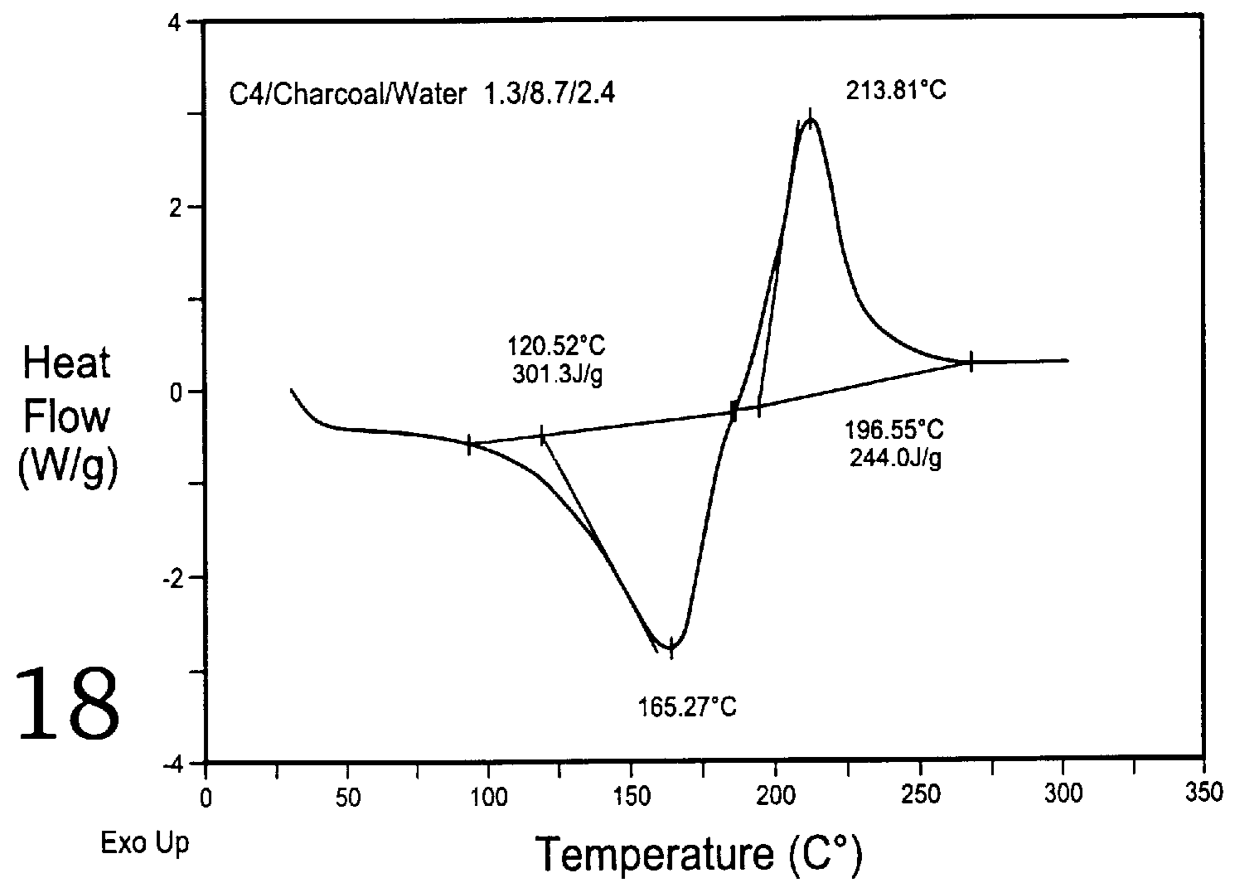
DSC thermogram of C4/Water/Charcoal, sample weight is 12.3 mg
