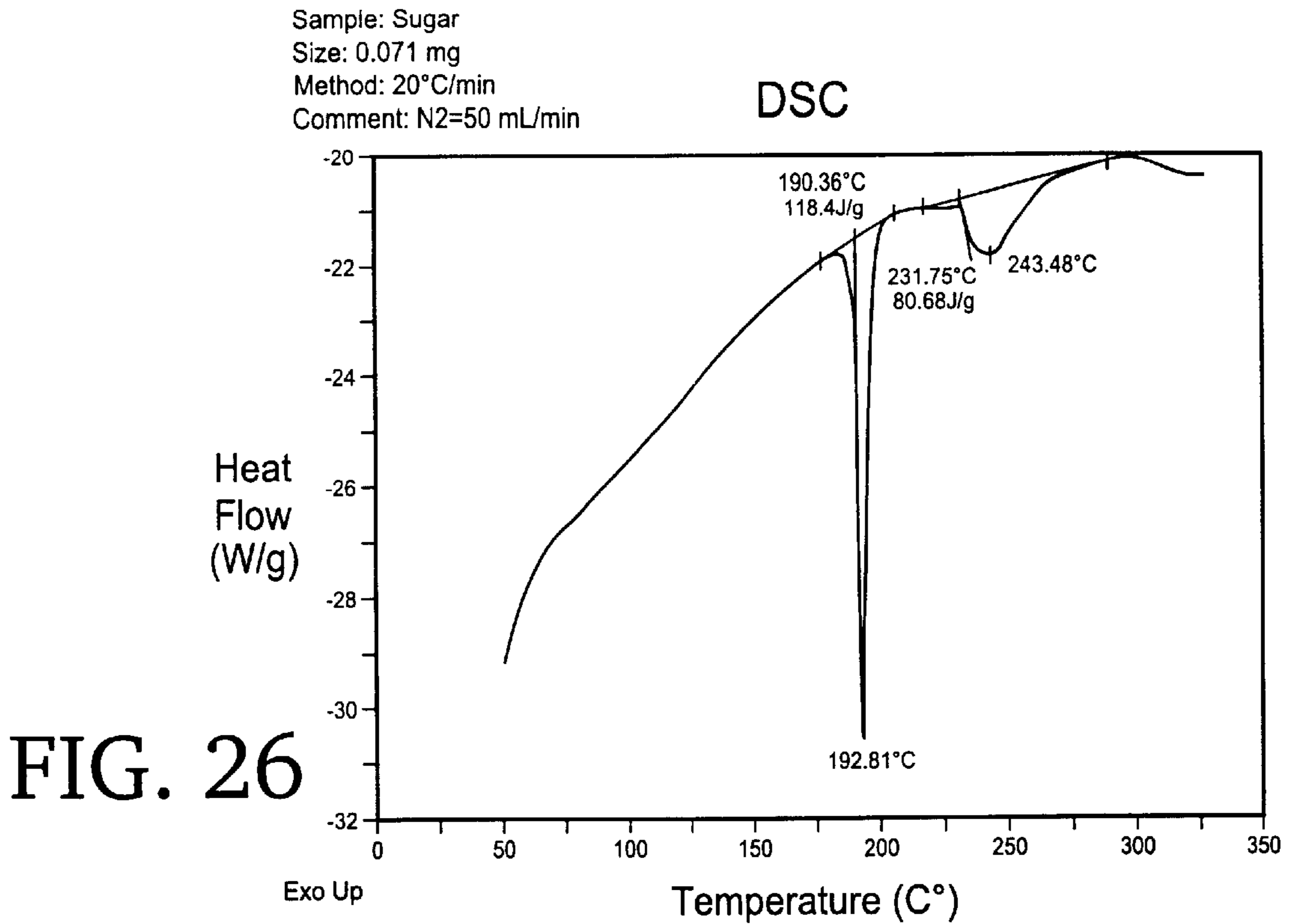
DSC thermogram of Sugar, sample weight is 0.071 mg
