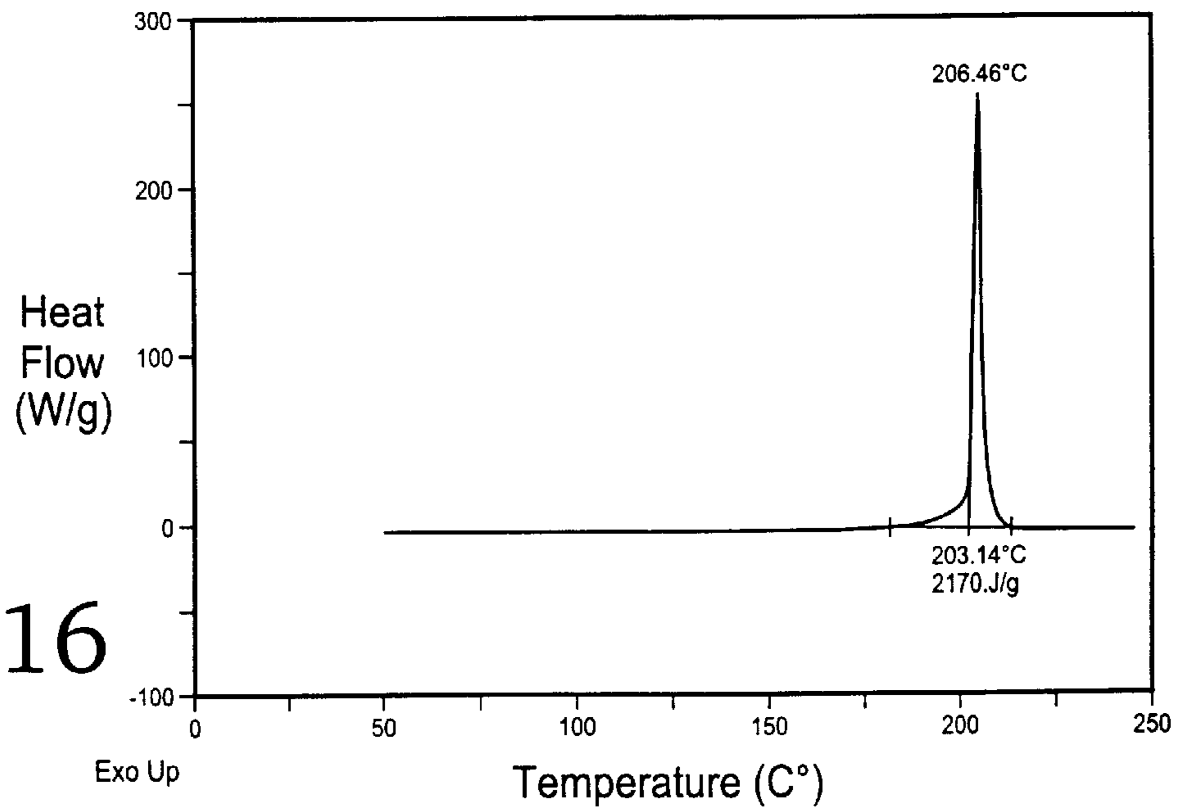
DSC thermogram of Mil. Spec. Ammo., sample weight is 0.215 mg
