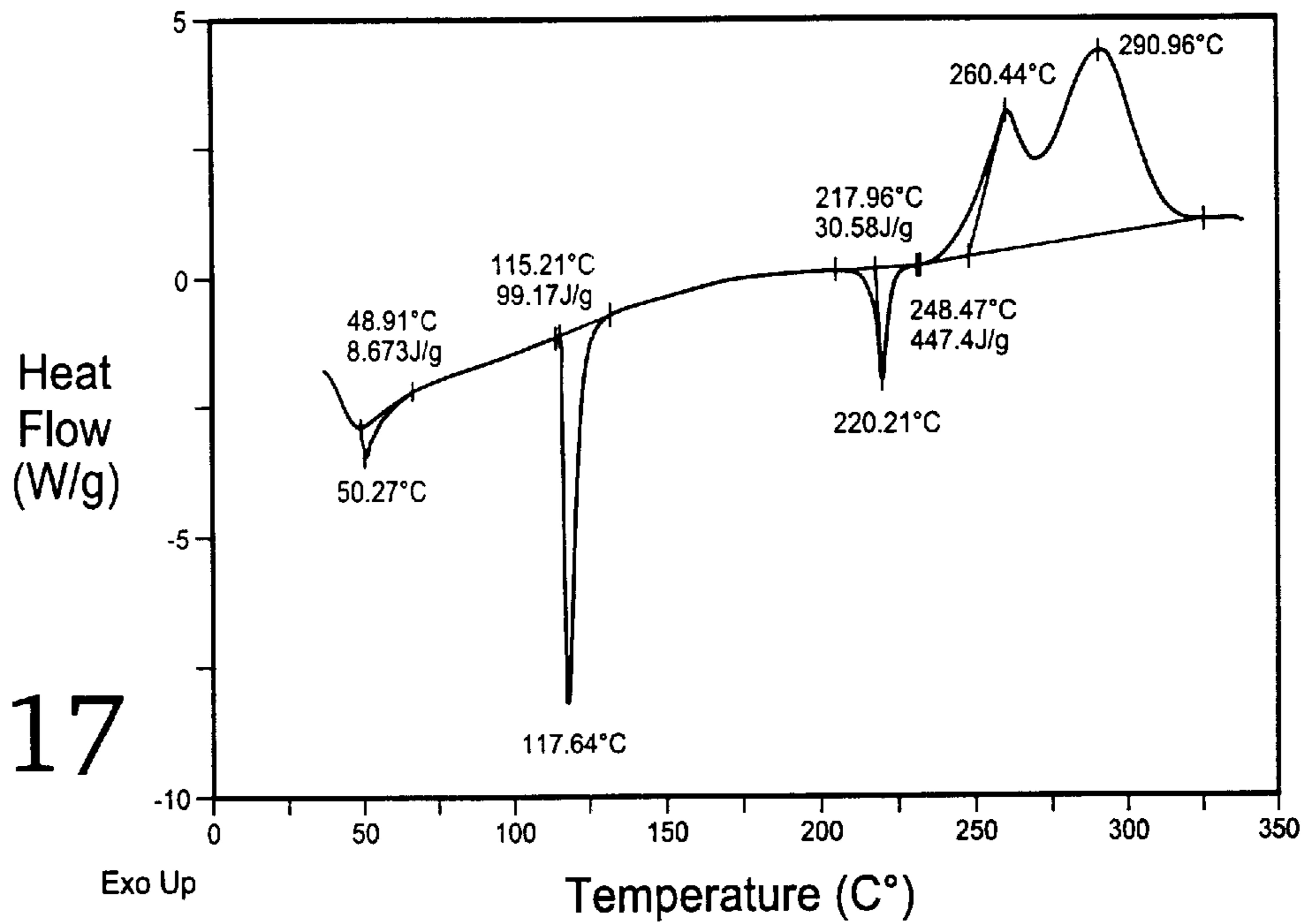
DSC thermogram of 2,3-dimethyl-2,3-dinitrobutane, sample weight is 0.184 mg
