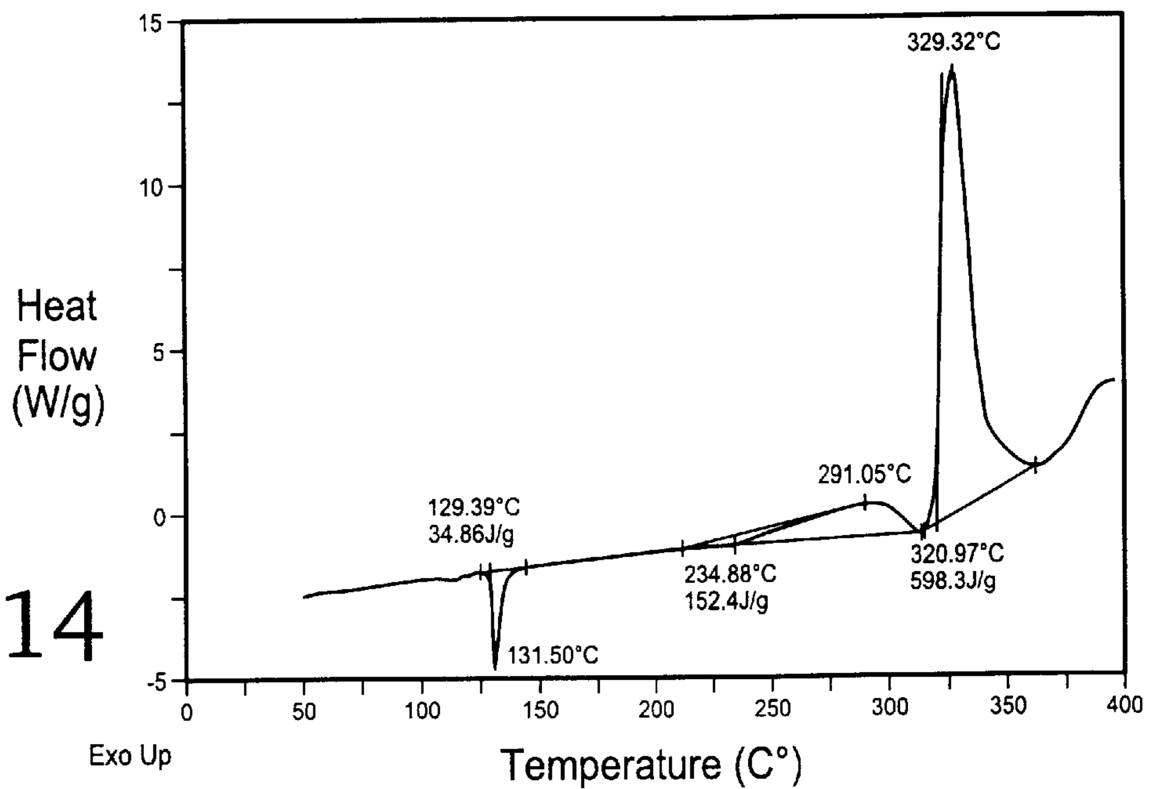
DSC thermogram of Black Powder, sample weight is 0.489 mg
