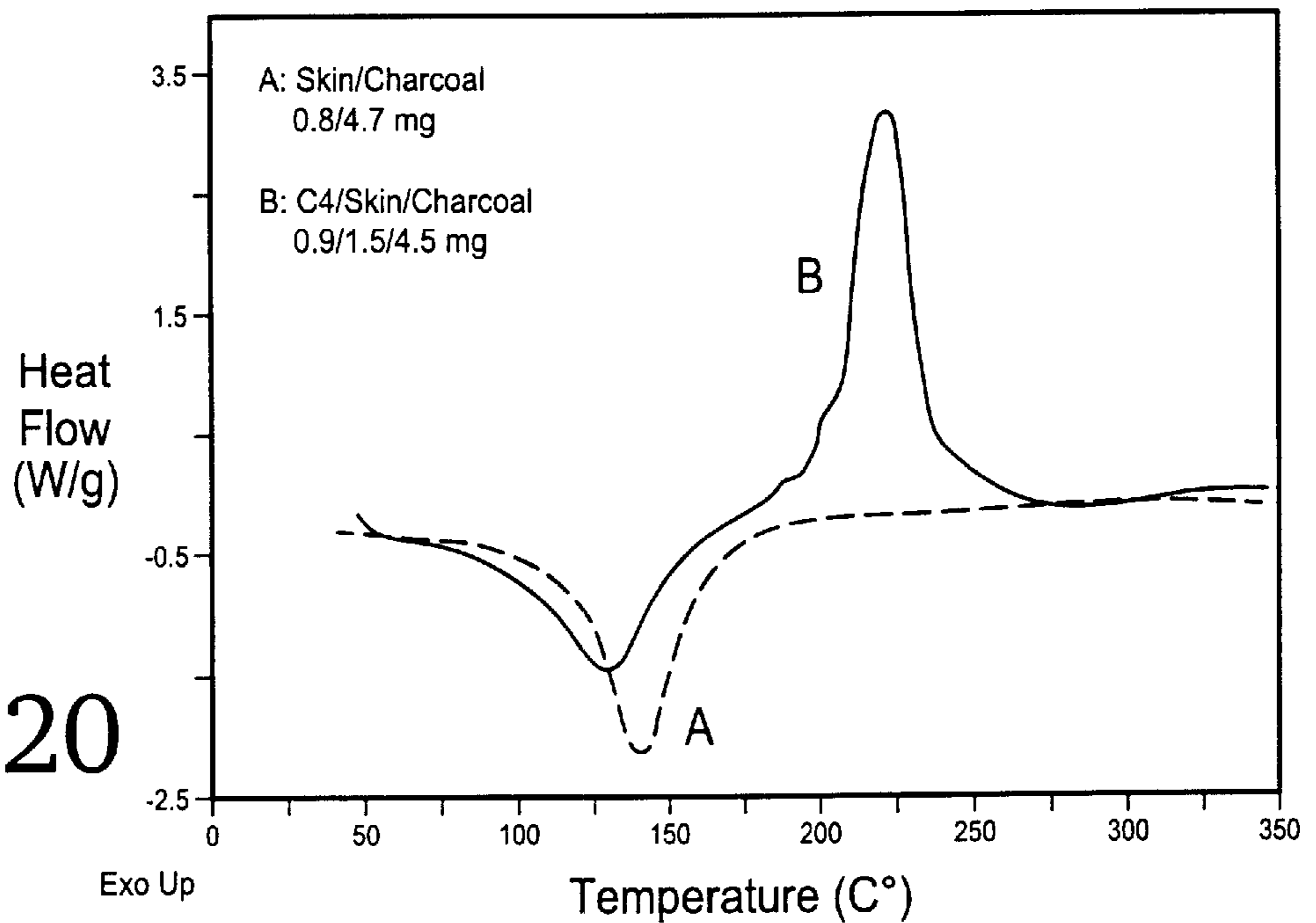
DSC thermogram for Charcoal/Skin Fragments, and for Charcoal/Skin/C4 mixture
