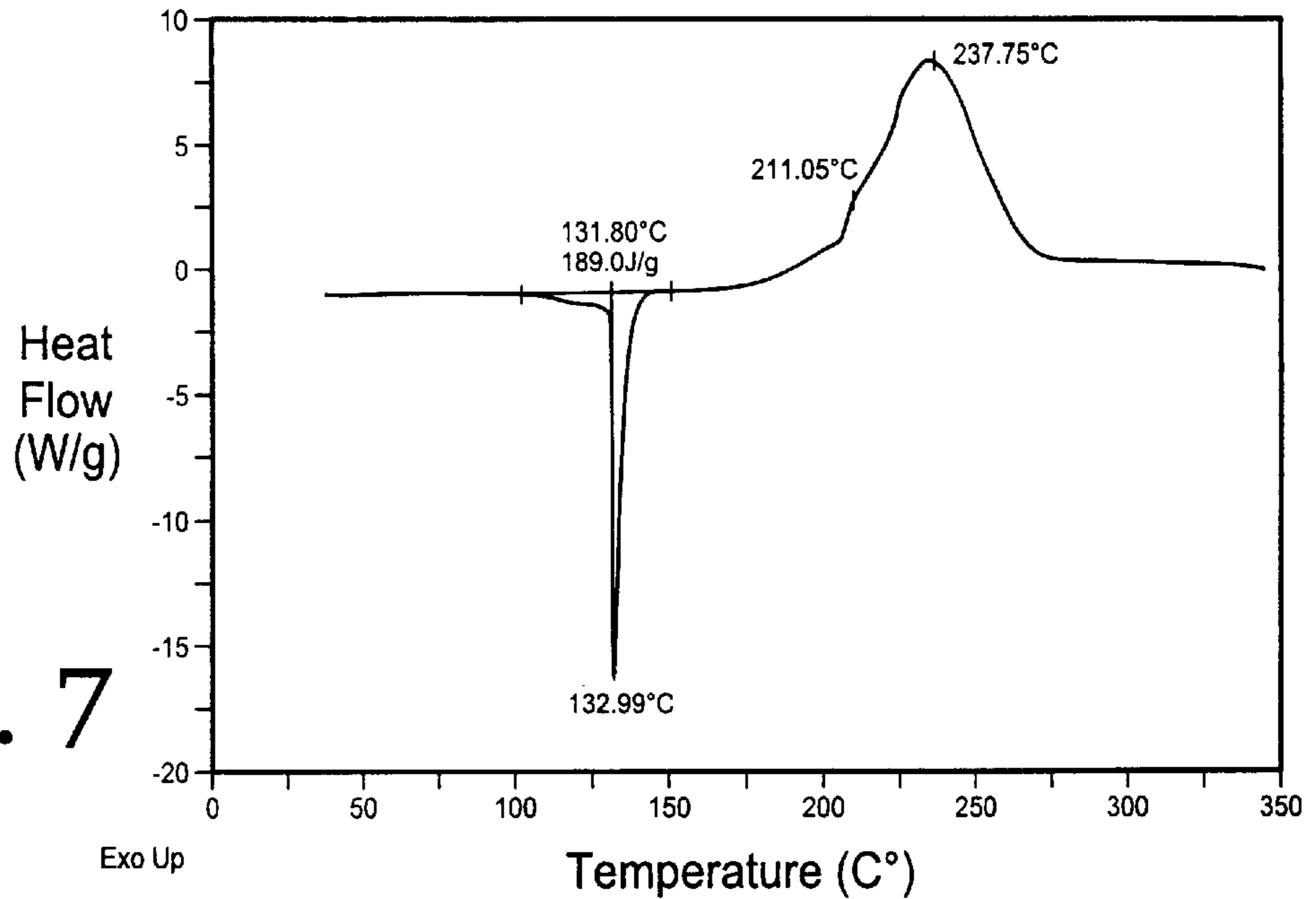
DSC thermogram of DADP, sample weight is 0.699 mg
