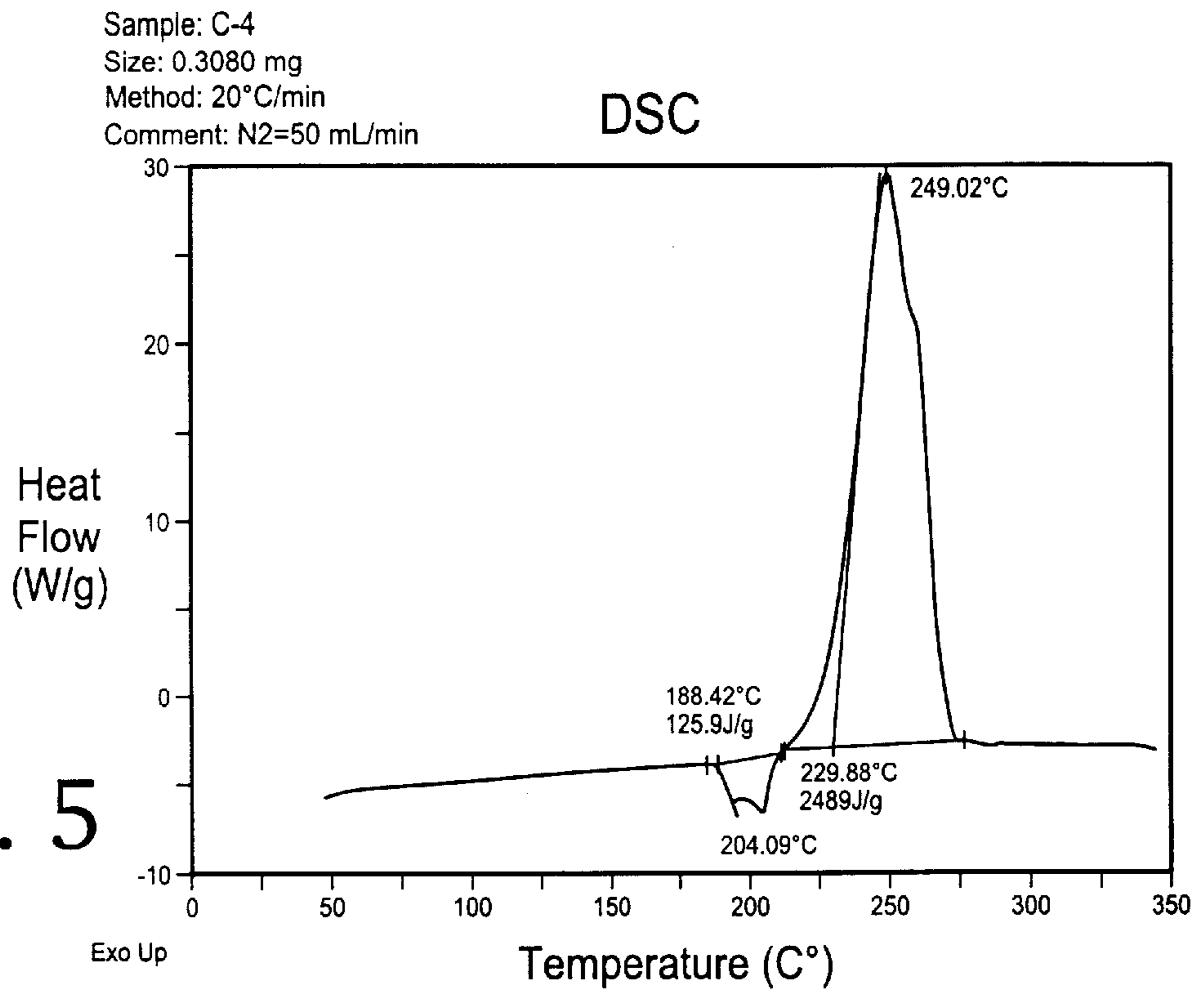
DSC thermogram of C-4, sample weight is 0.308 mg
