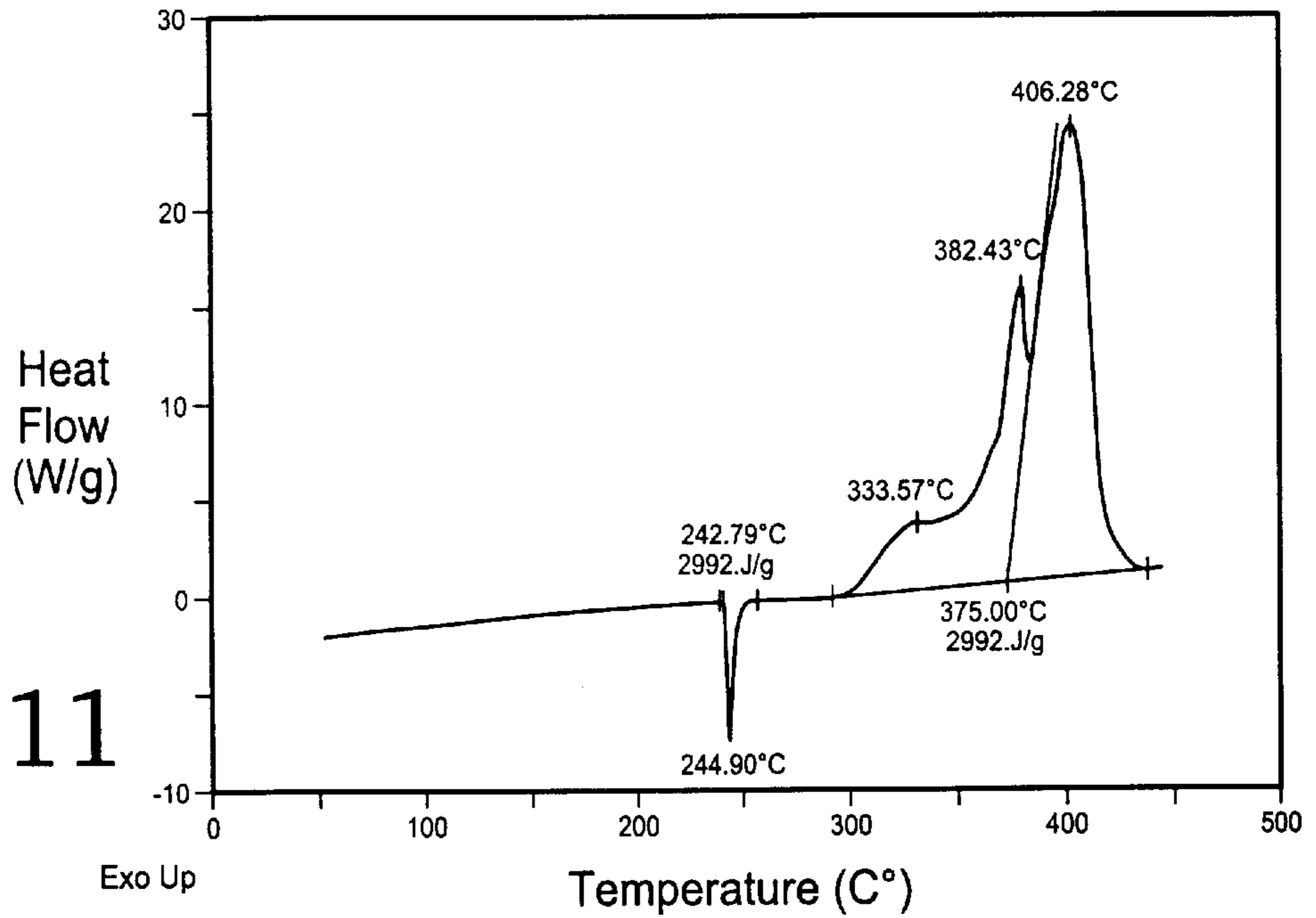
DSC thermogram of Ammonium Perchlorate, sample weight is 0.444 mg
