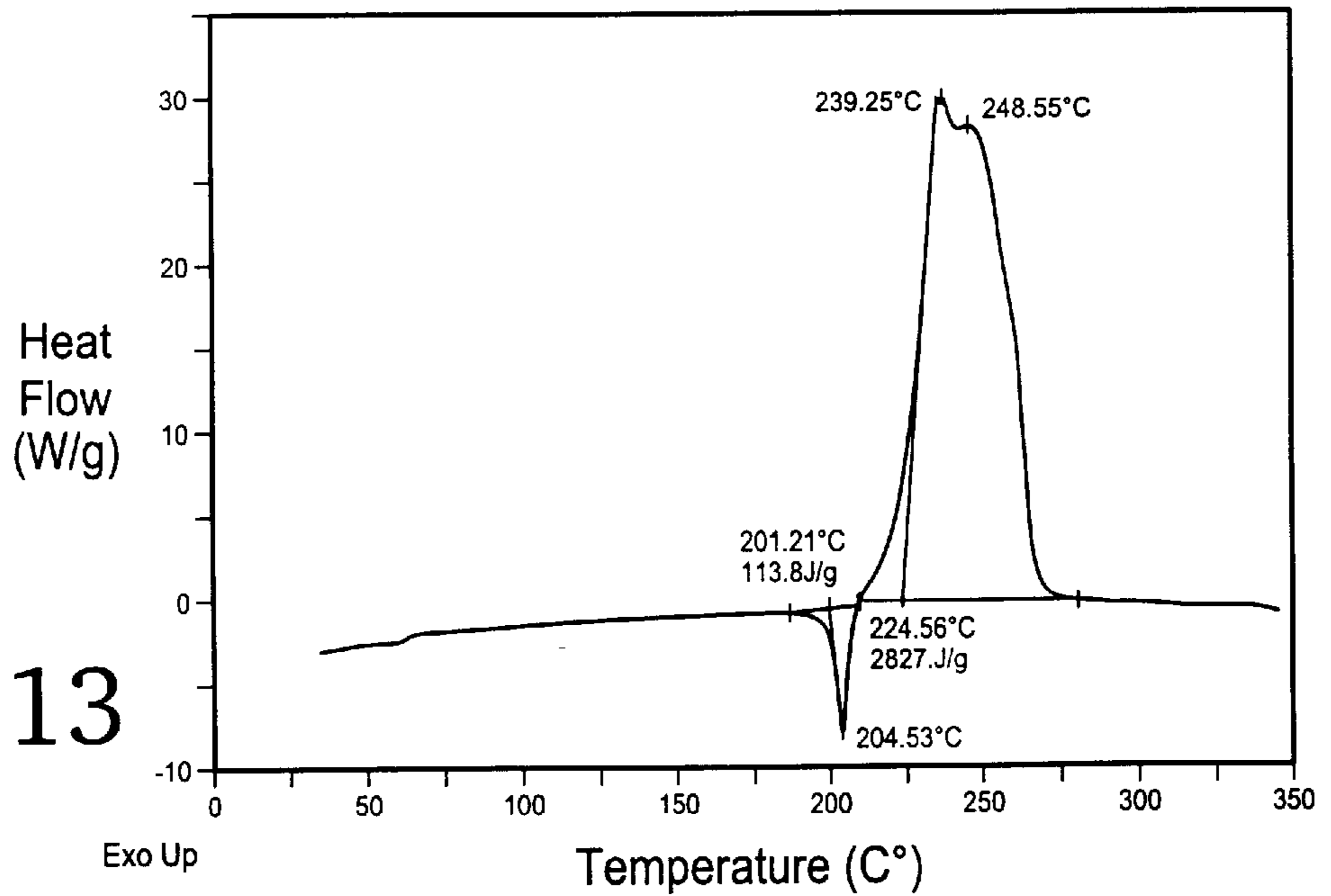
DSC thermogram of RDX, sample weight is 0.400 mg
