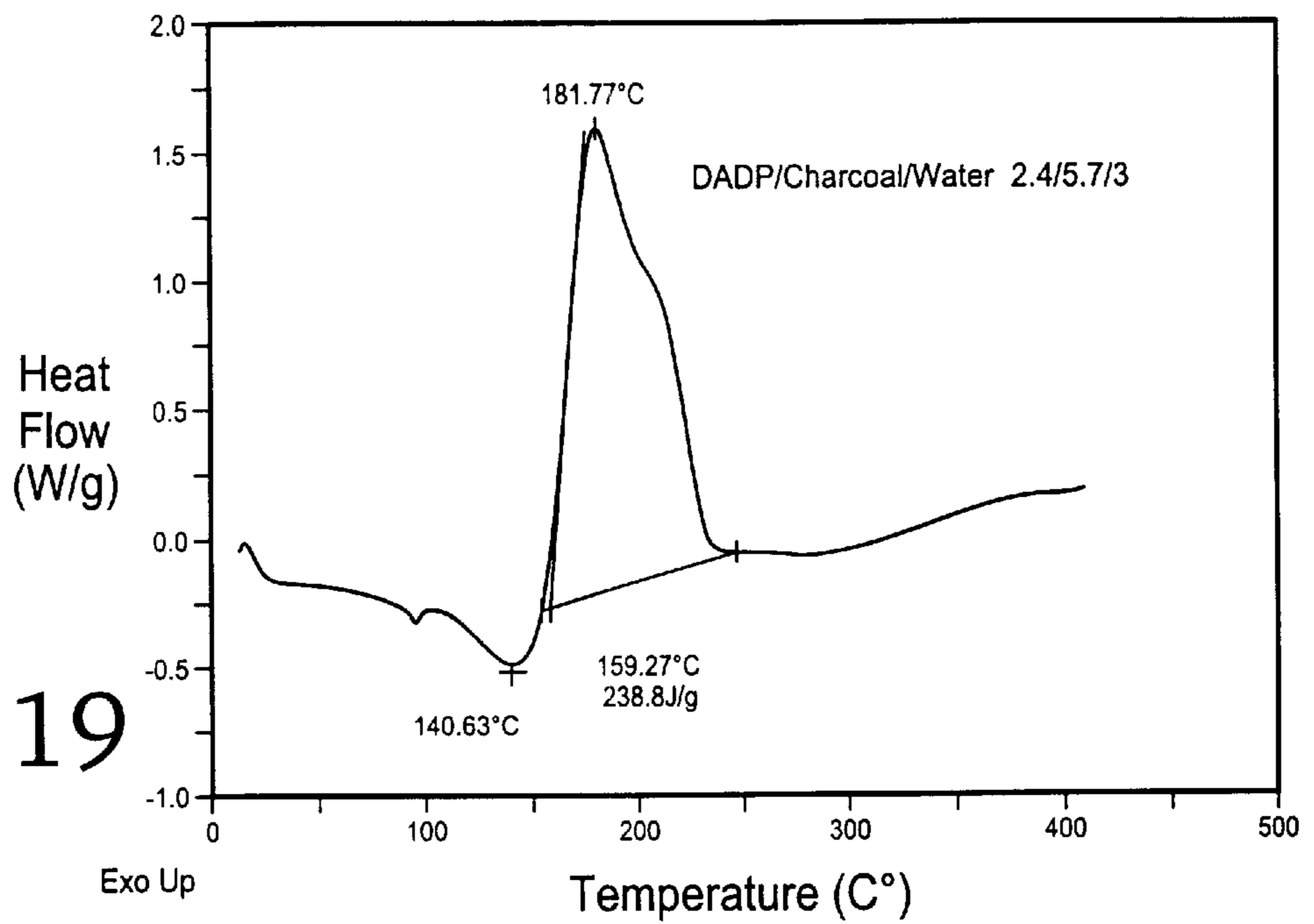
DSC thermogram of DADP/Water/Charcoal, sample weight is 11.1 mg
