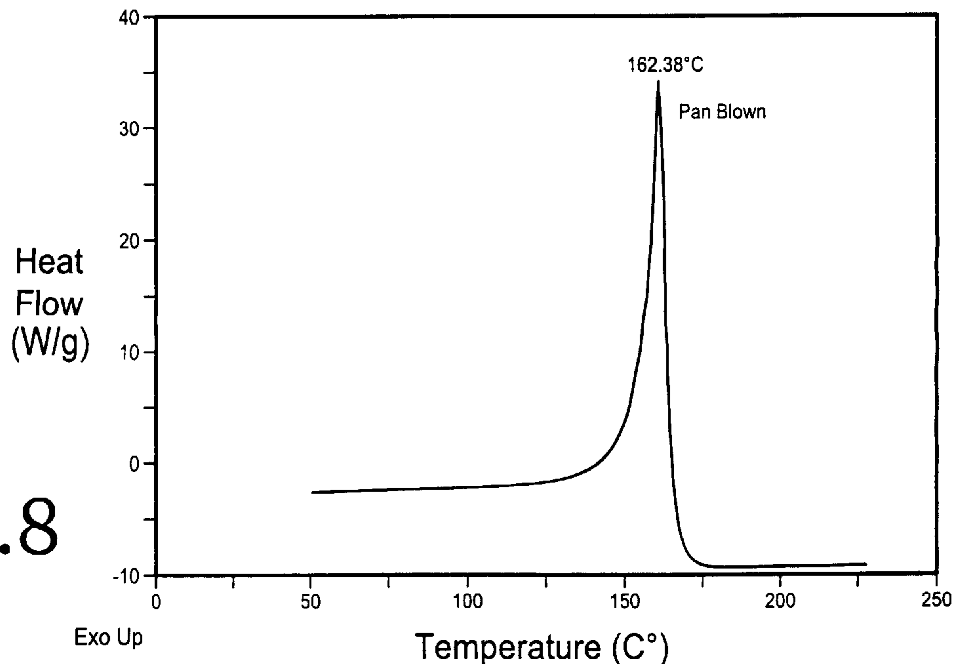
DSC thermogram of HMTD, sample weight is 0.44 mg
