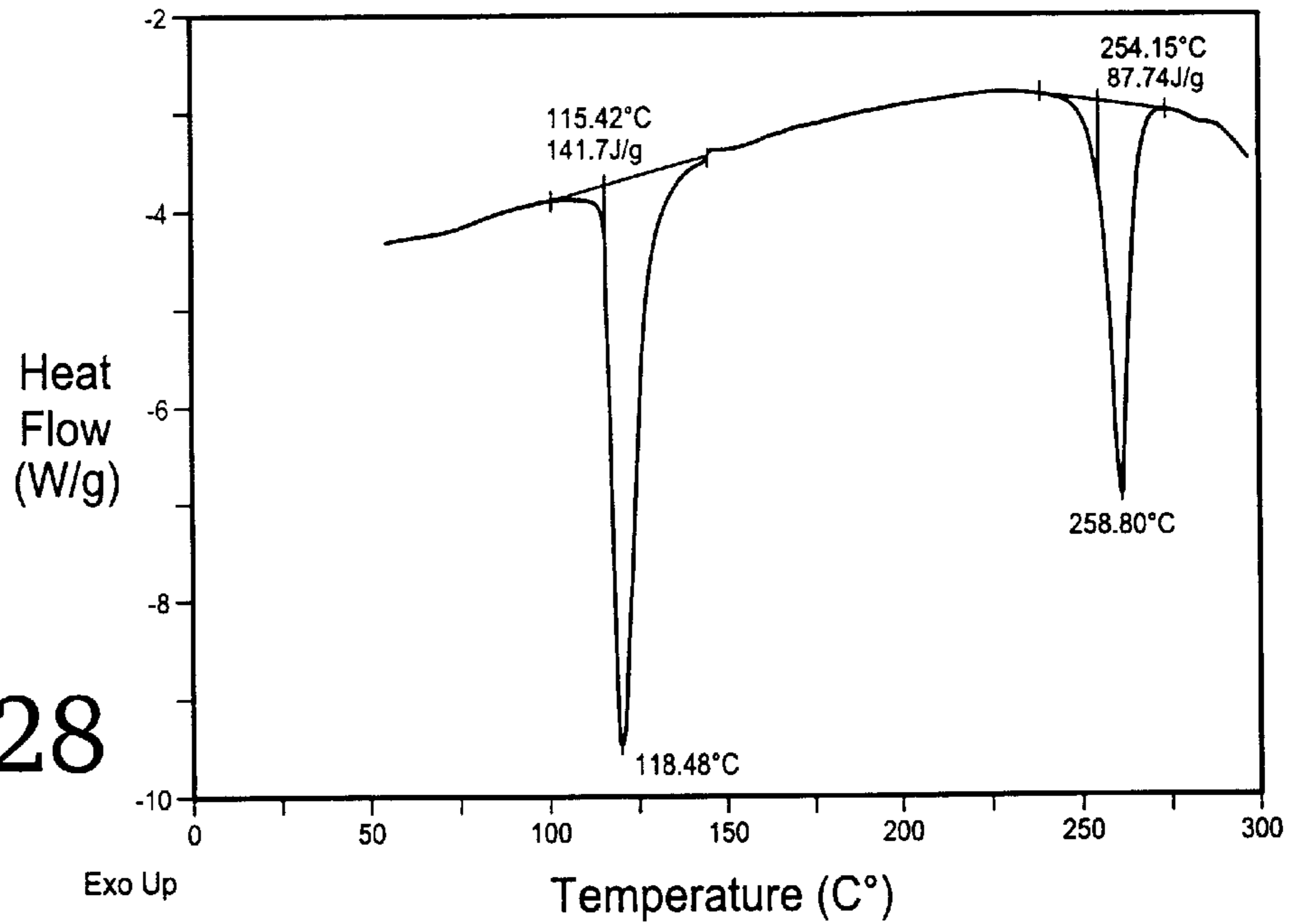
DSC thermogram of Bupivacaine, sample weight is 0.321 mg
