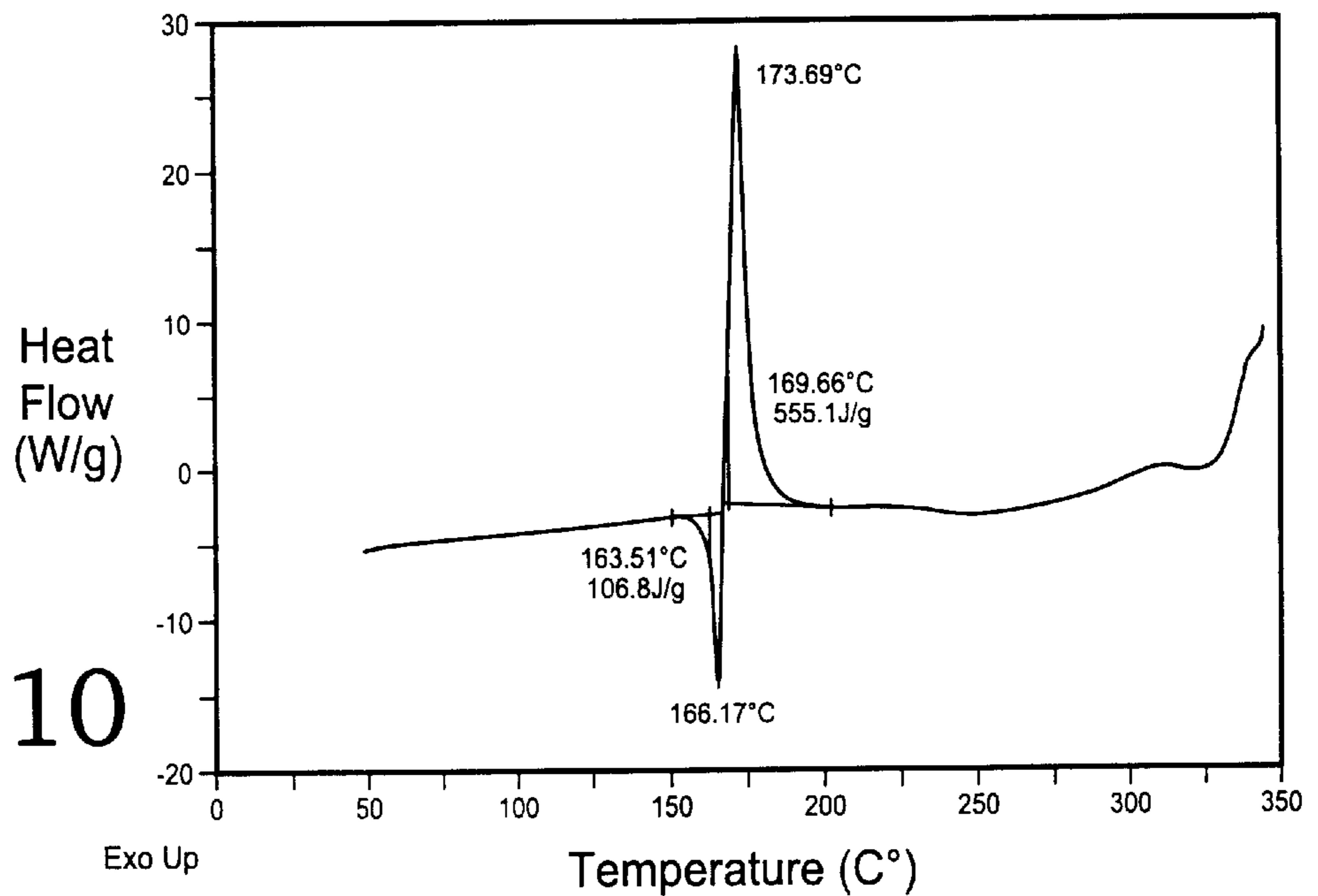
DSC thermogram of Urea Nitrate, sample weight is 0.211 mg
