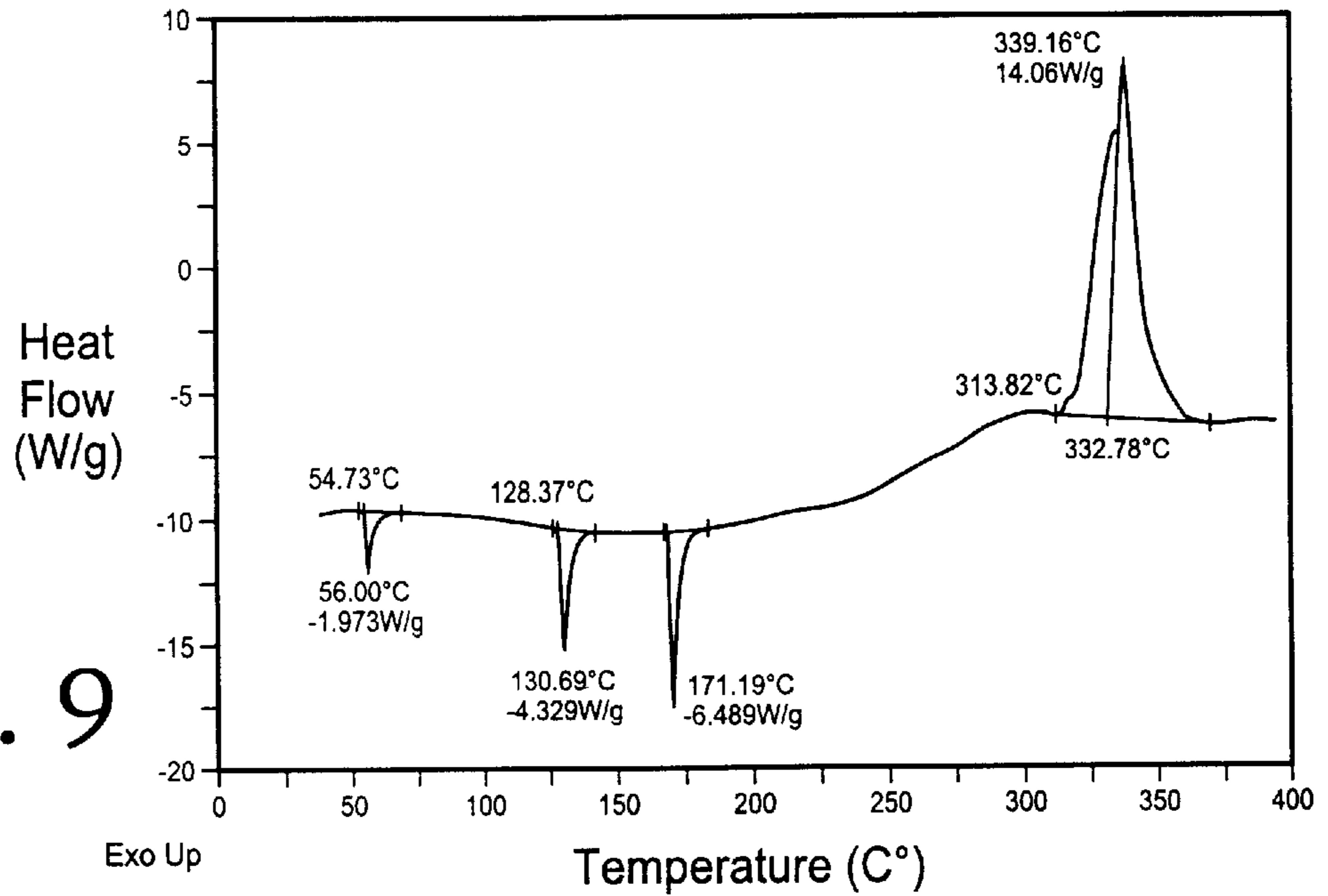
DSC thermogram of Ammonium Nitrate, sample weight is 0.09 mg
