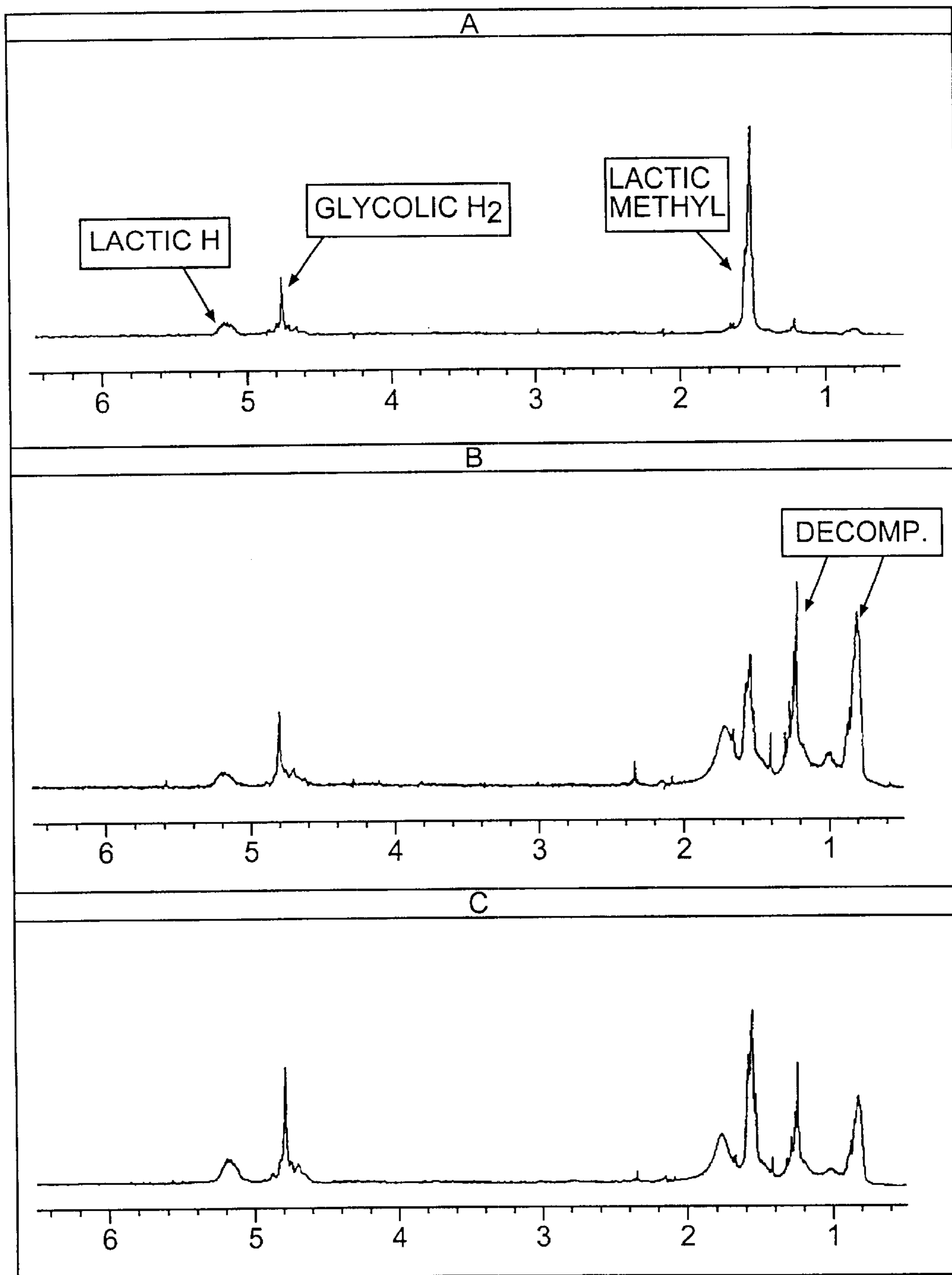
1 H-NMR SPECTRA OF A) ORIGINAL PLGA, B) DEPOSITED PLGA AT 200 mJ AT ATMOSPHERIC PRESSURE, AND C) NEAR ATMOSPHERIC PRESSURE(10 Torr).
