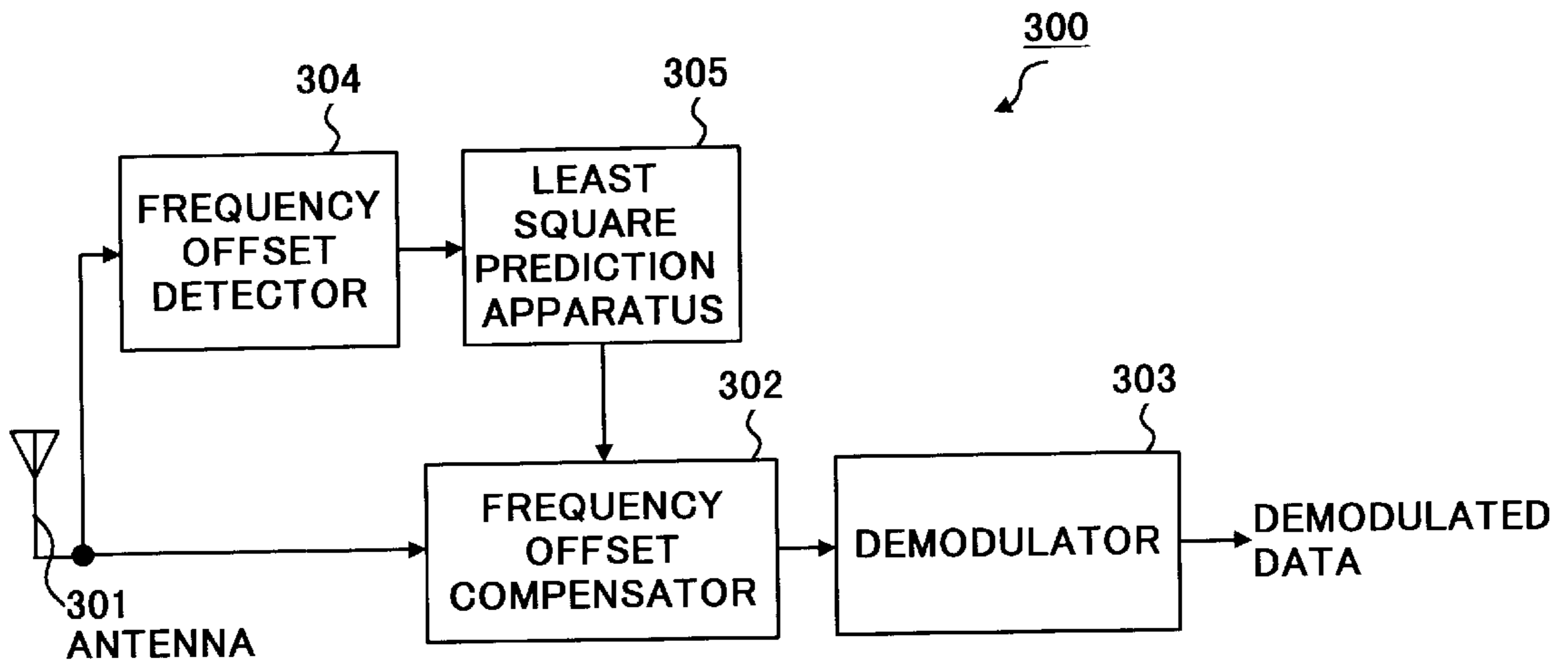
FIG.3 PRIOR ART
