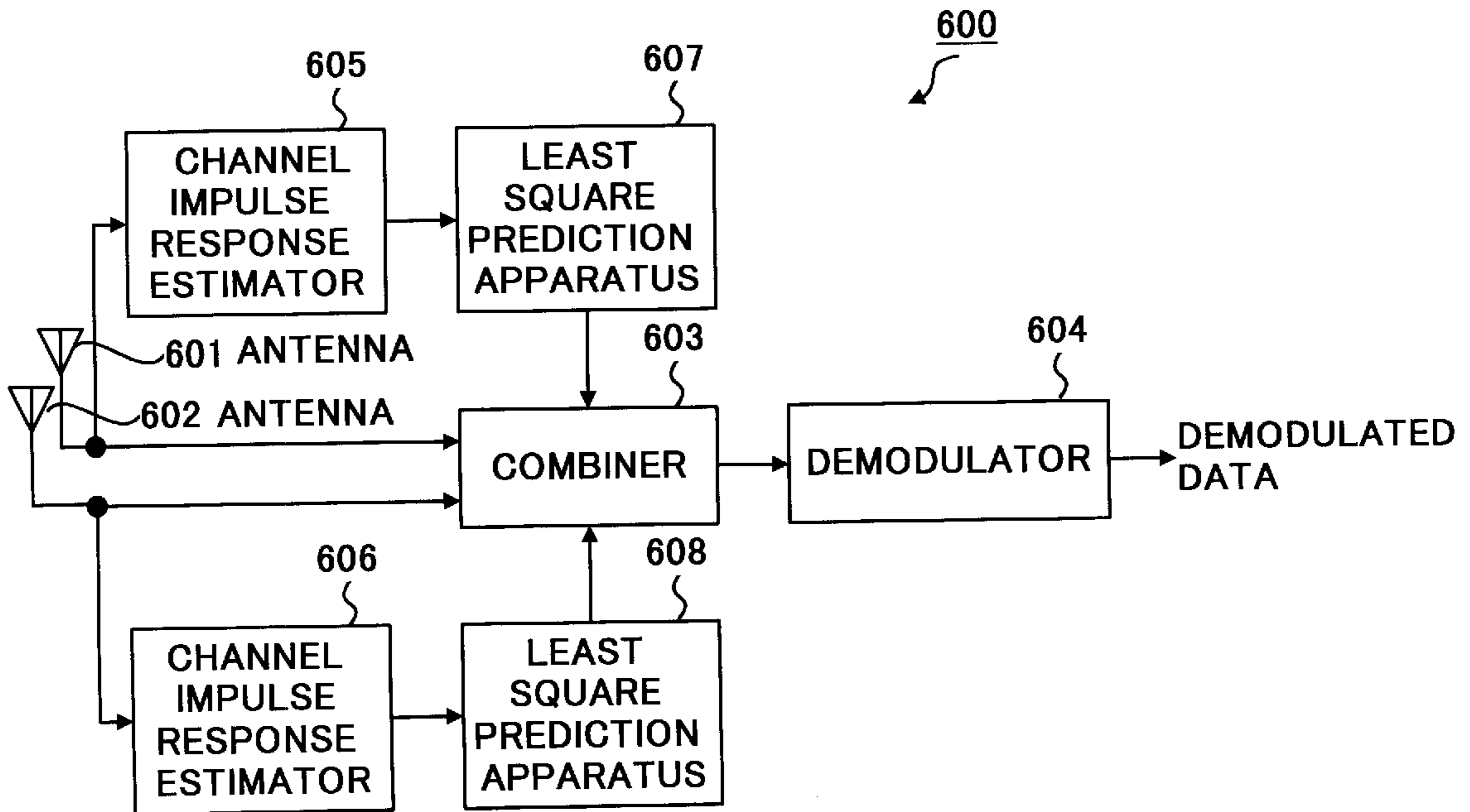
FIG.6 PRIOR ART
