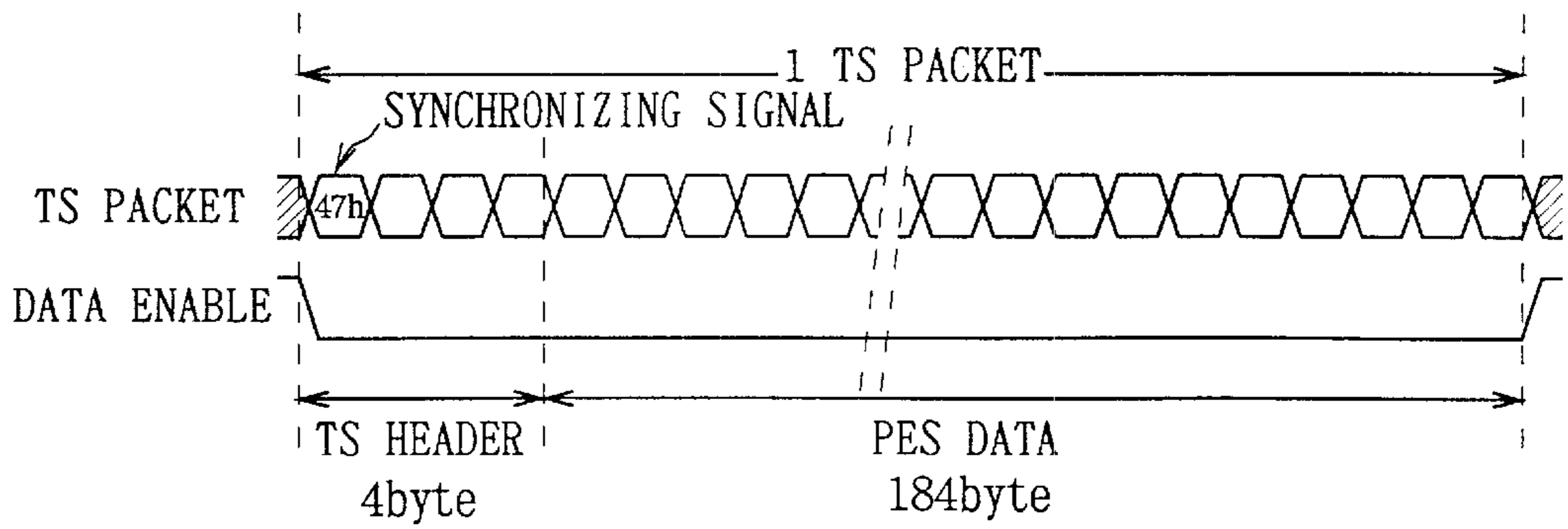
FIG. 6B(RELATED ART)
