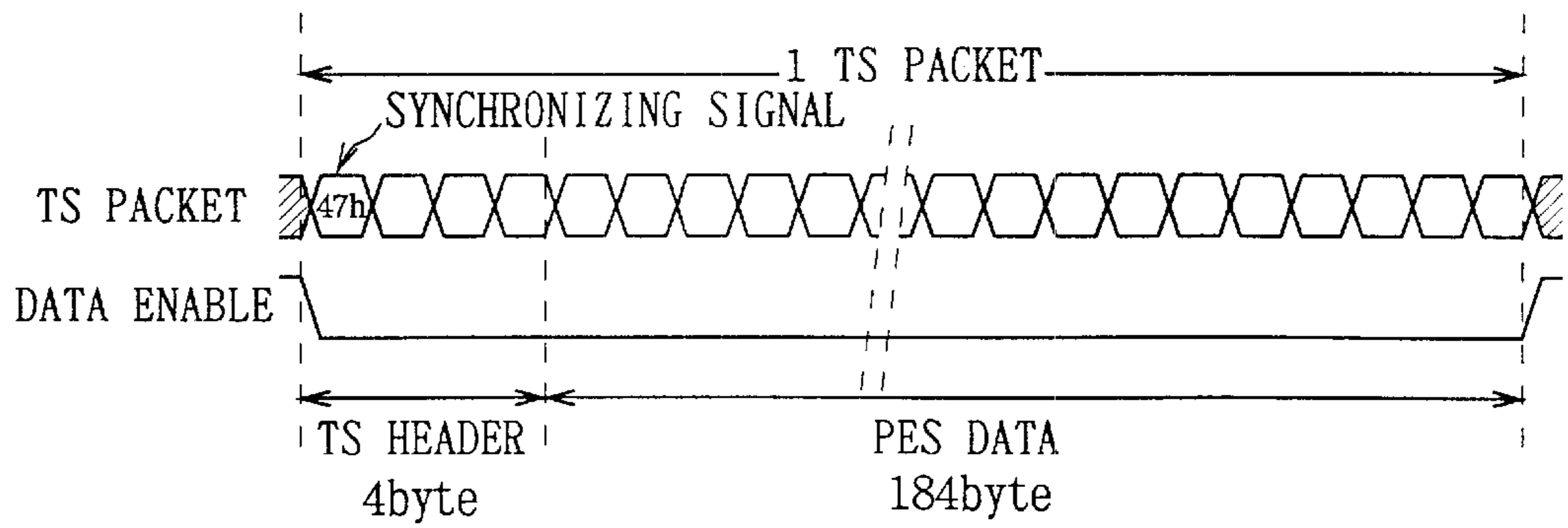
FIG. 6B(RELATED ART)
