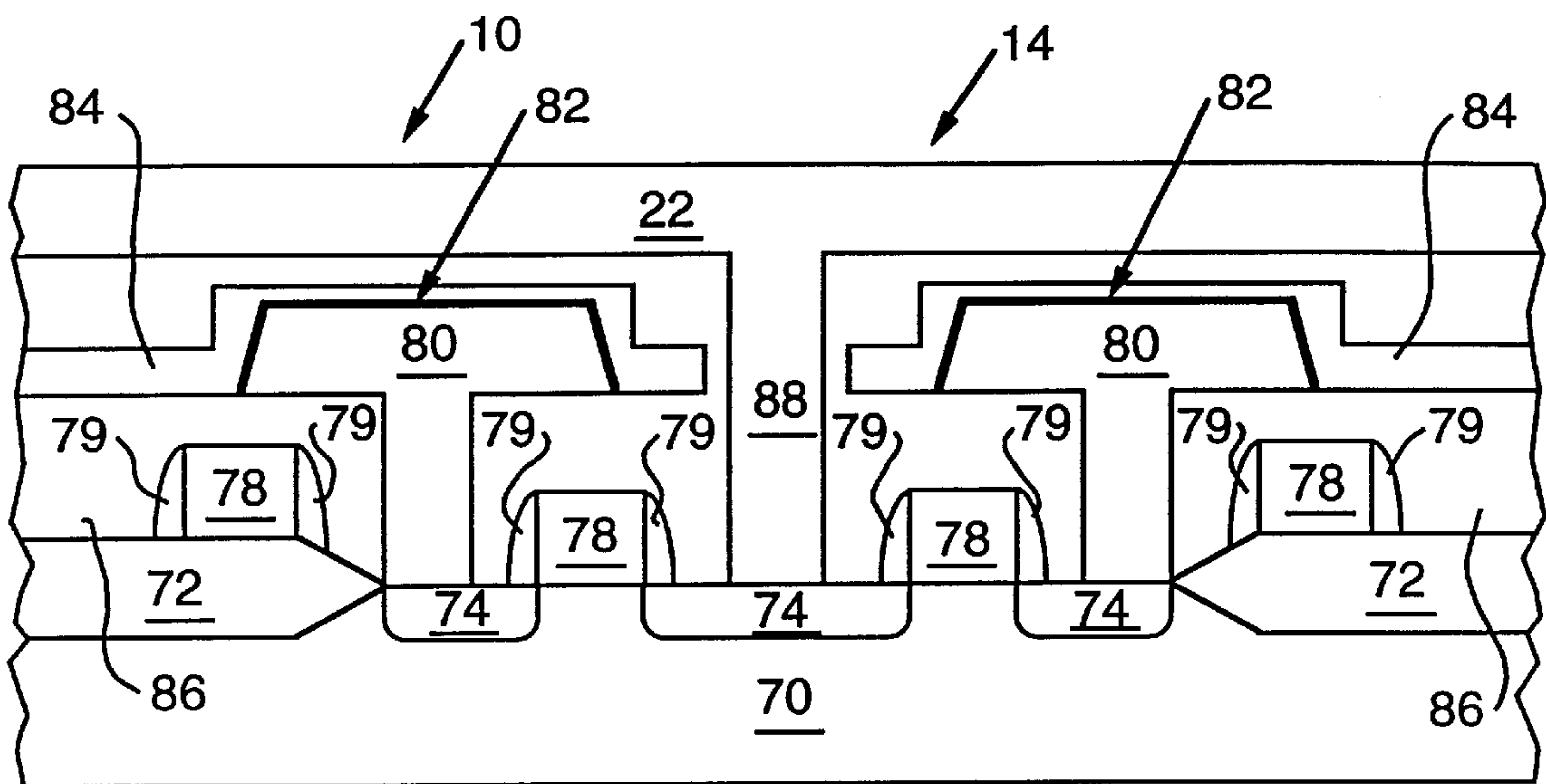
FIG. 2 Prior Art
