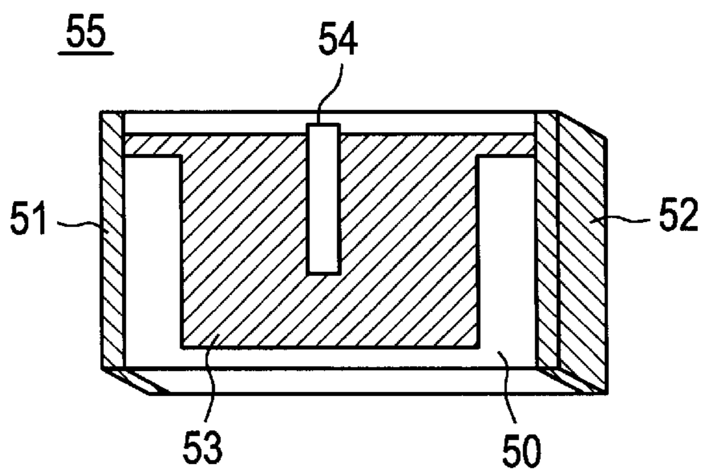
FIG. 5 PRIOR ART
