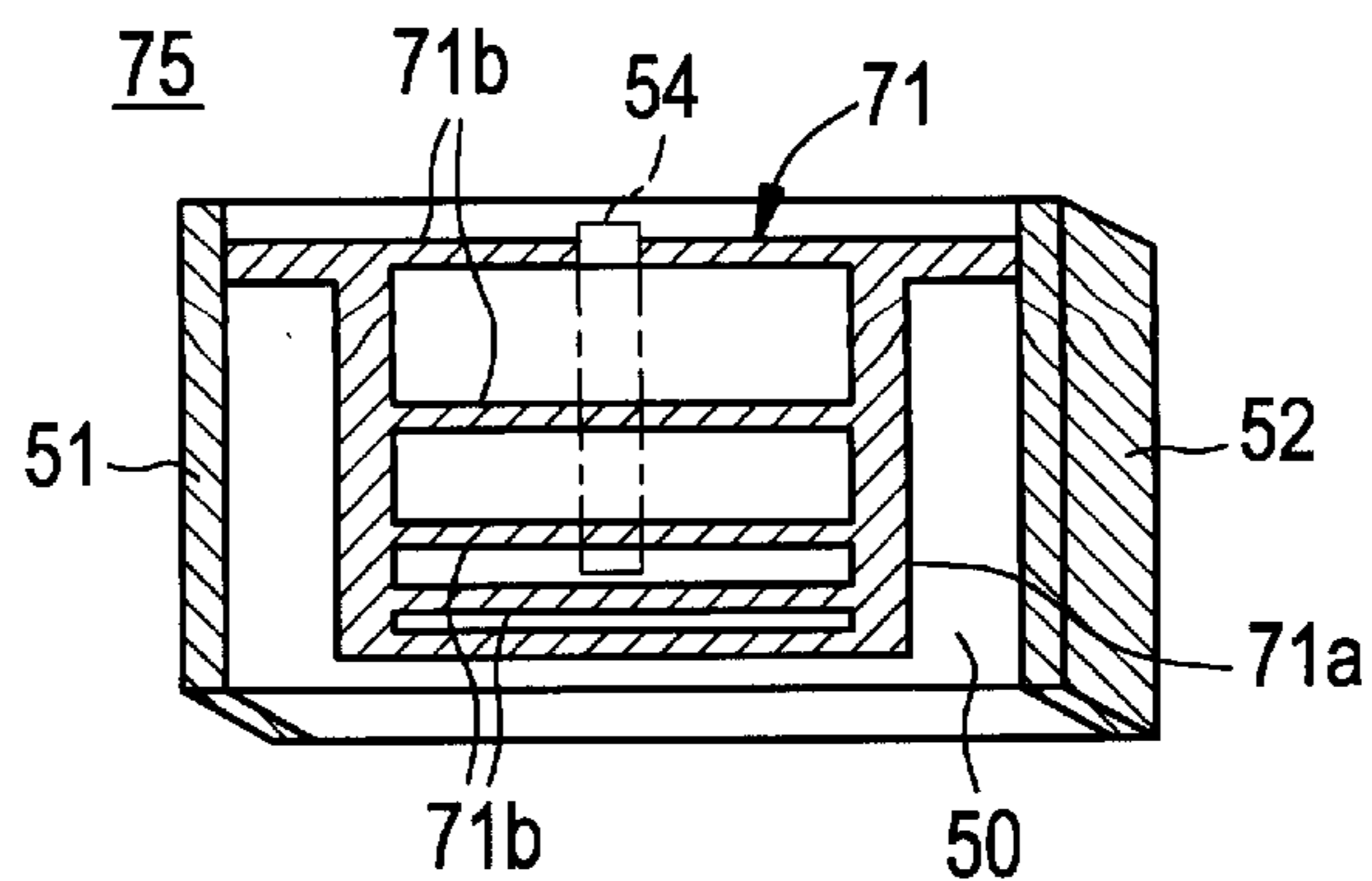
FIG. 6 PRIOR ART
