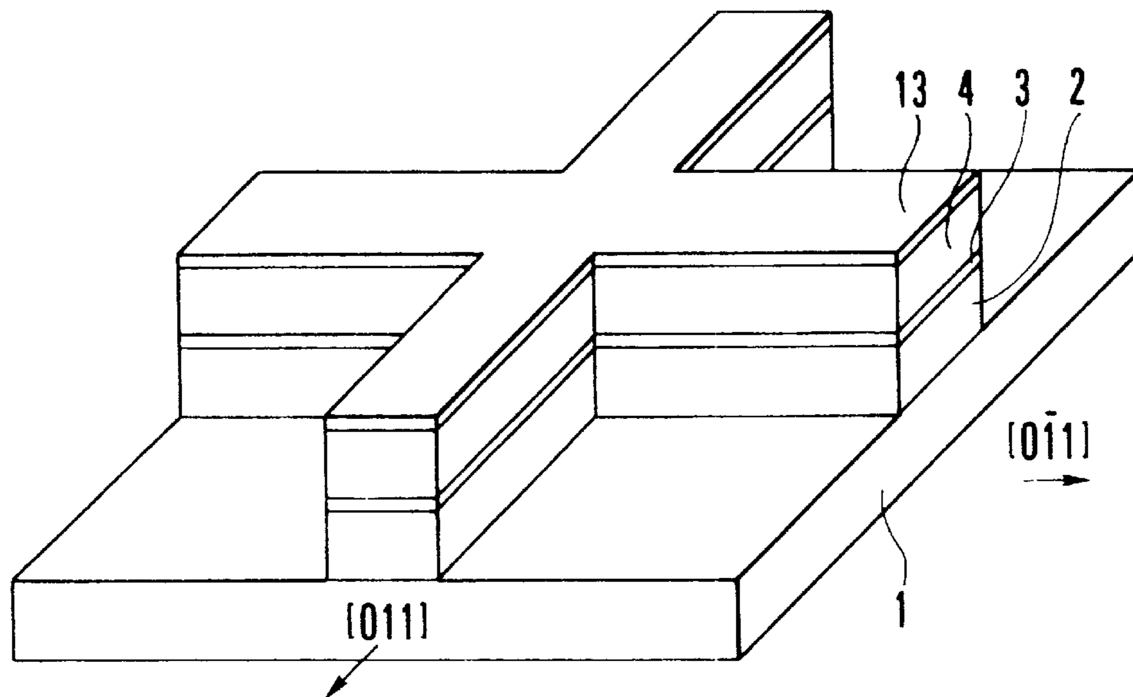
FIG. 32A PRIOR ART
