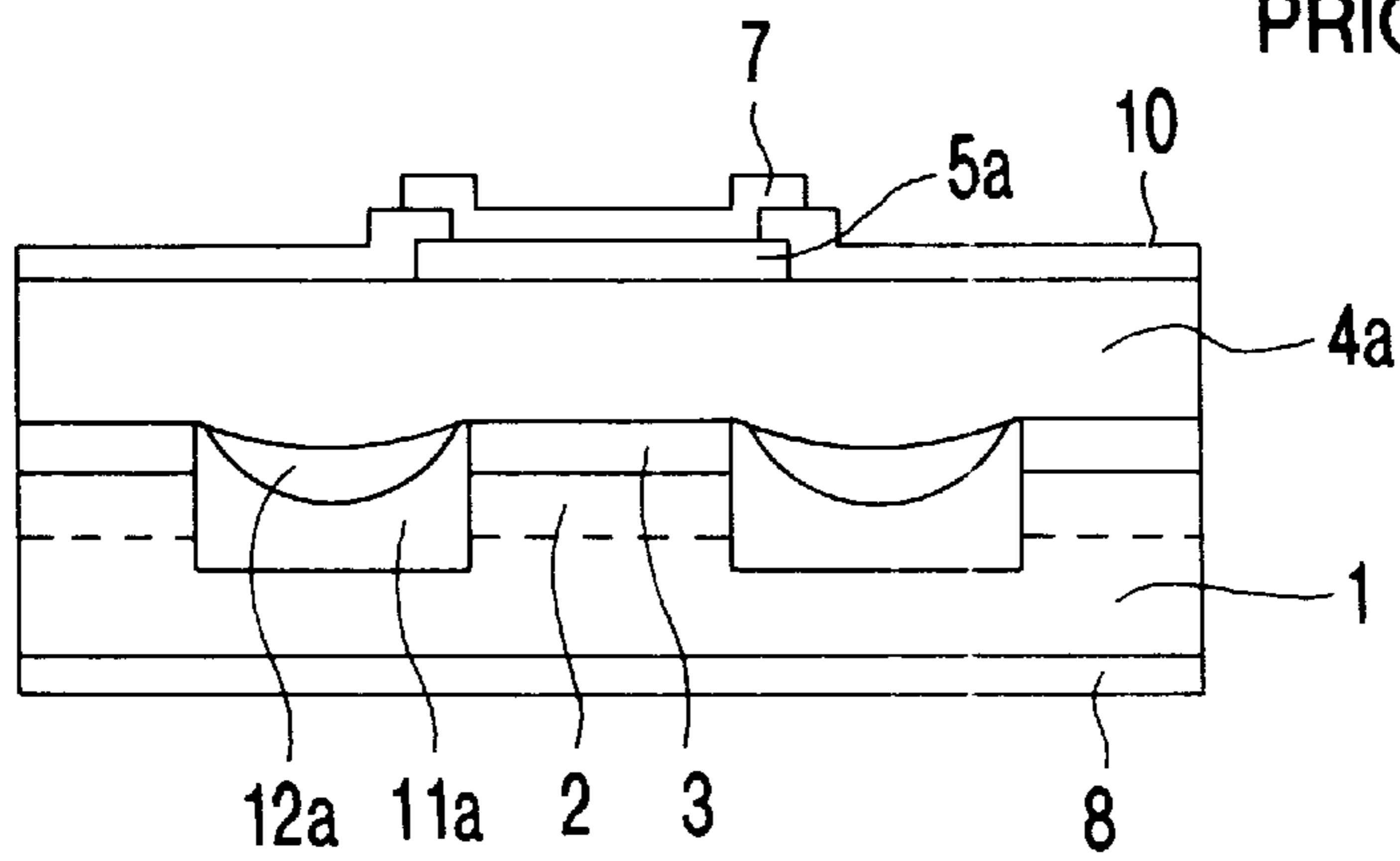
FIG. 30B PRIOR ART
