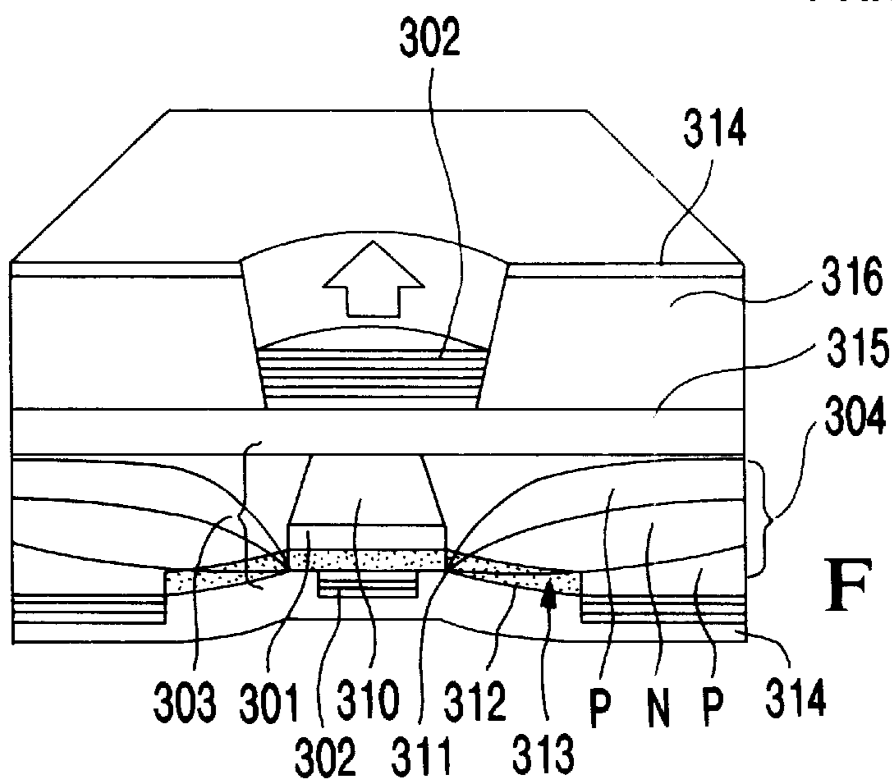
FIG. 30B PRIOR ART
