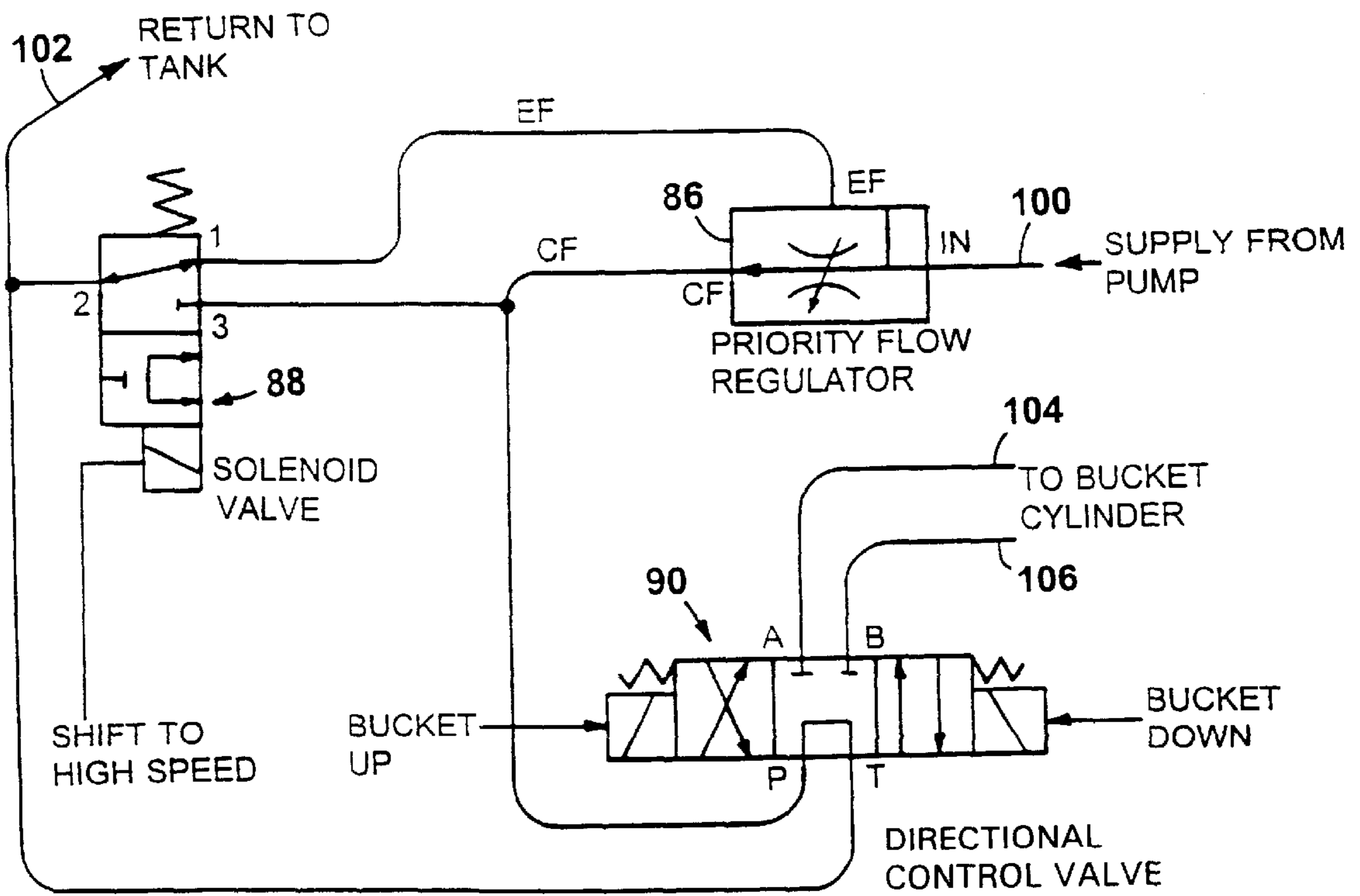
JETSTICK BUCKET HYDRAULIC CONTROL
