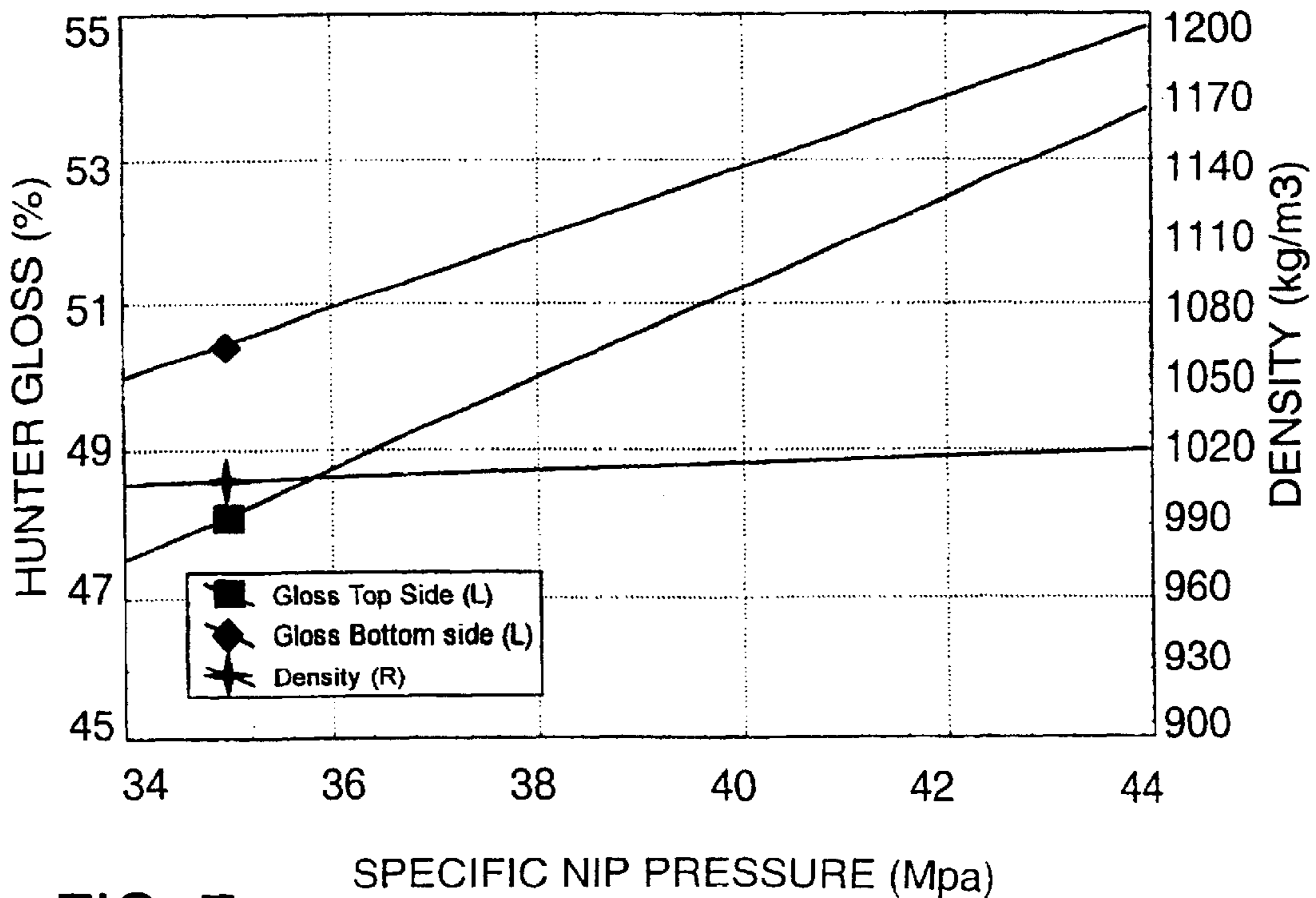
FIG. 7 SPECIFIC NIP PRESSURE (Mpa)
