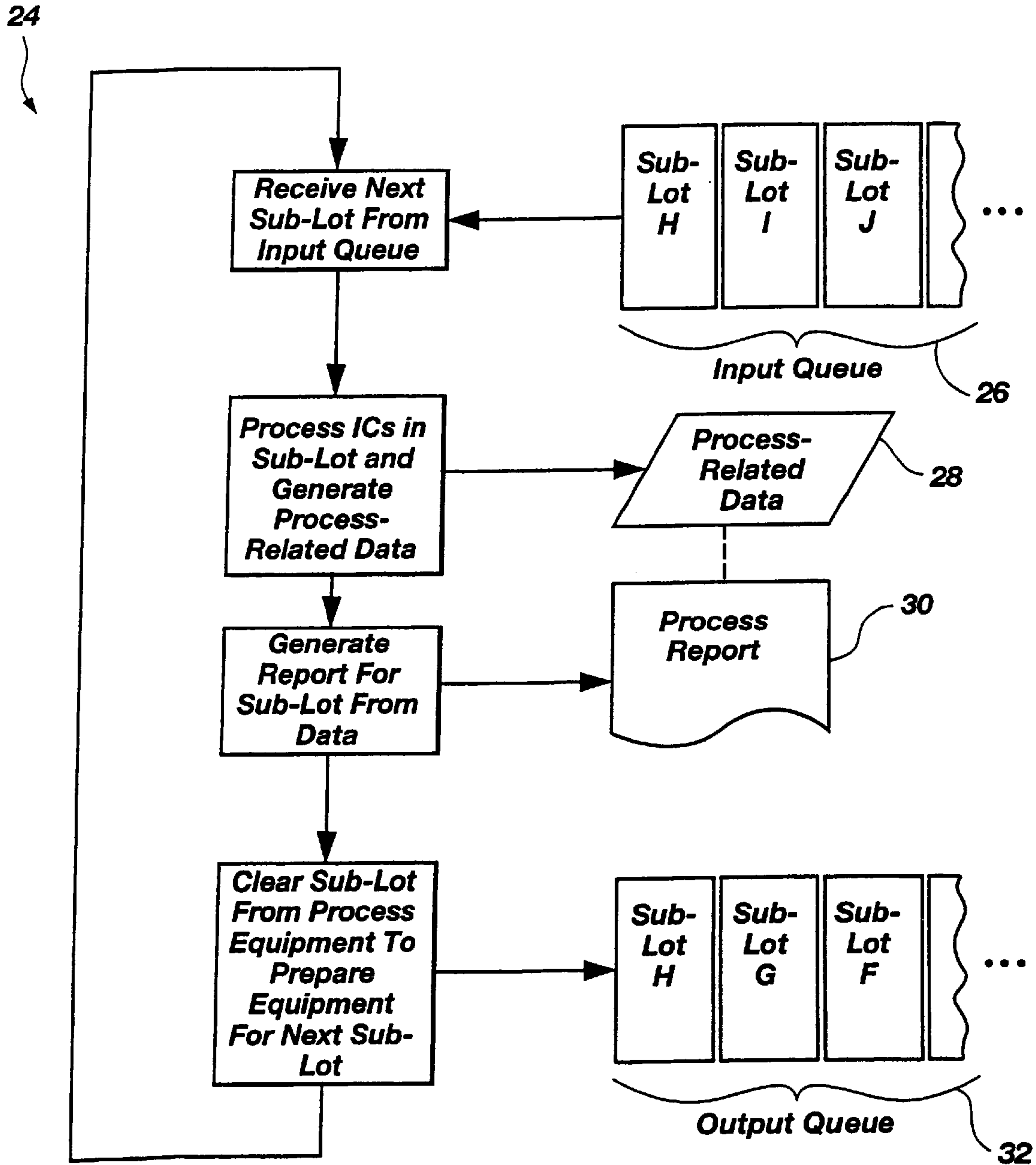
Fig. 3 (PRIOR ART)
