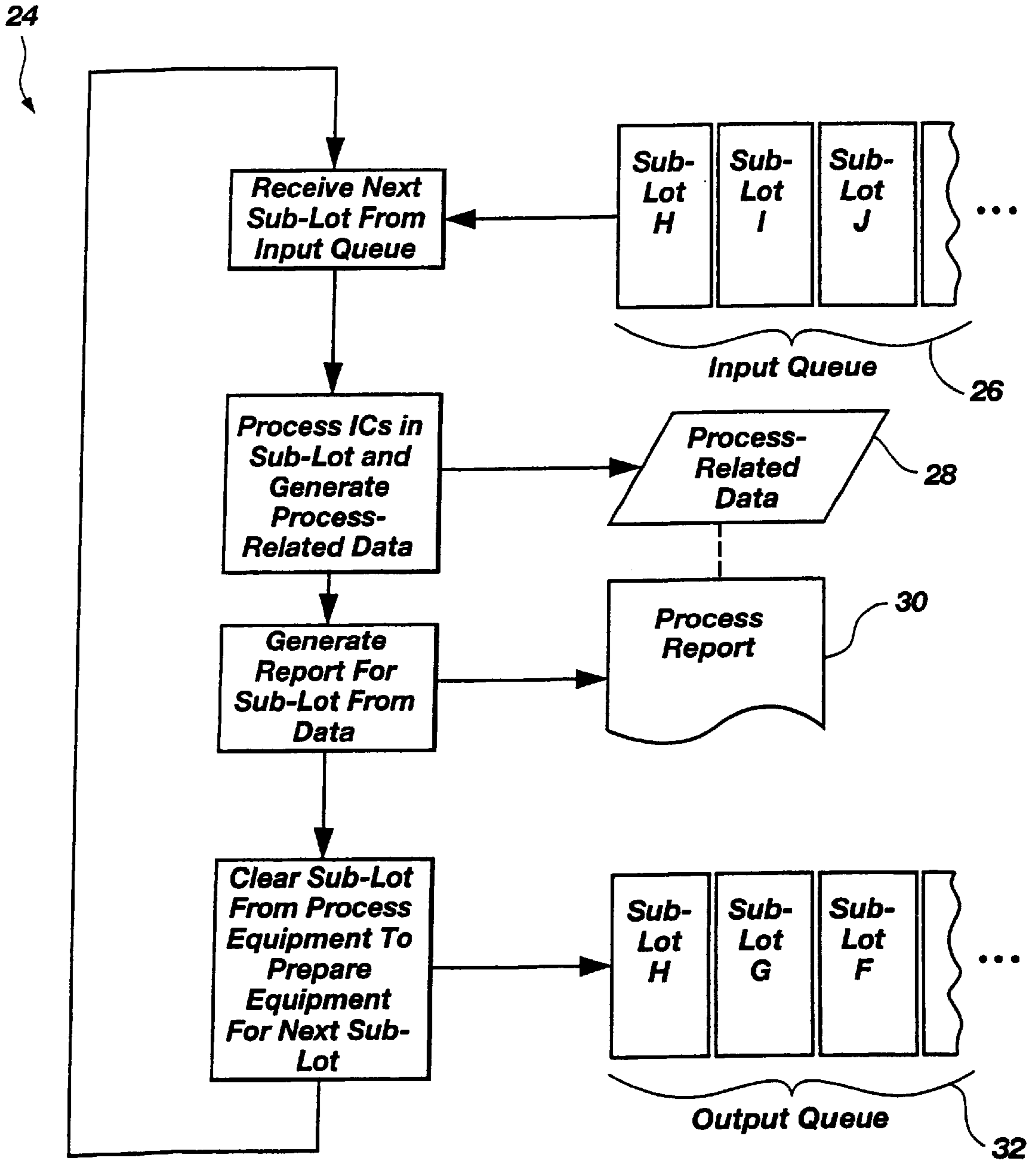
Fig. 3 (PRIOR ART)
