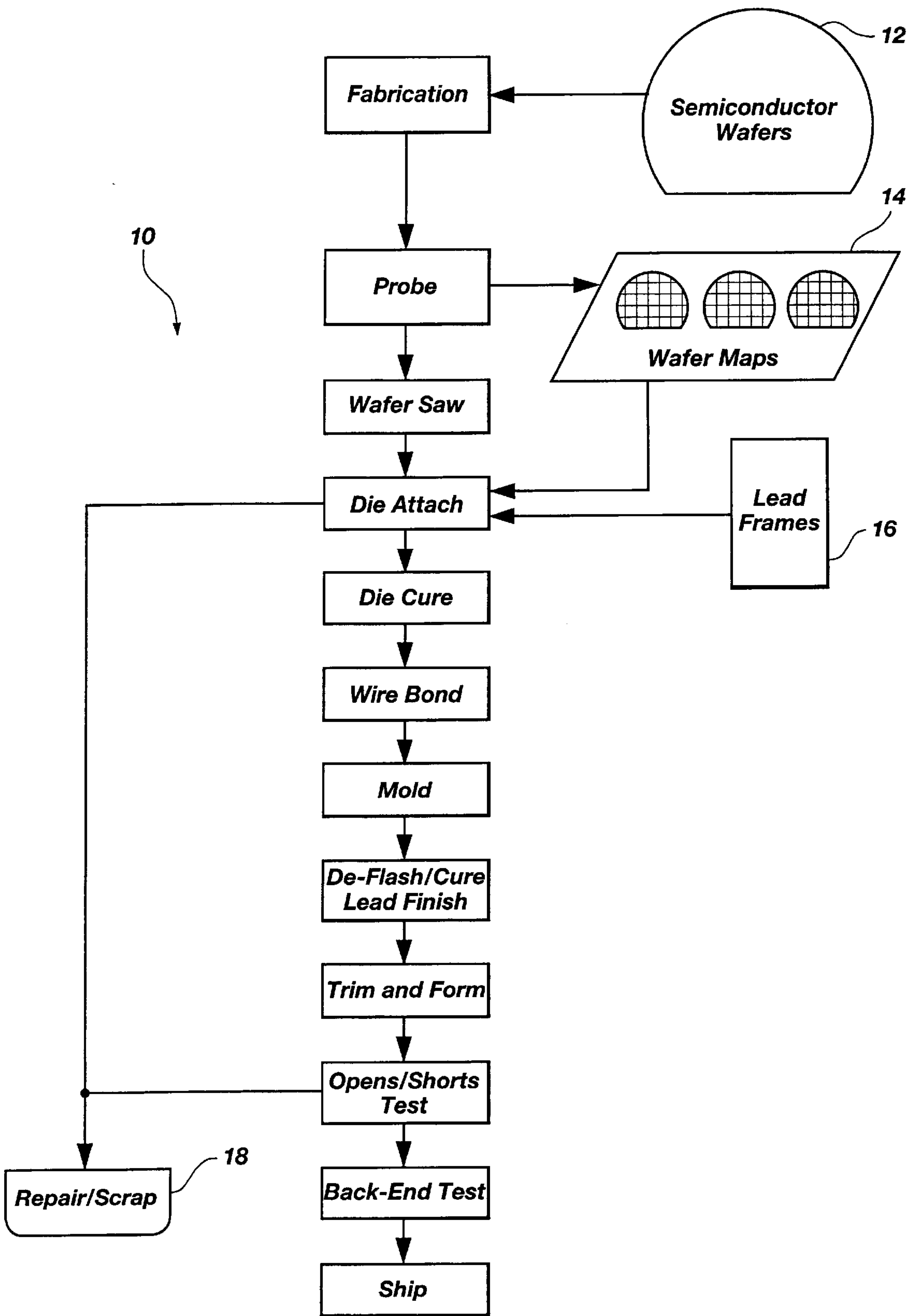
Fig. 1 (PRIOR ART)
