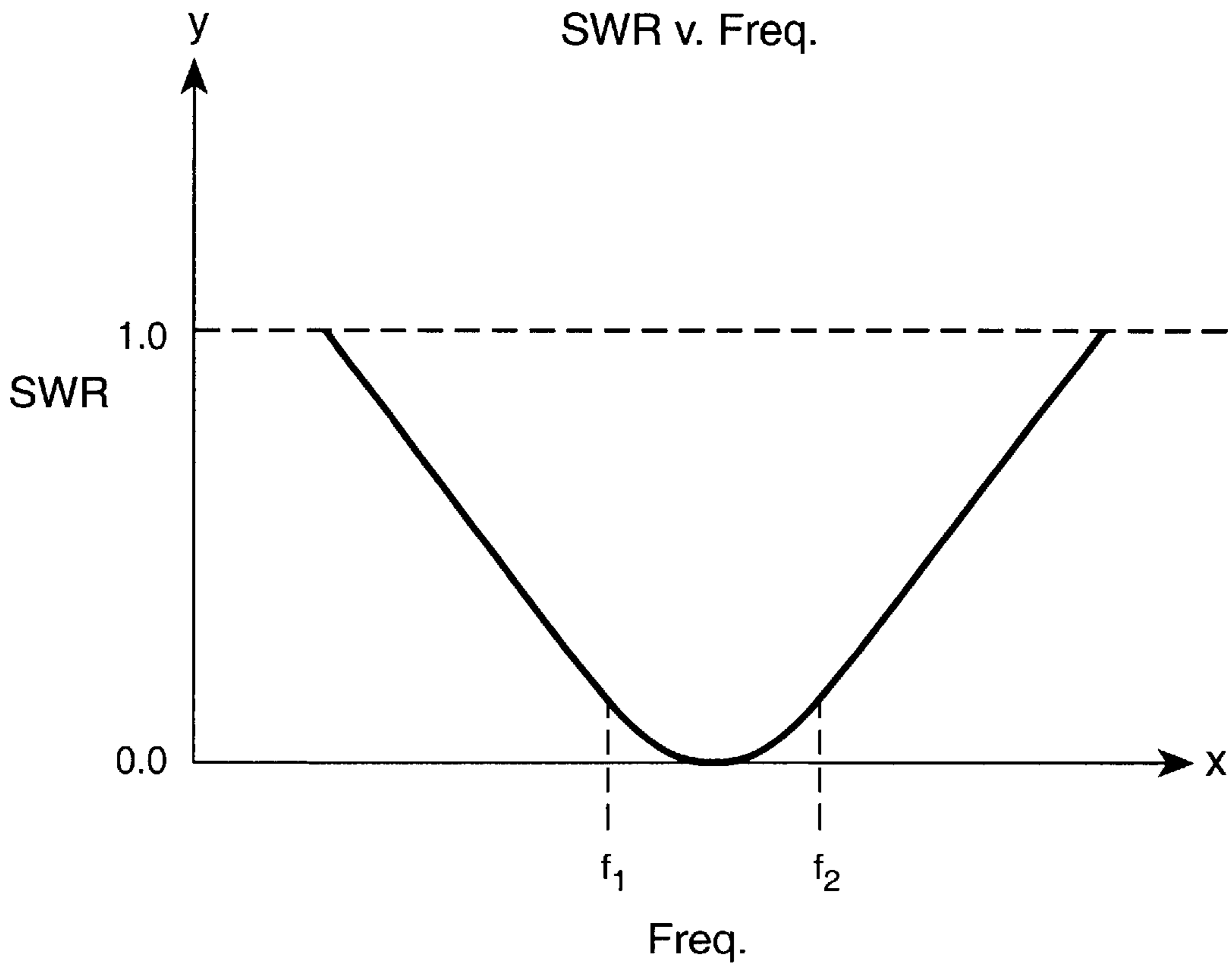
FIG. 2 (PRIOR ART)
