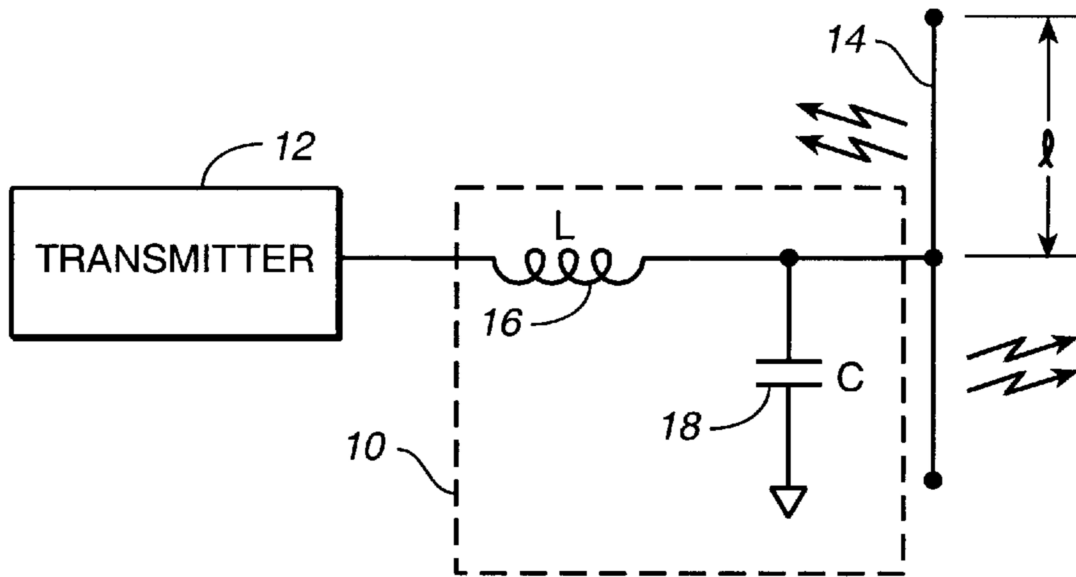
FIG. 1 (PRIOR ART)
