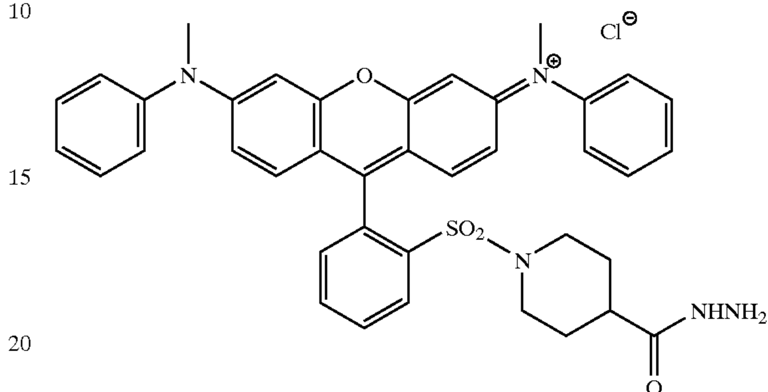
Compound 30
