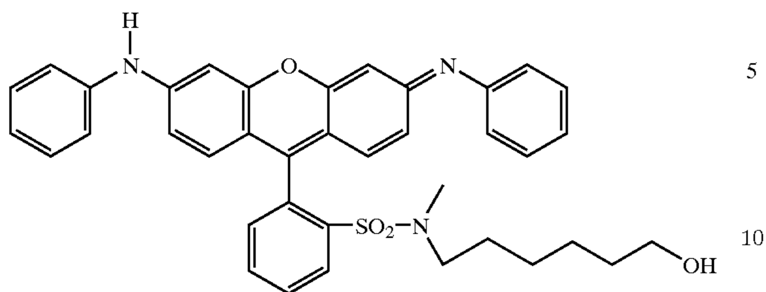
Compound 28
