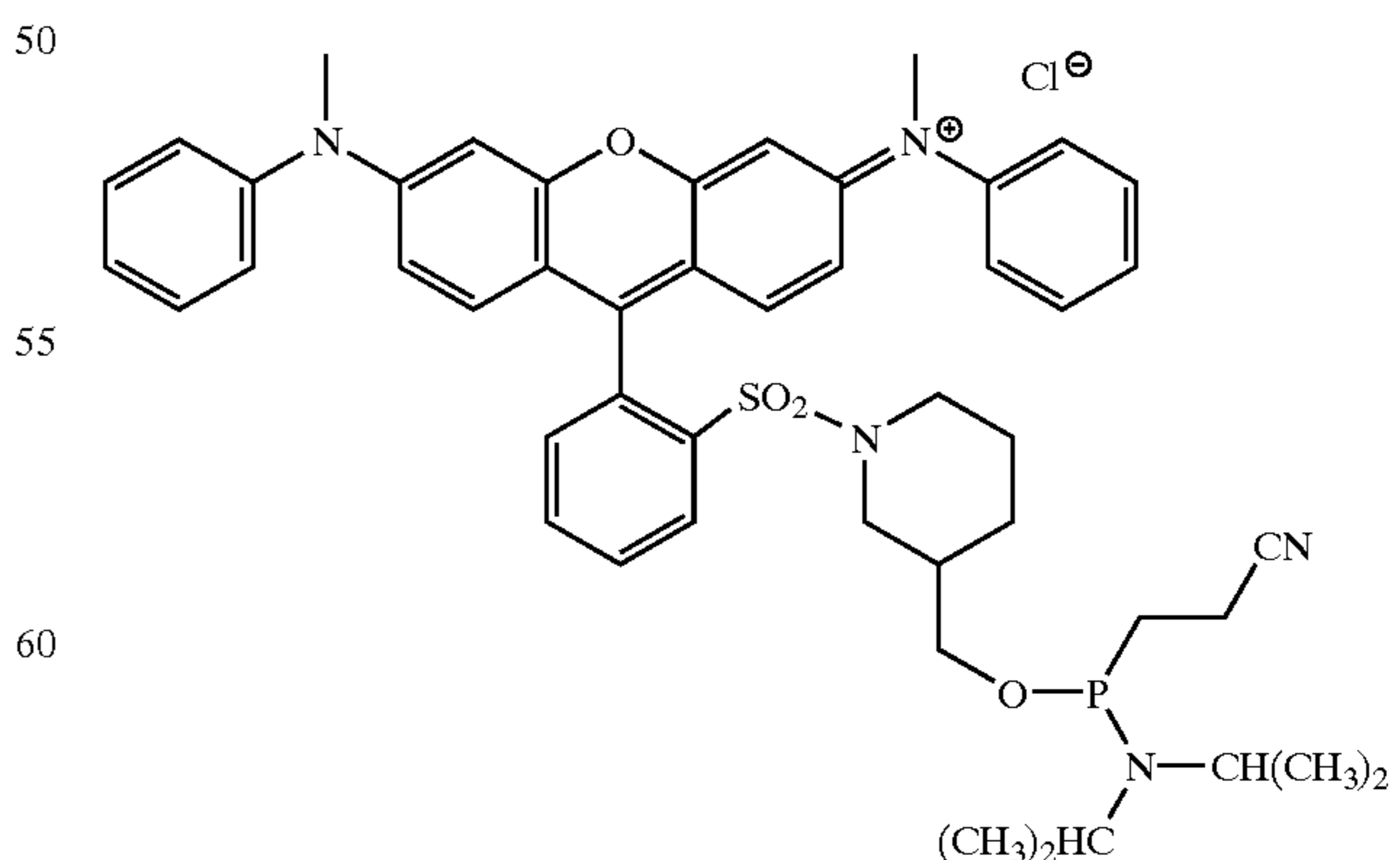
Compound 3
