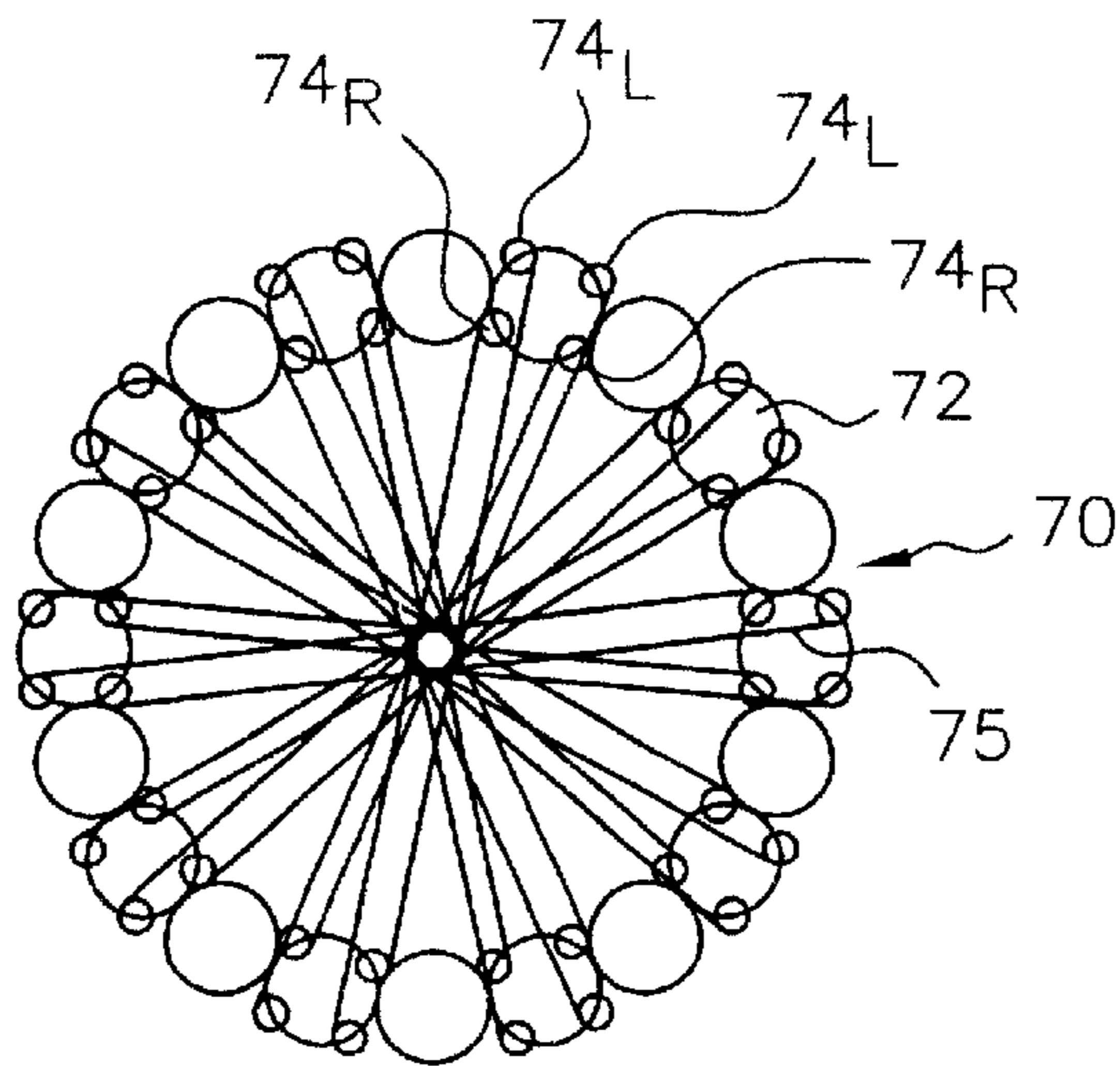
FIG. 16 (Prior Art)
