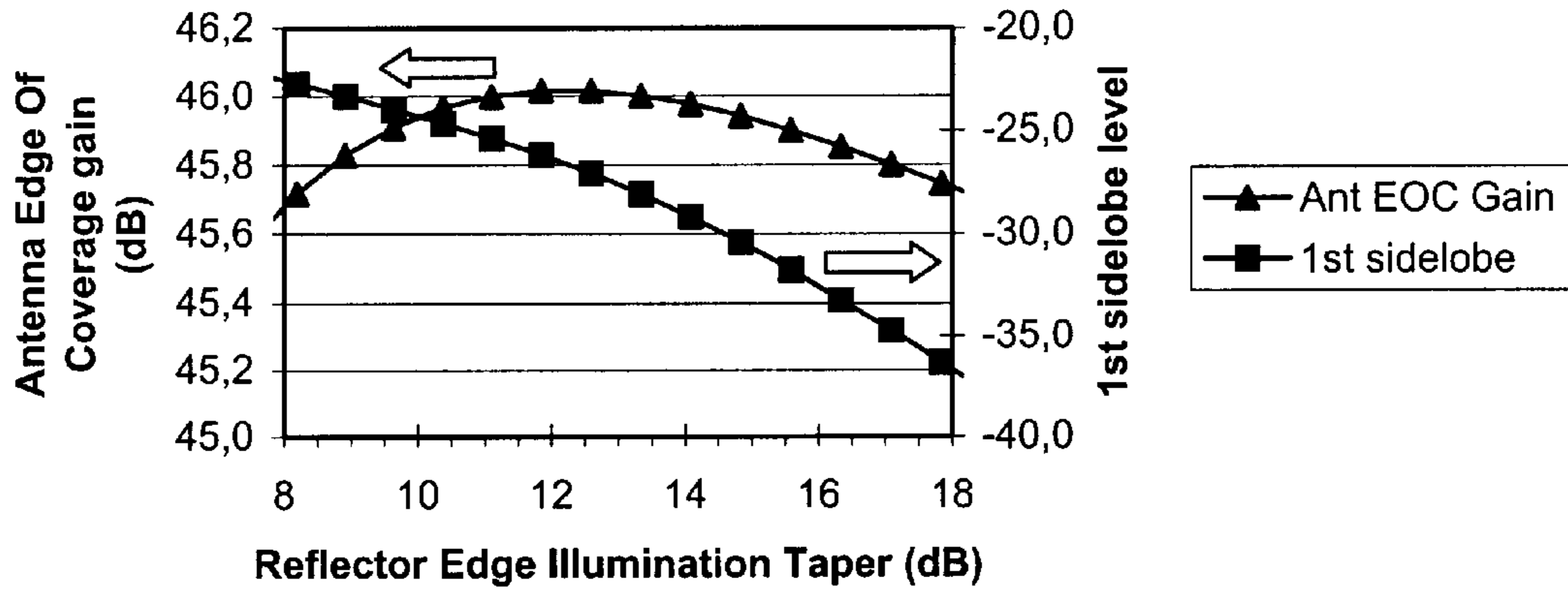
MBA performance vs Edge Taper (0.60-deg spacing; -4 dB crossover)
