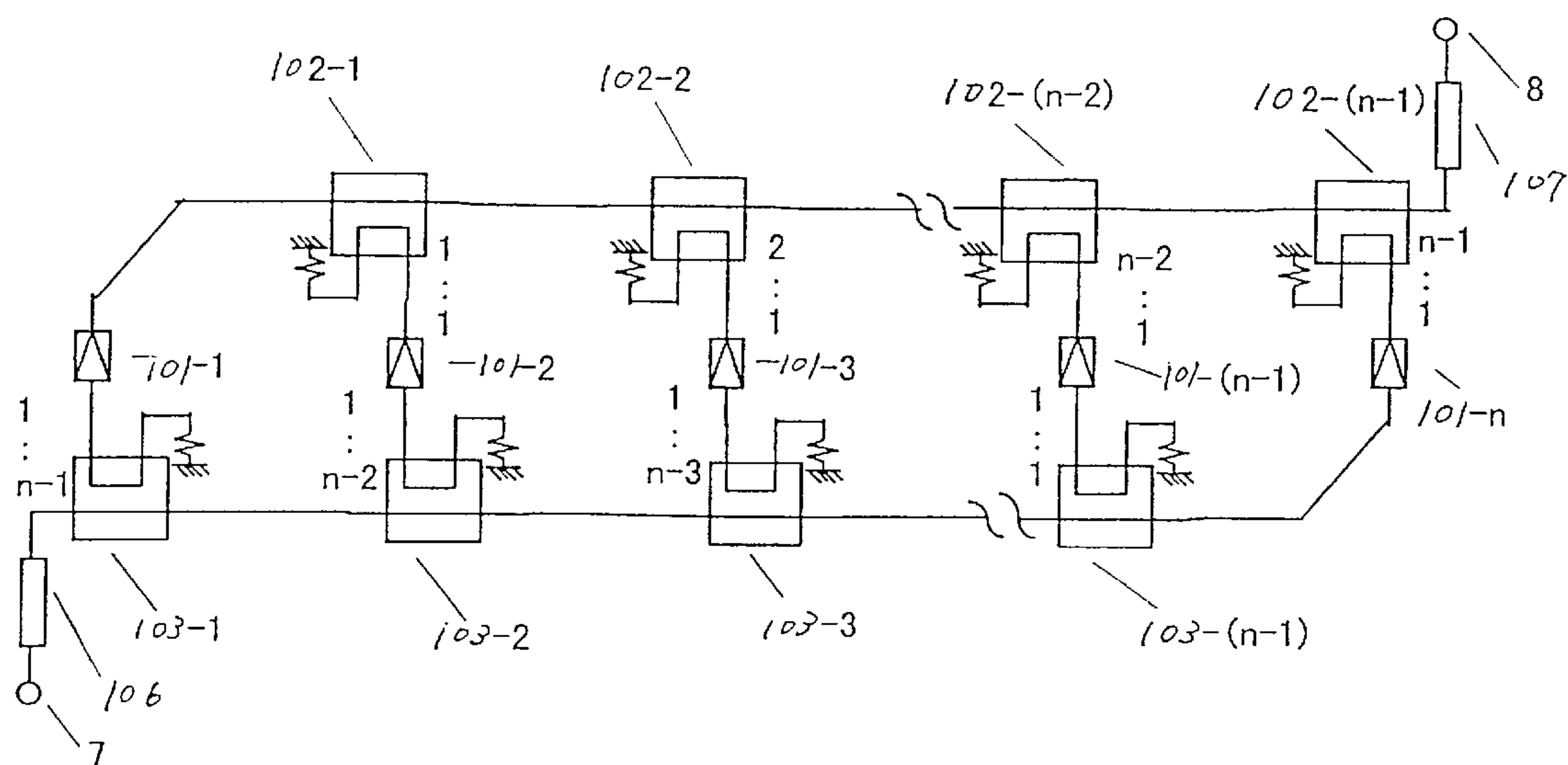
FIG. 18 (PRIOR ART)
