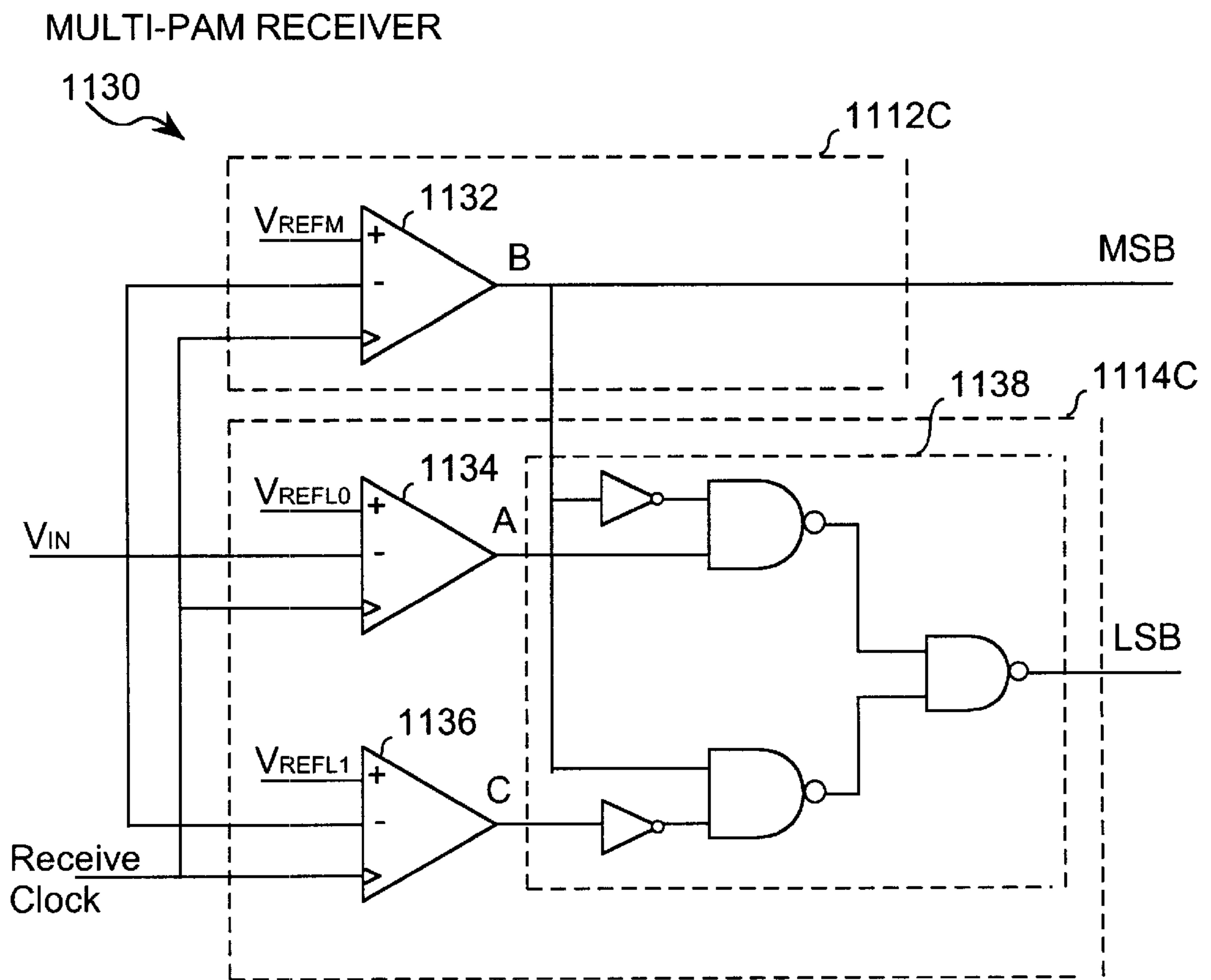
Multi-PAM Receiver FIG. 43
