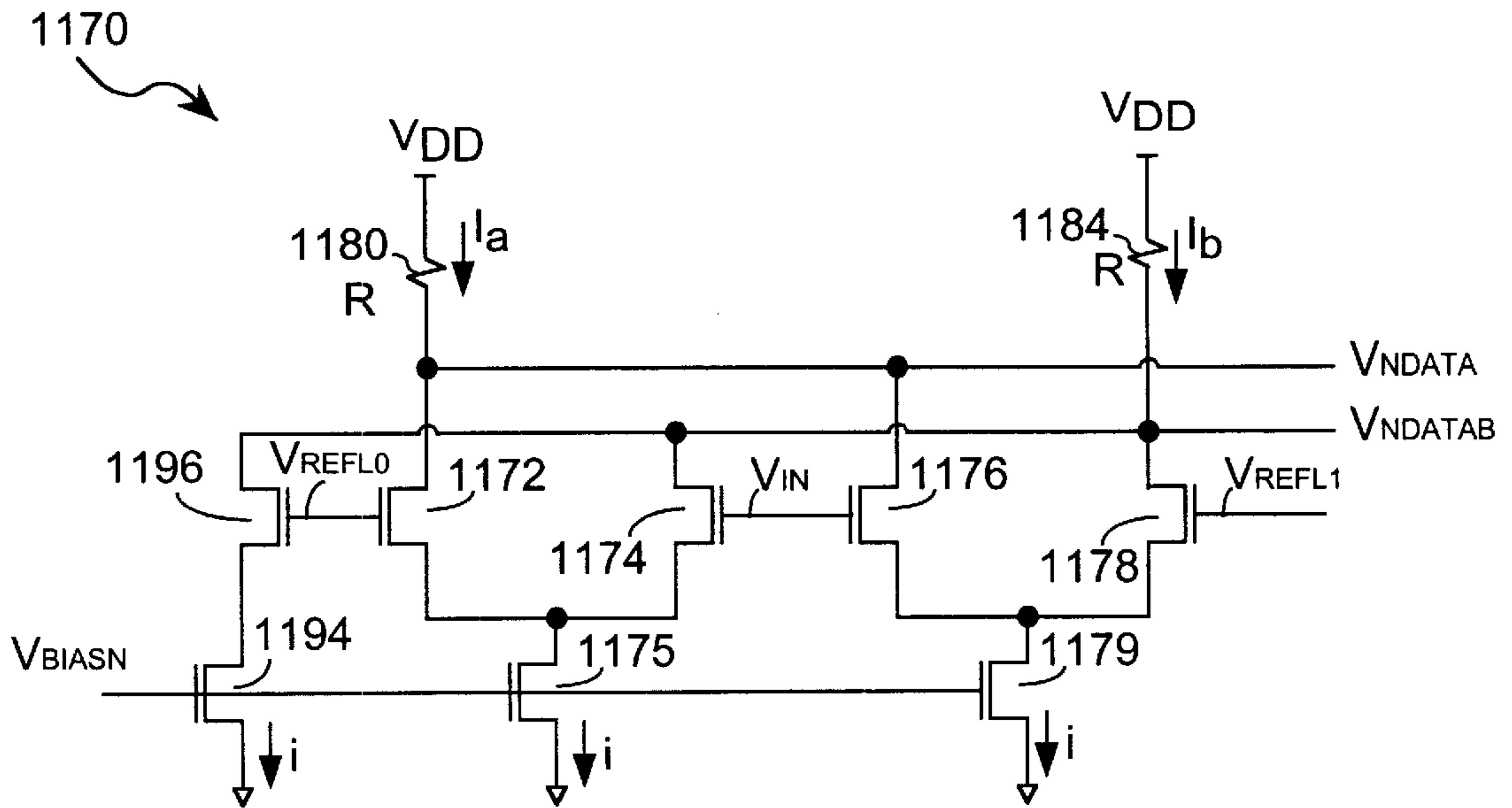
Multi-PAM Pre-Amplifier FIG. 45A
