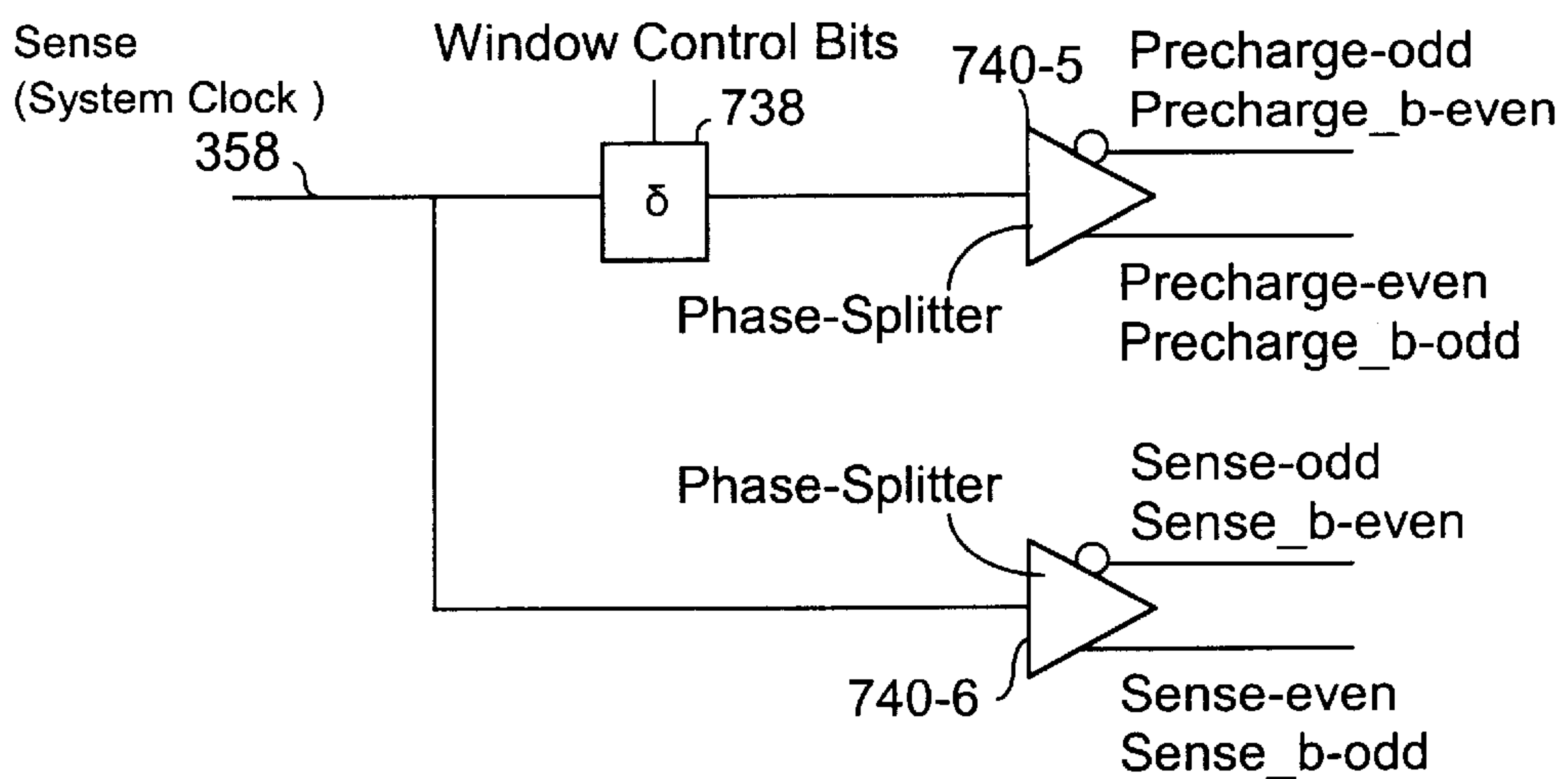
Circuit for Timing Diagram of Fig.17C
