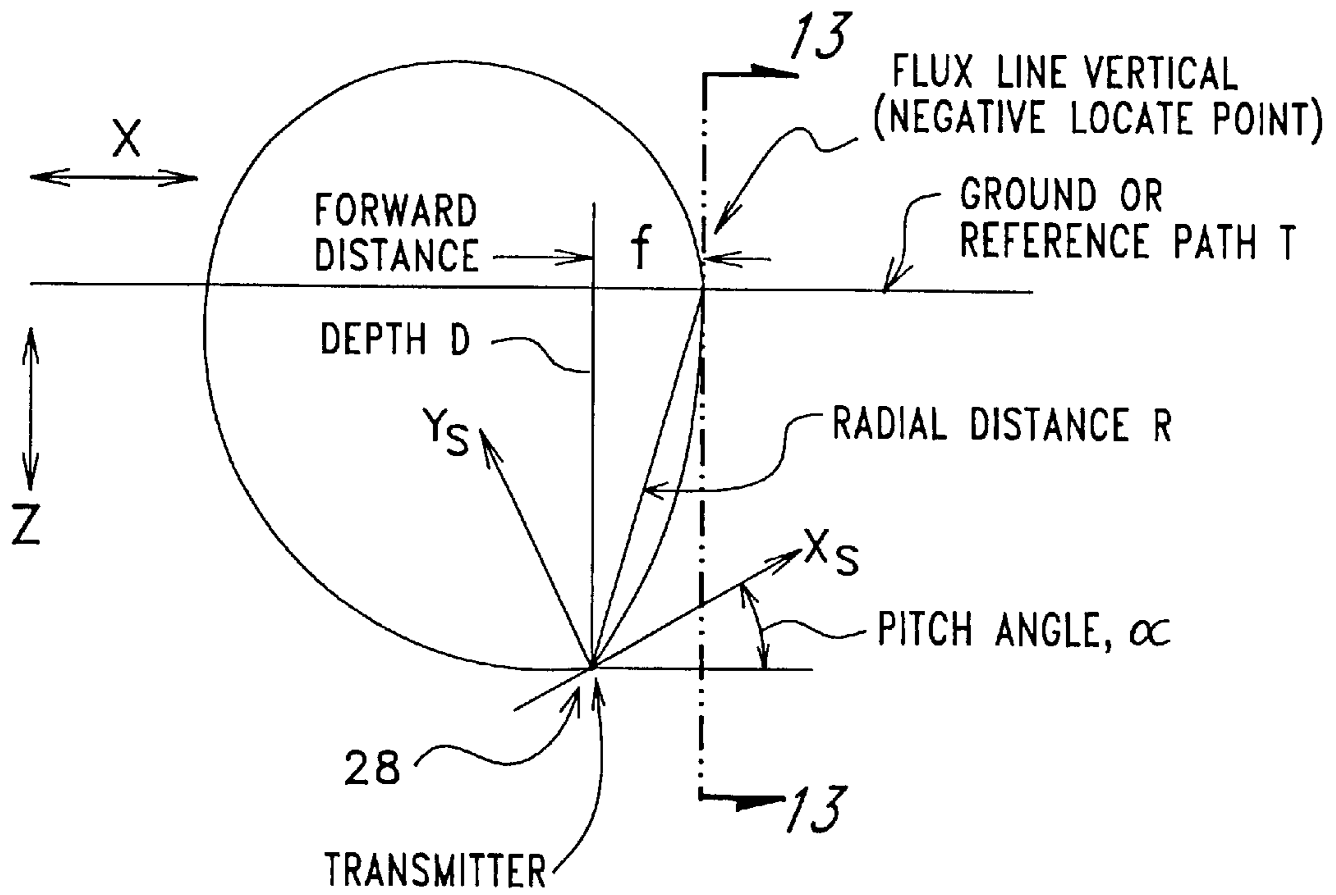
SIDE VIEW FIG. 12
