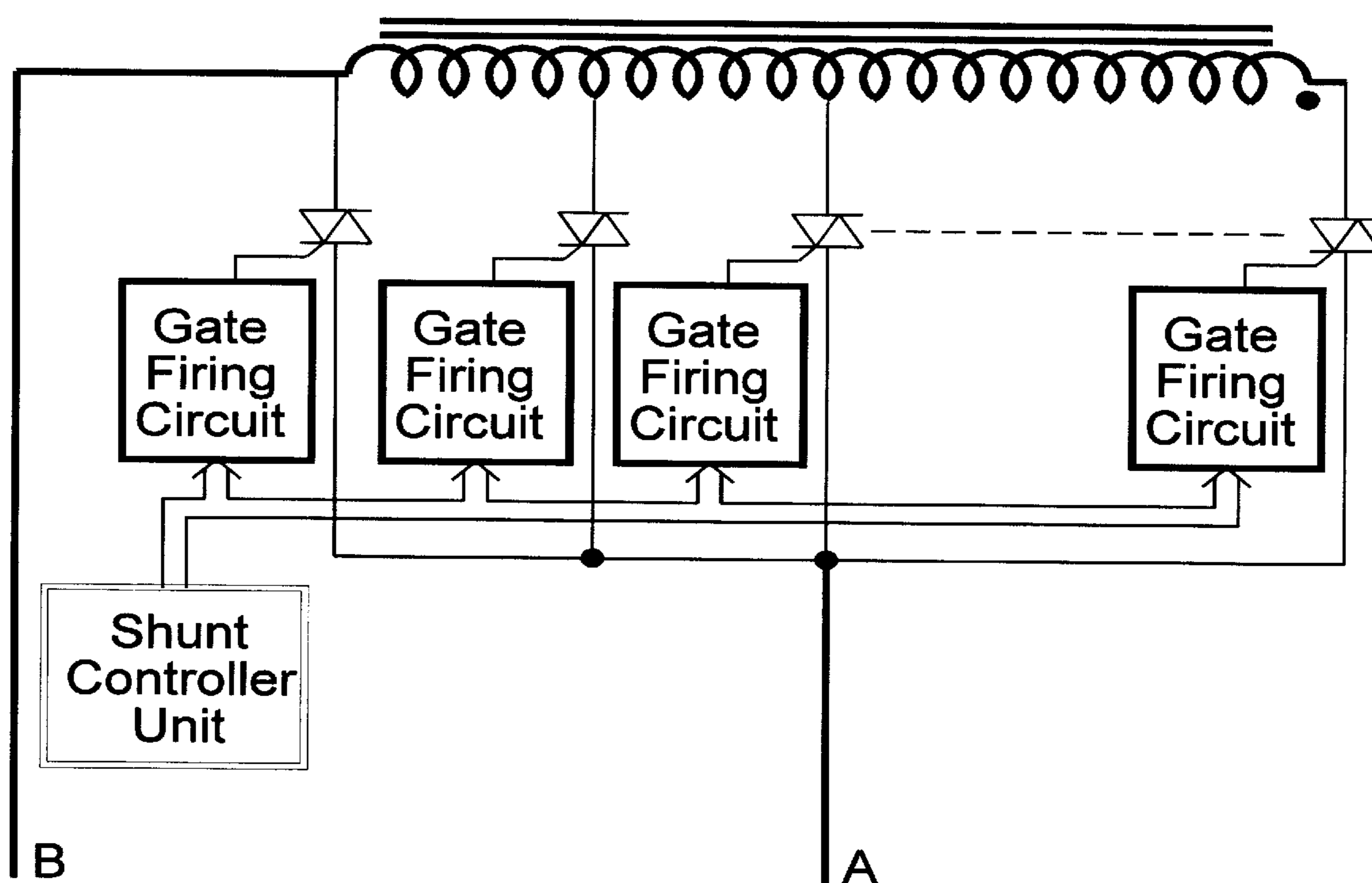
FIG. 3 – PRIOR ART
