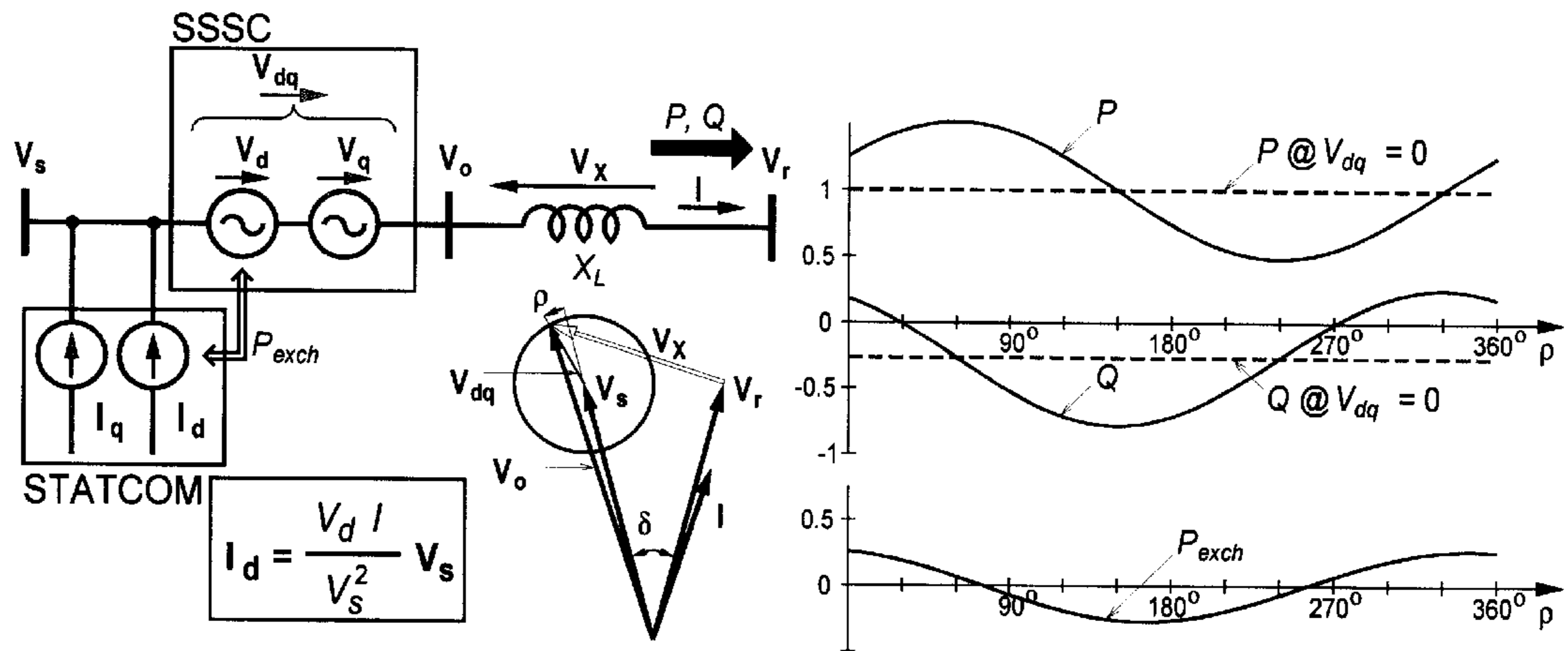
FIG. 13 – PRIOR ART
