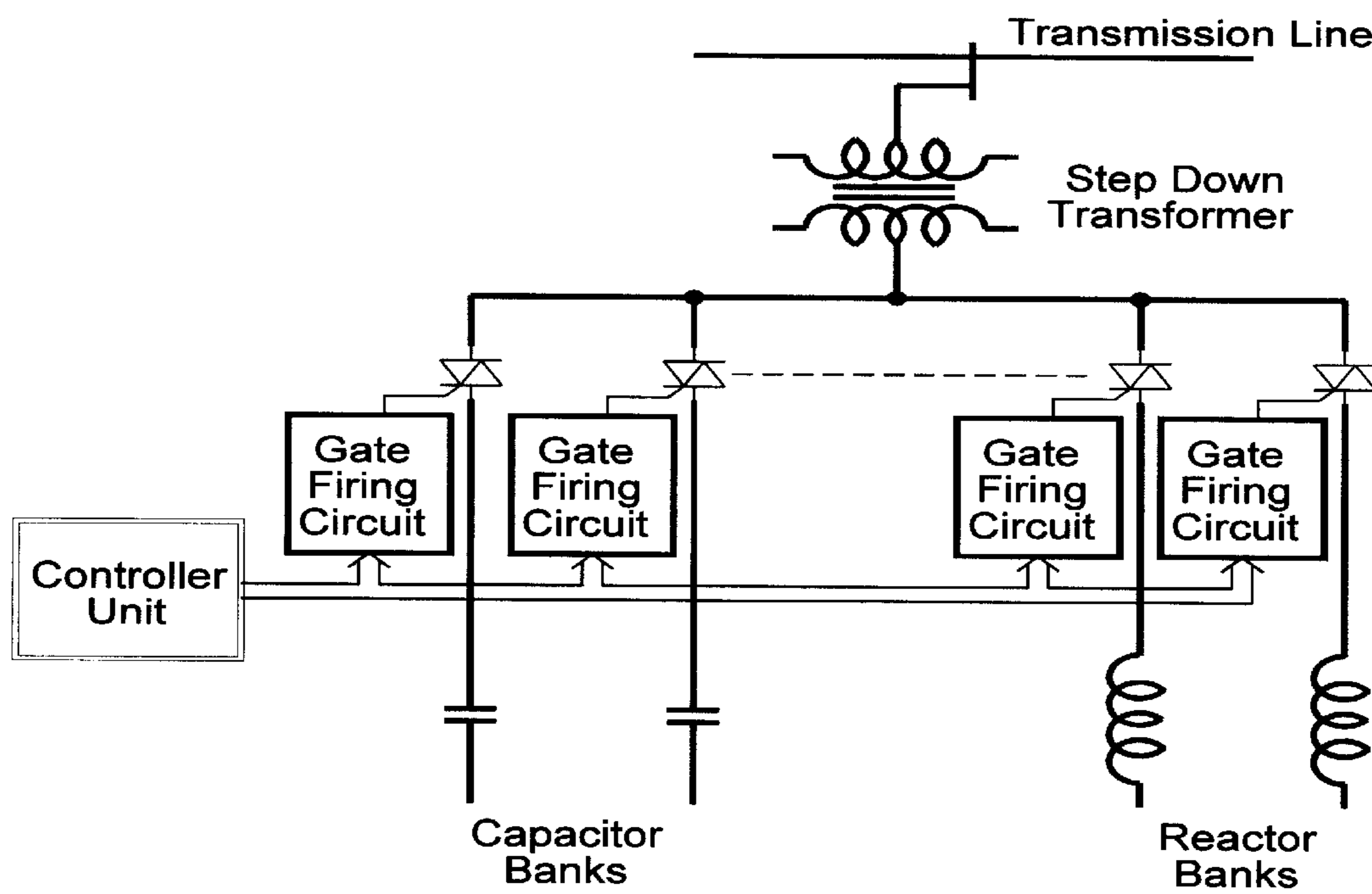
FIG. 4 – PRIOR ART
