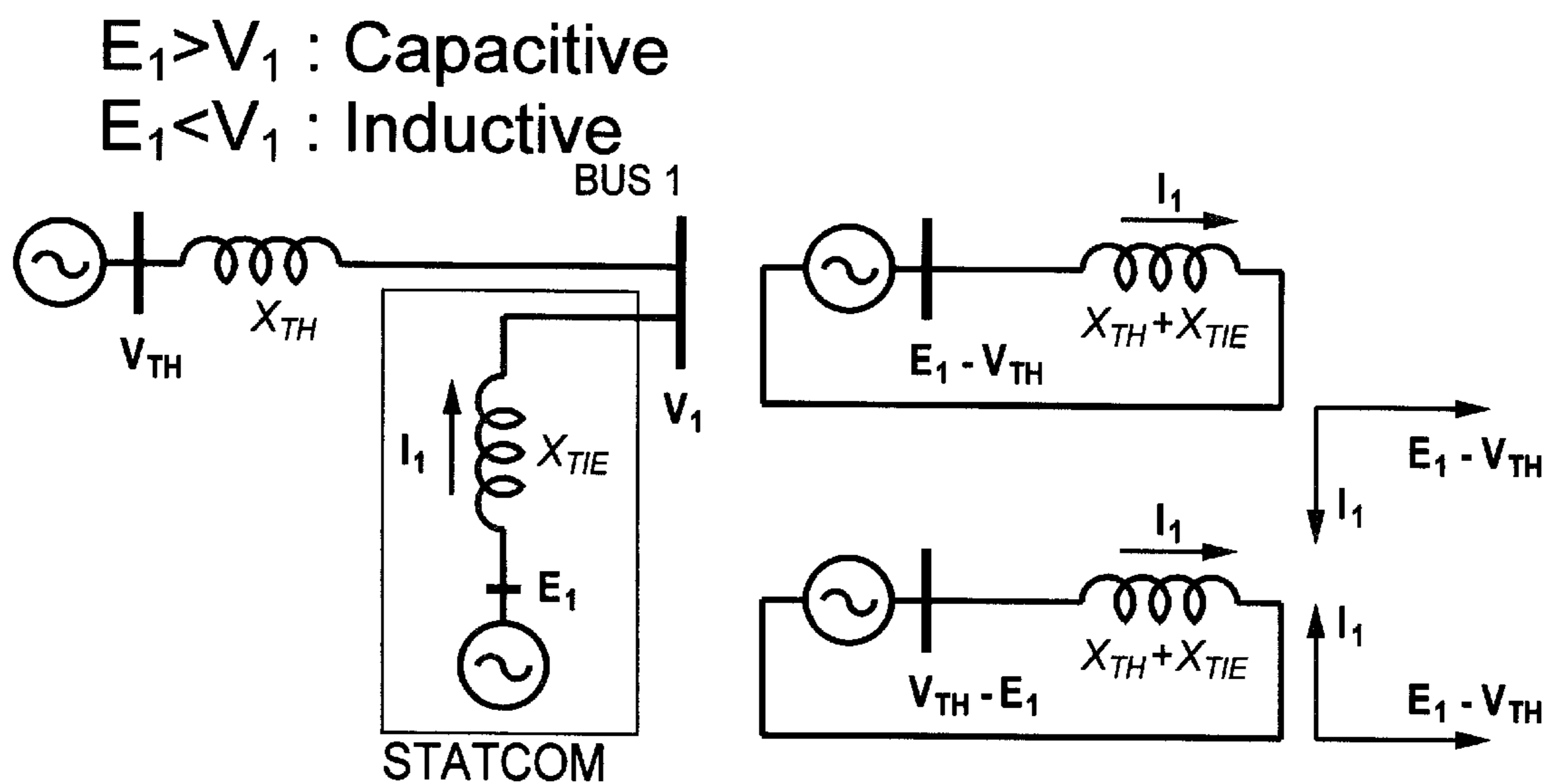
FIG. 6 – PRIOR ART
