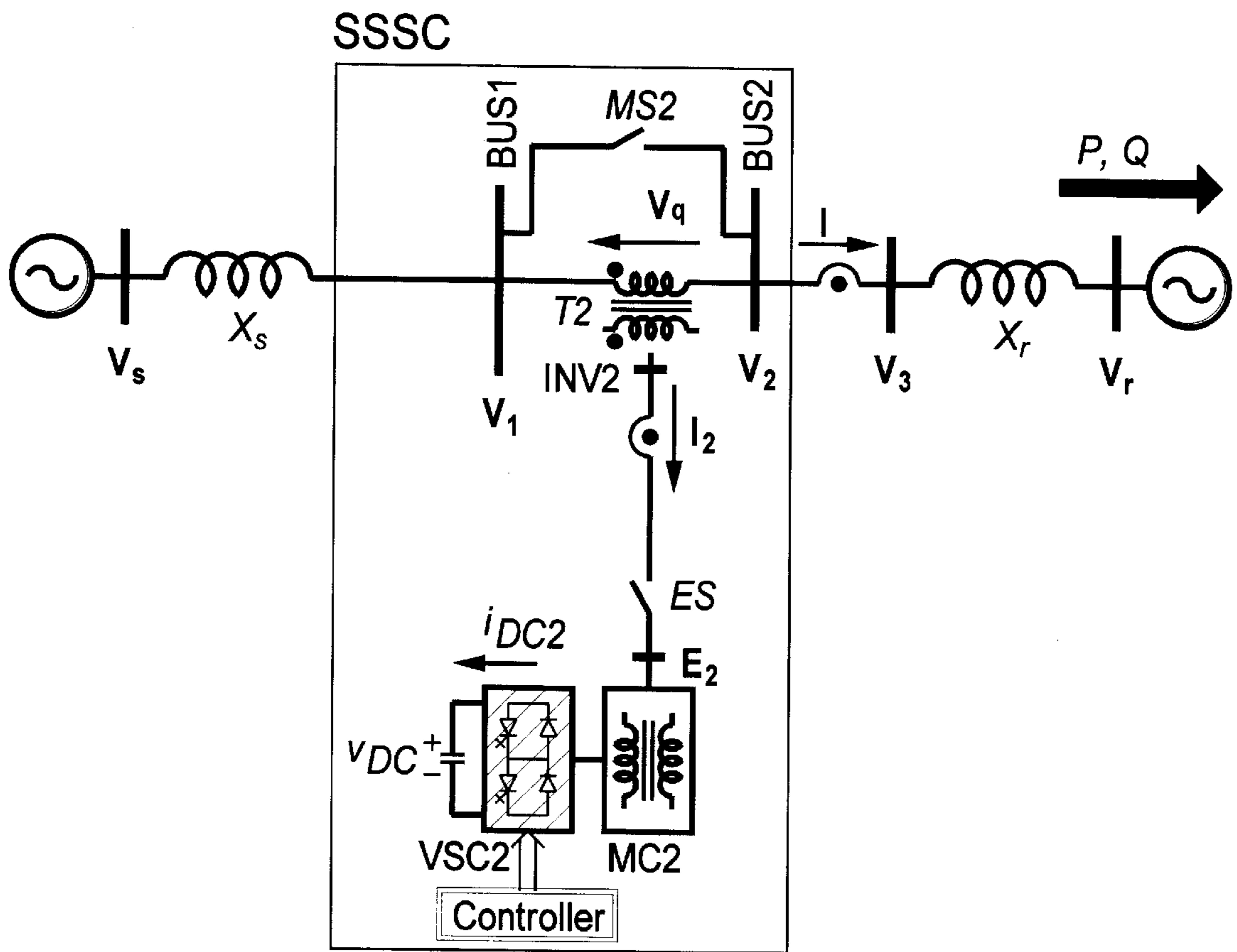
FIG. 8 – PRIOR ART
