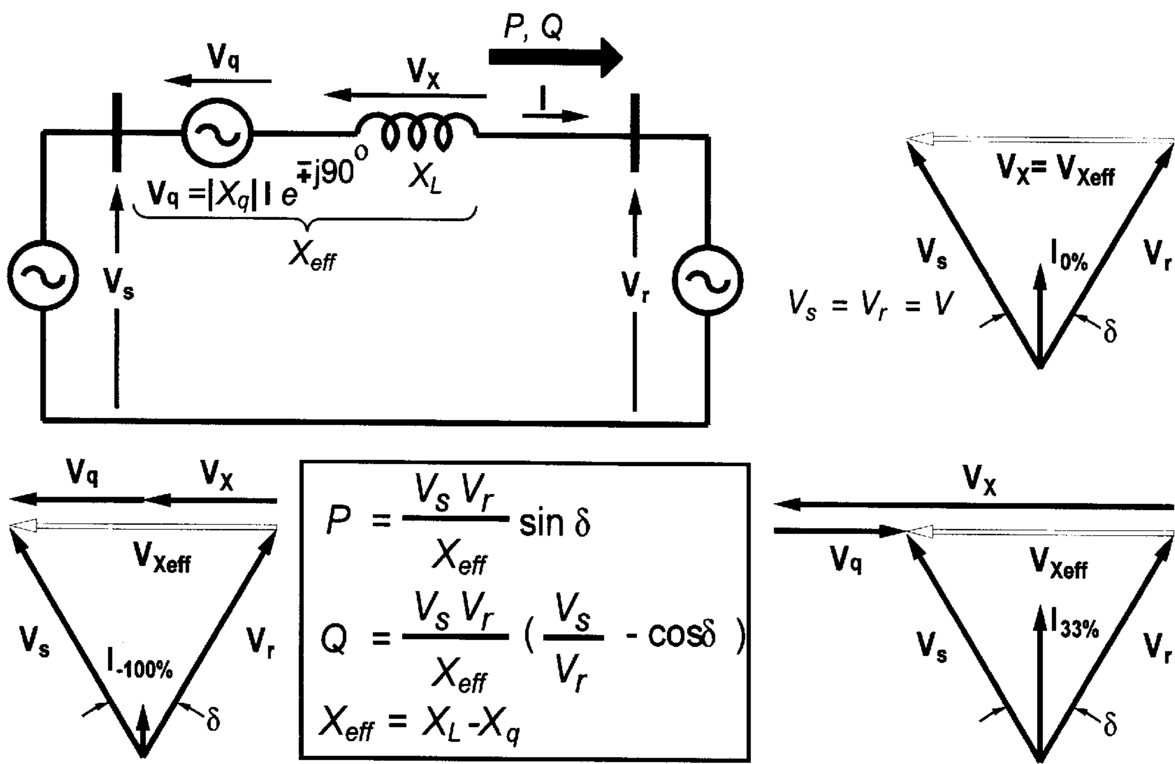
FIG. 9 – PRIOR ART
