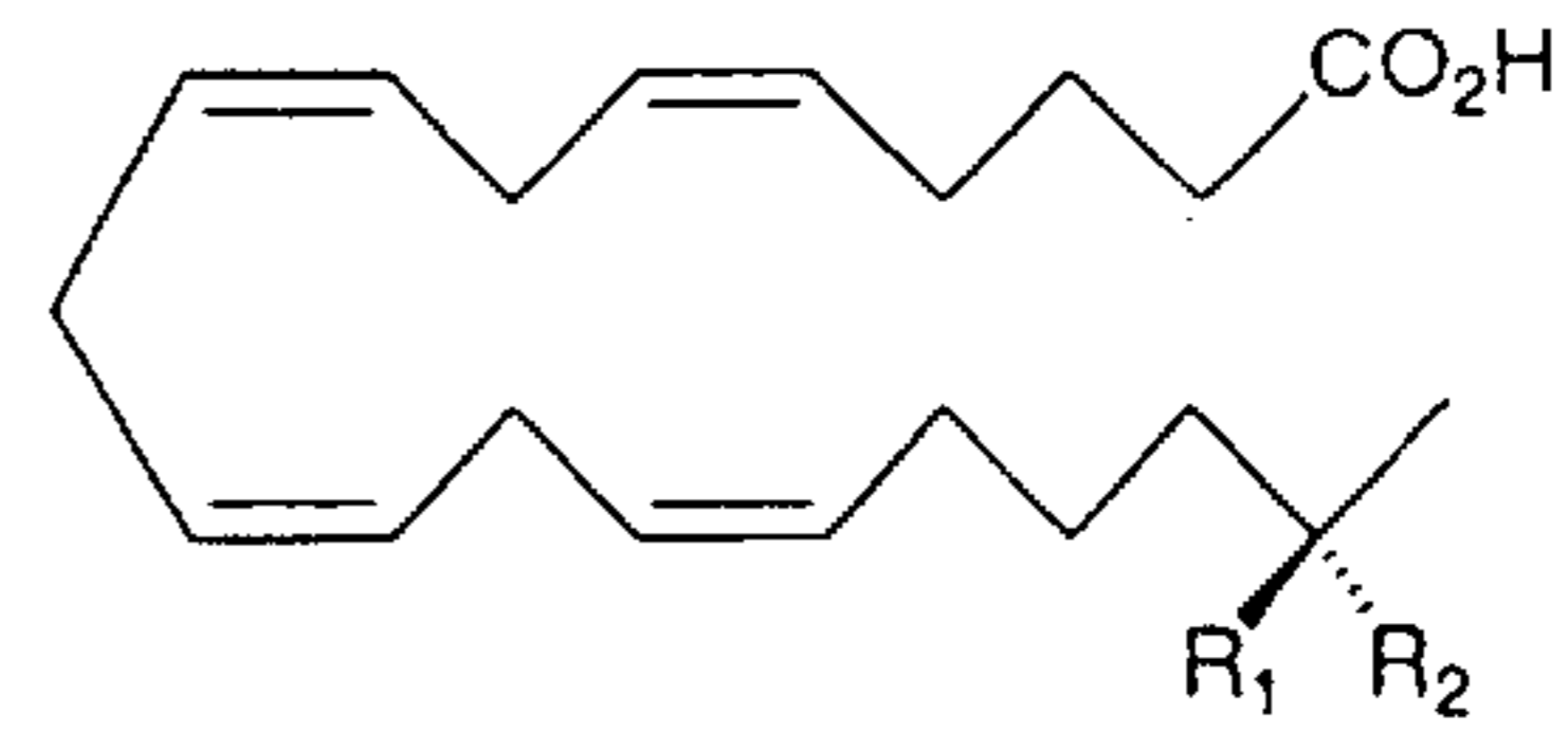
19(S)-HETE (34: R 1 = H, R 2 = OH)
