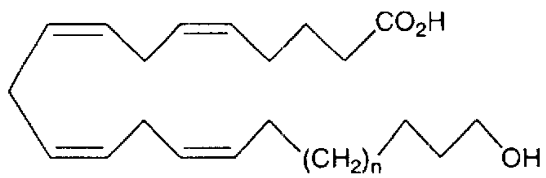
19-Hydroxynonadeca-5(Z),8(Z),11(Z),14(Z)-tetraenoic Acid (9a: n = 0)
