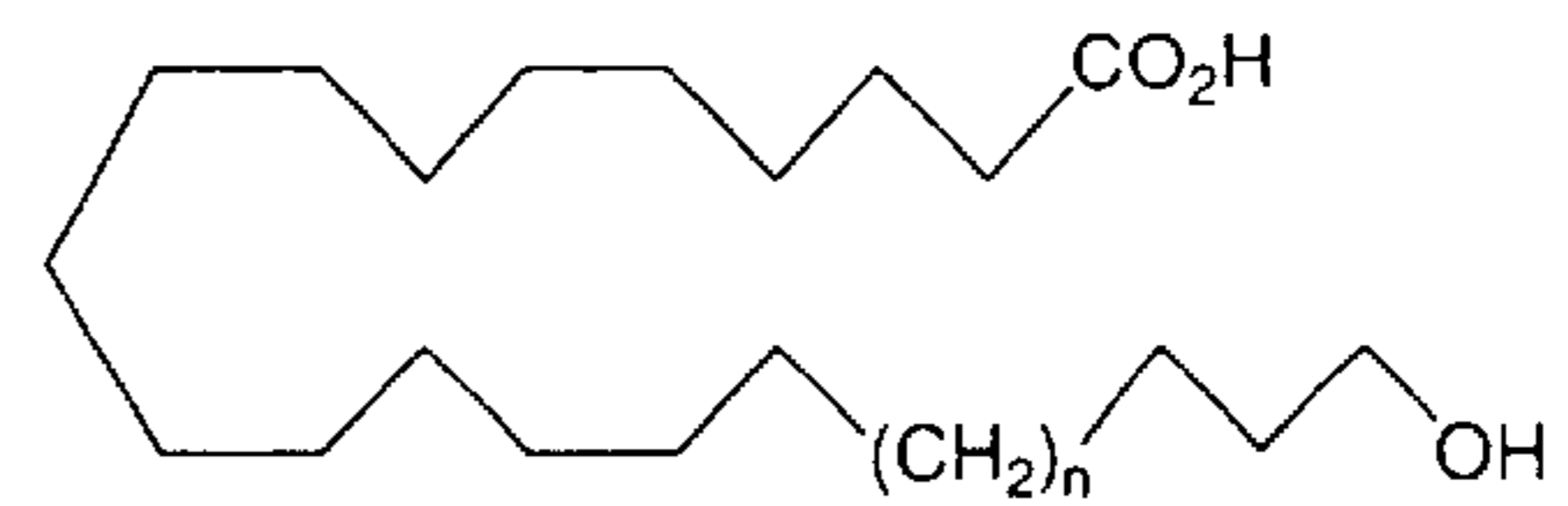
20-Hydroxyeicosanoic Acid (55: n = 1) 19-Hydroxynonadecanoic Acid (56: n = 0)
