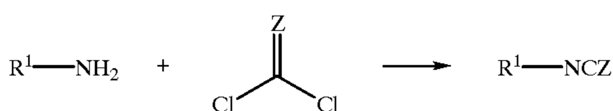
SCHEME II
