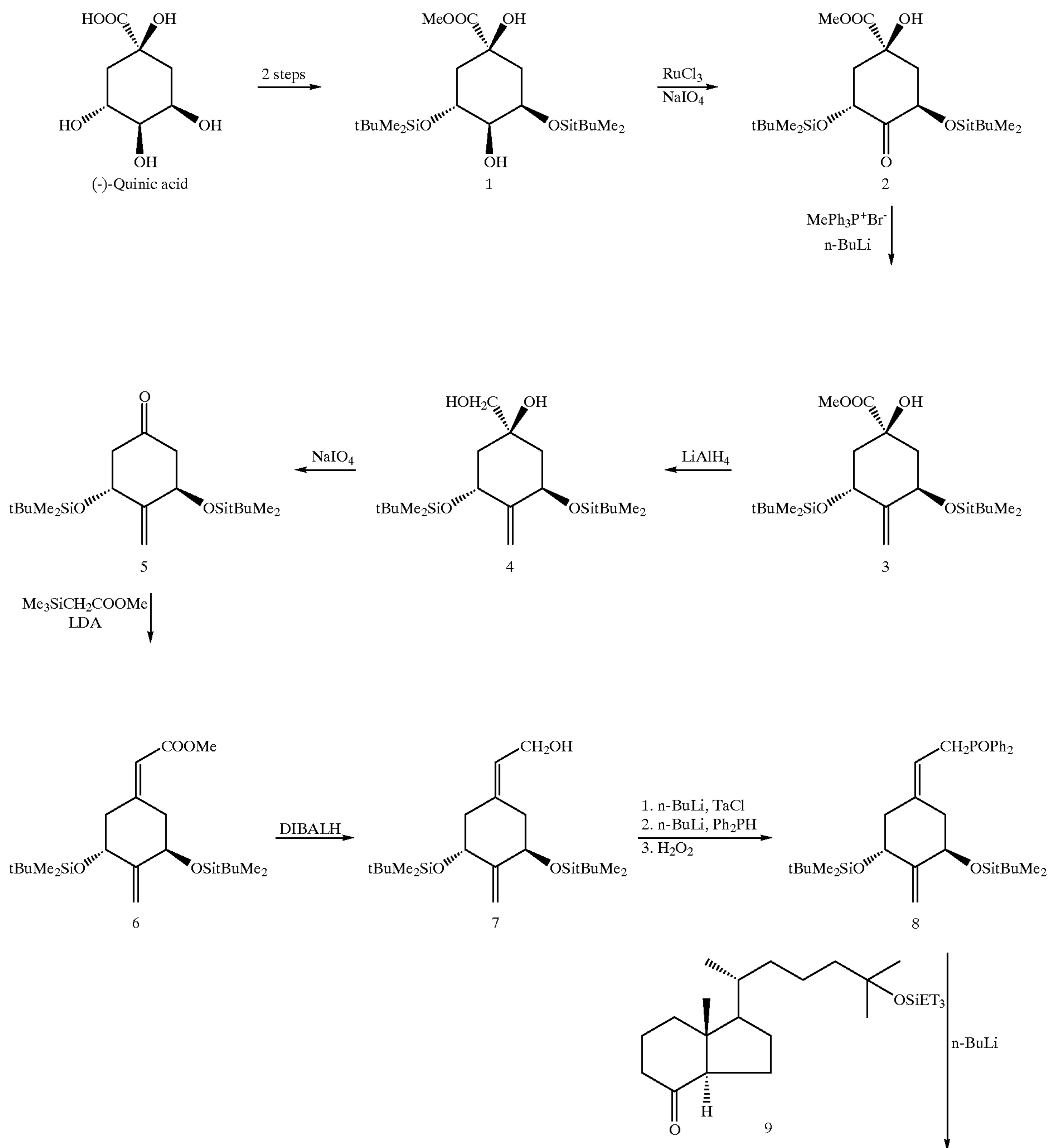
SCHEME I
