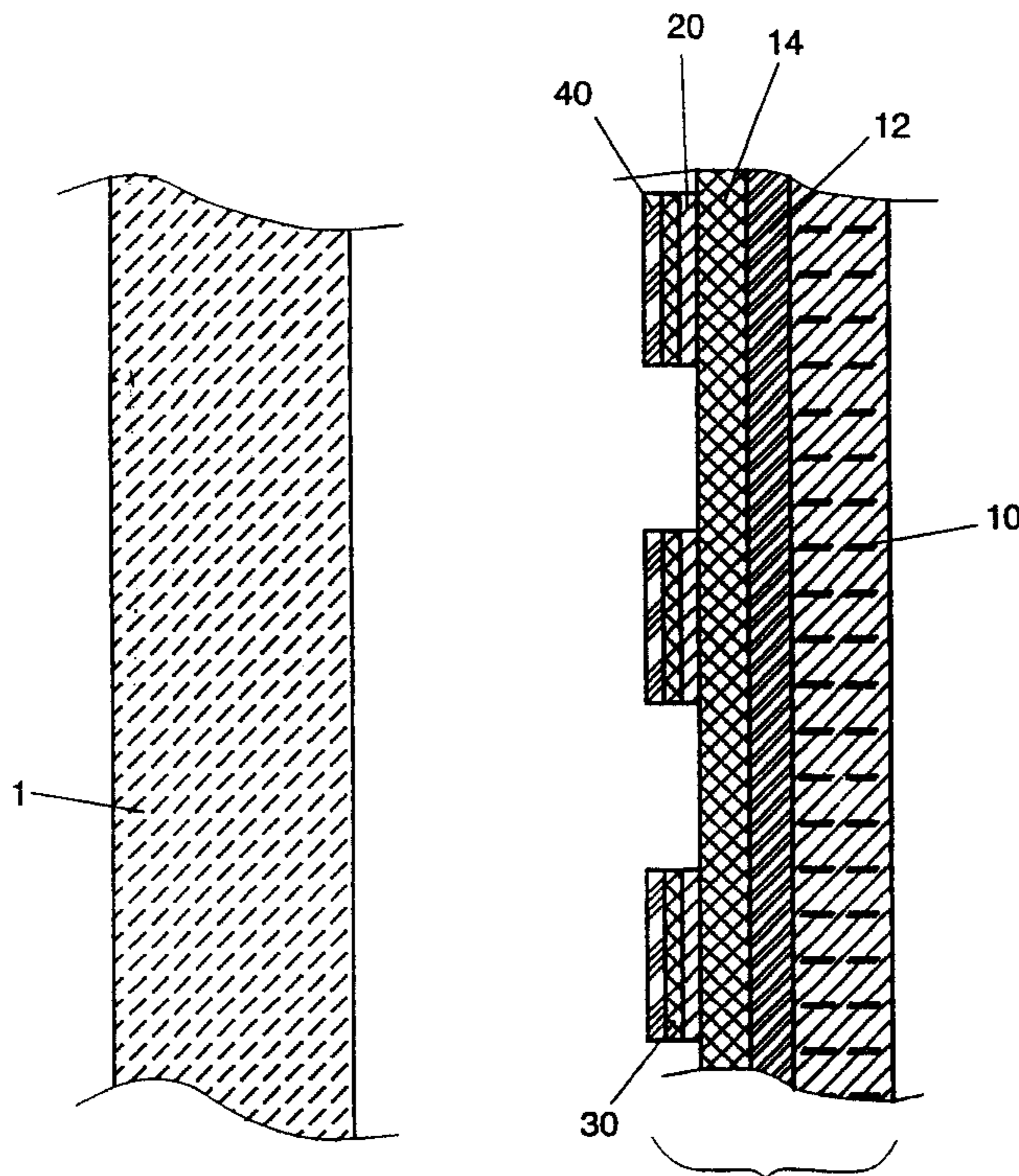
LABEL & SUBSTRATE EXPLODED VIEW
