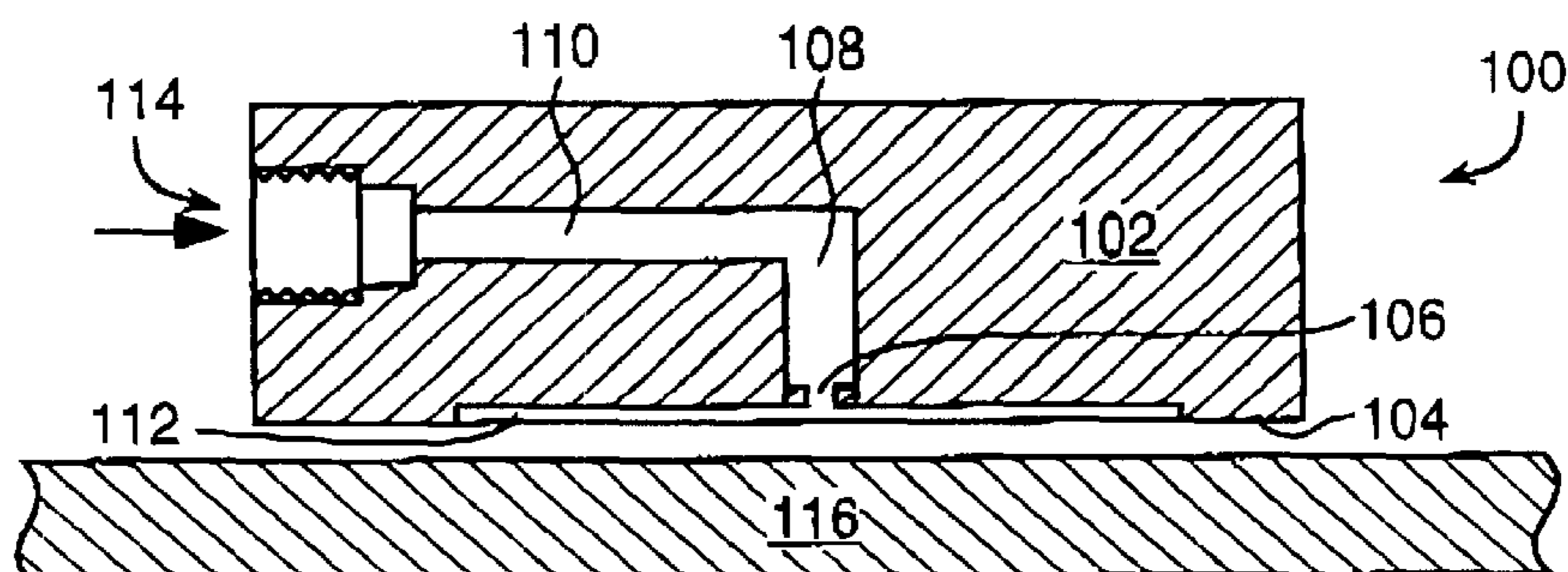
FIG. 1 (Prior Art)
