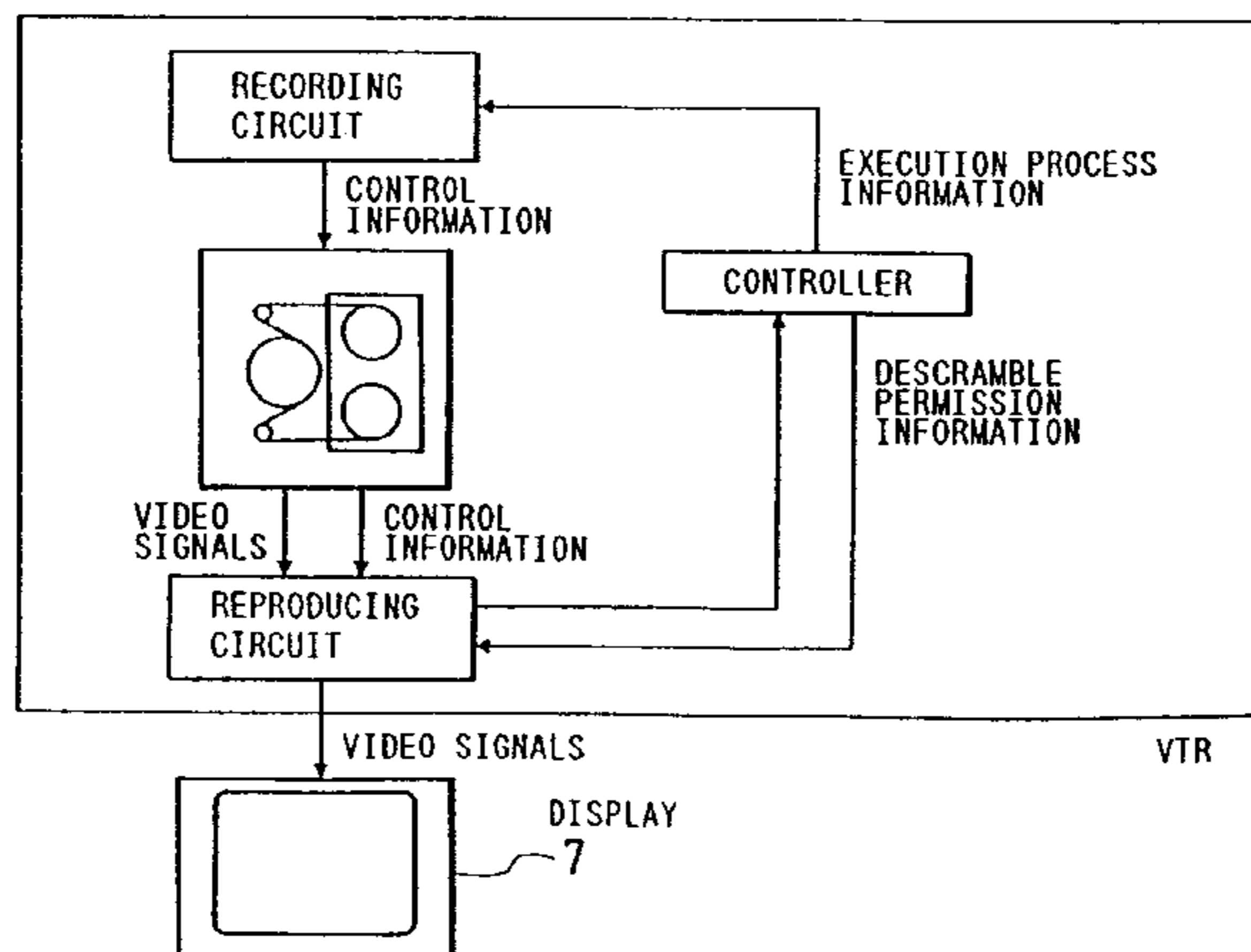
REPRODUCING SYSTEM
