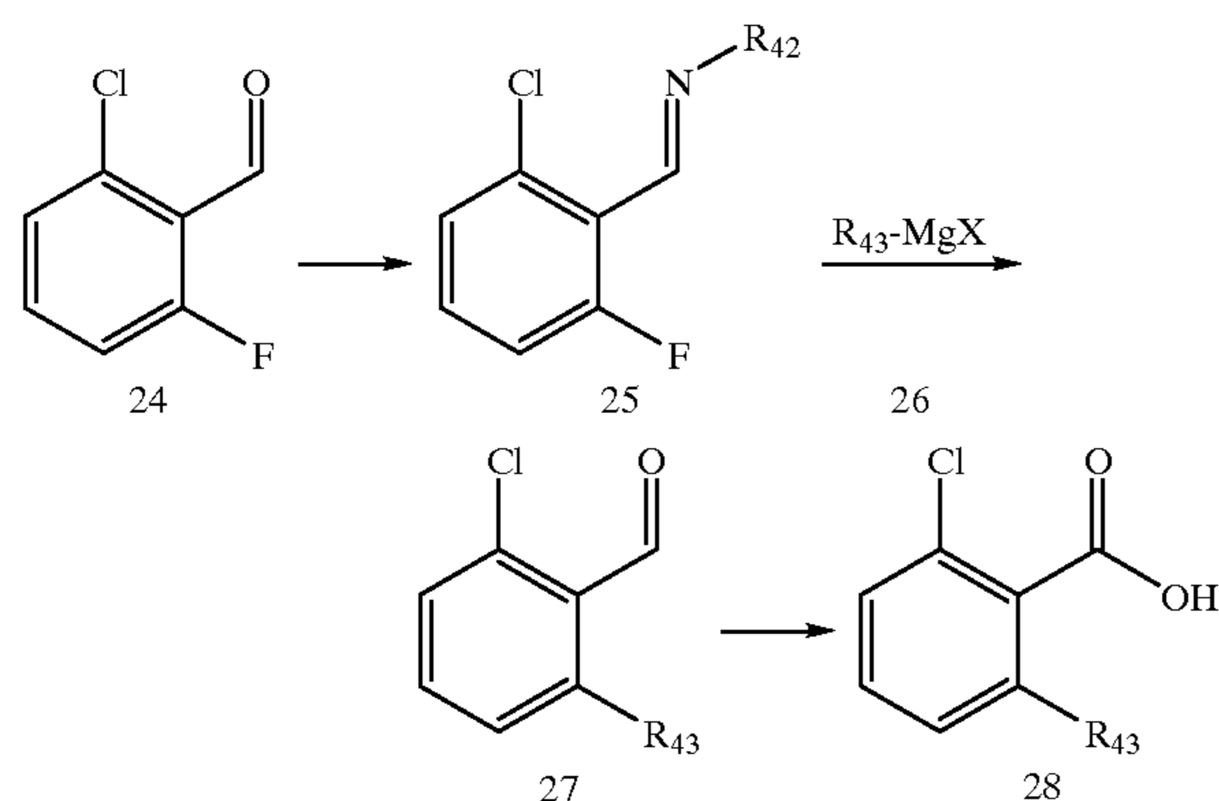
Reaction Scheme 8
