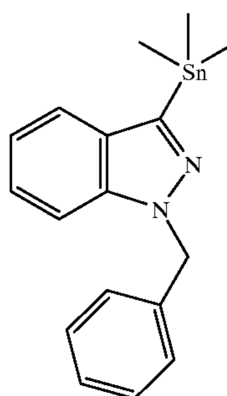
1-Benzyl-3-trimethylstannyl-indazole
