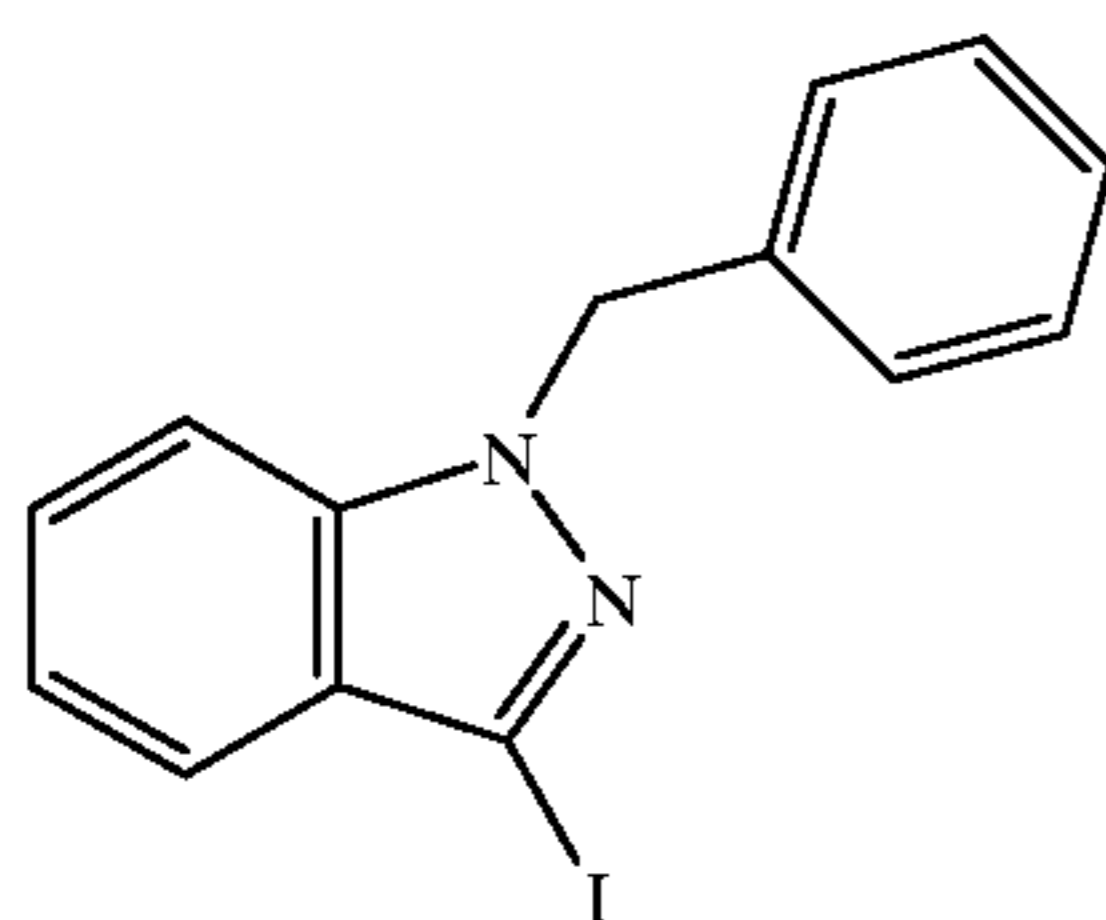
1-Benzyl-3-iodoindazole
