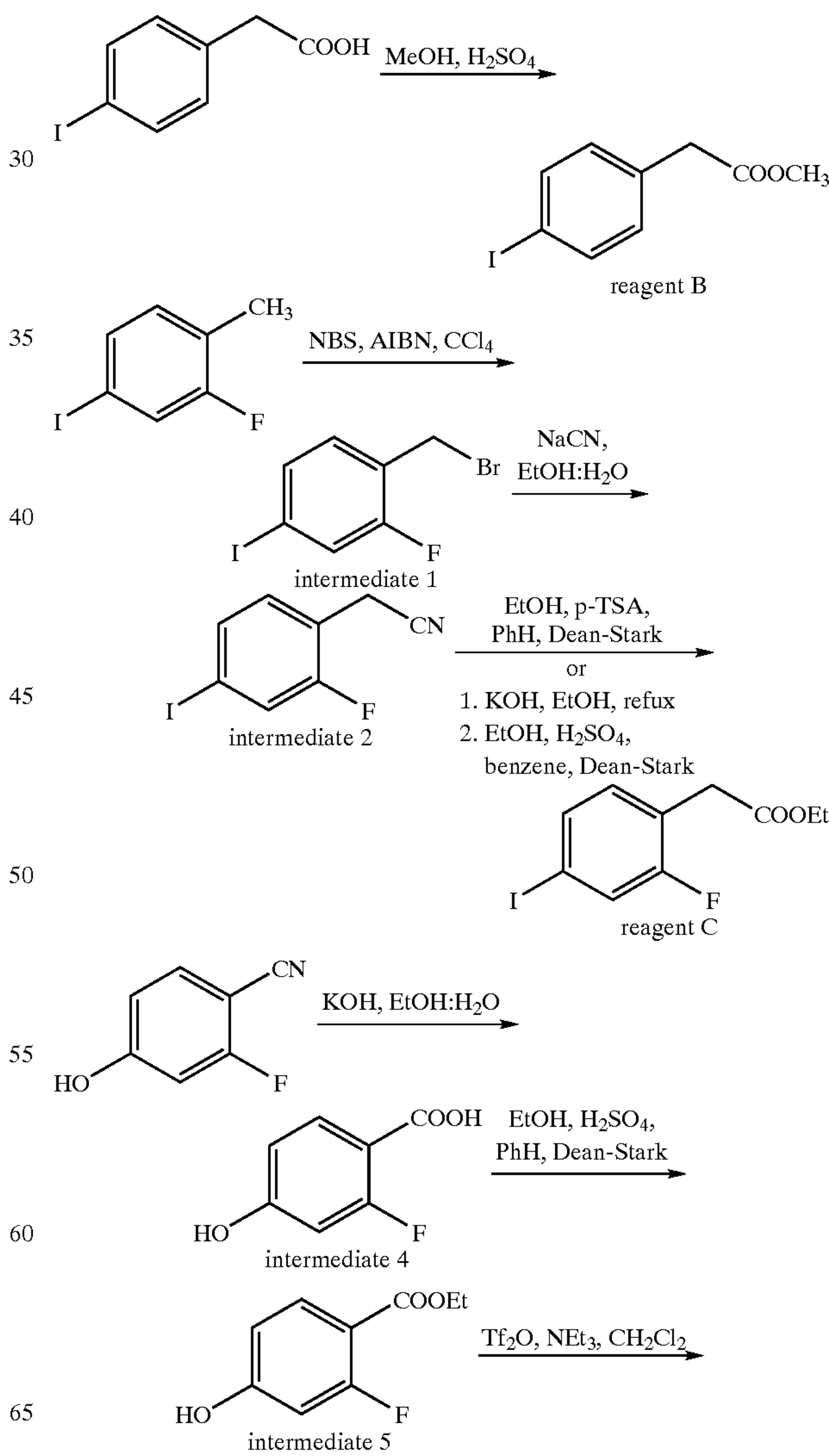
REACTION SCHEME 1
