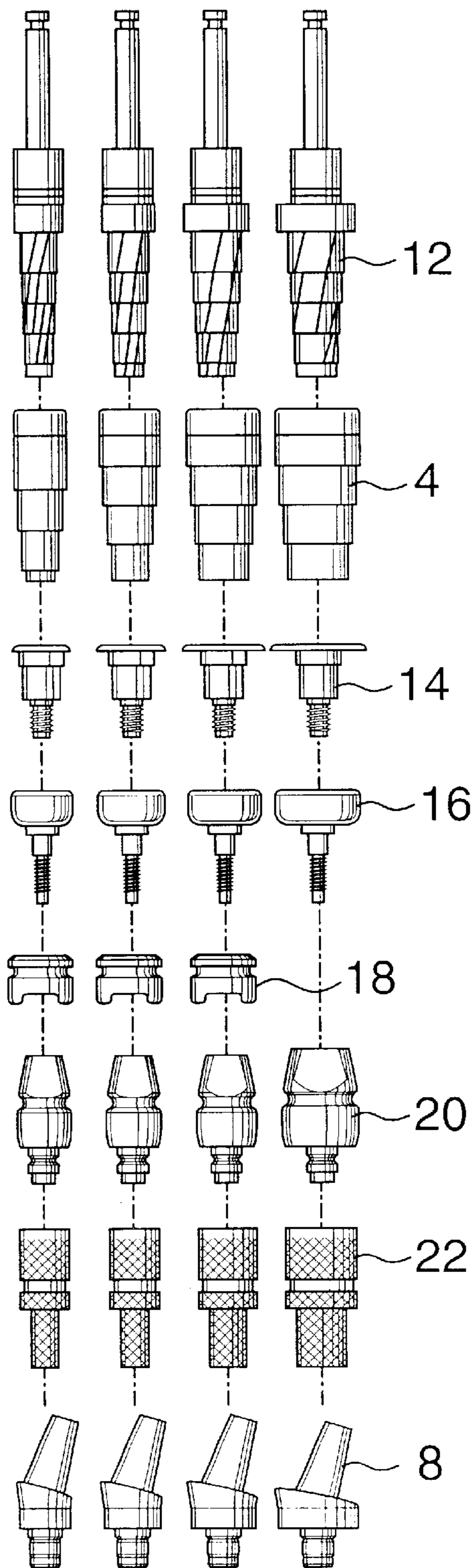
FIG. 2 PRIOR ART
