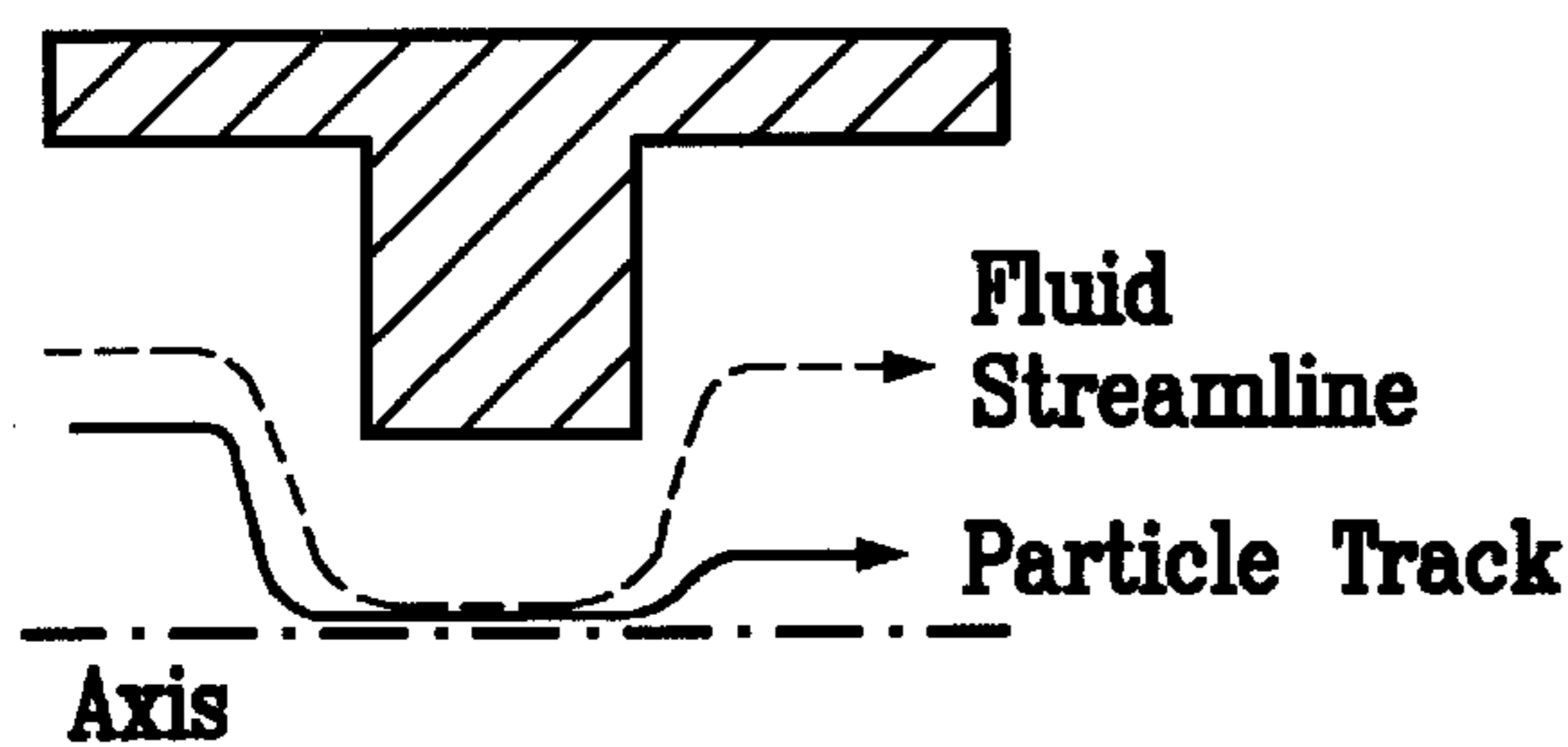
Aerodynamic Lens
