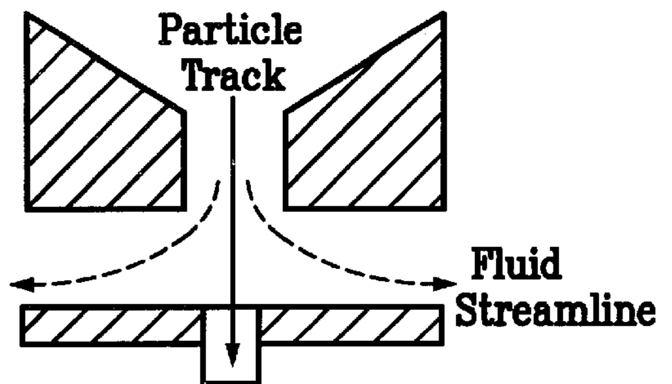
Virtual Impactor
