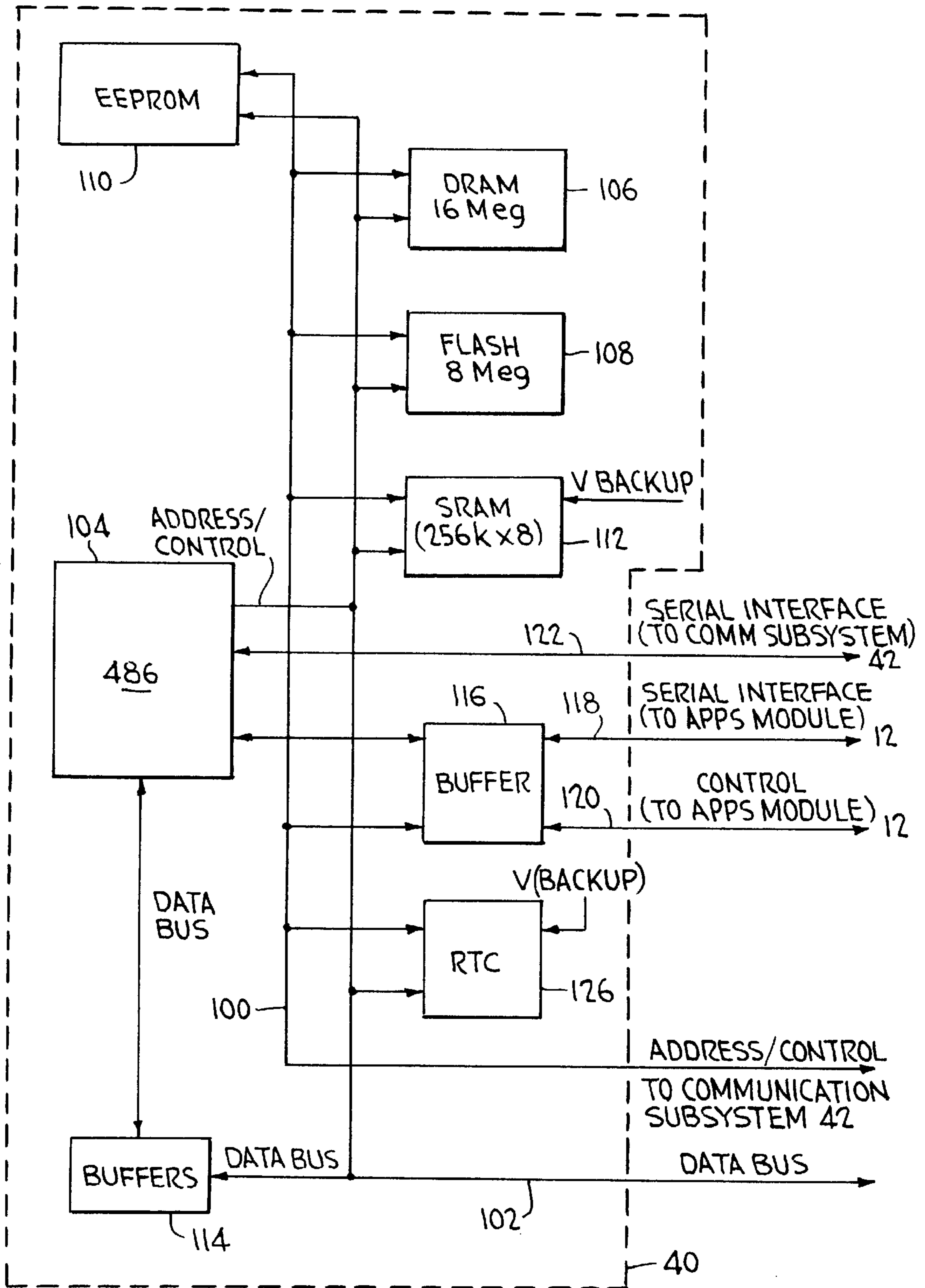
FIG. 3 PROCESSOR SUBSYSTEM
