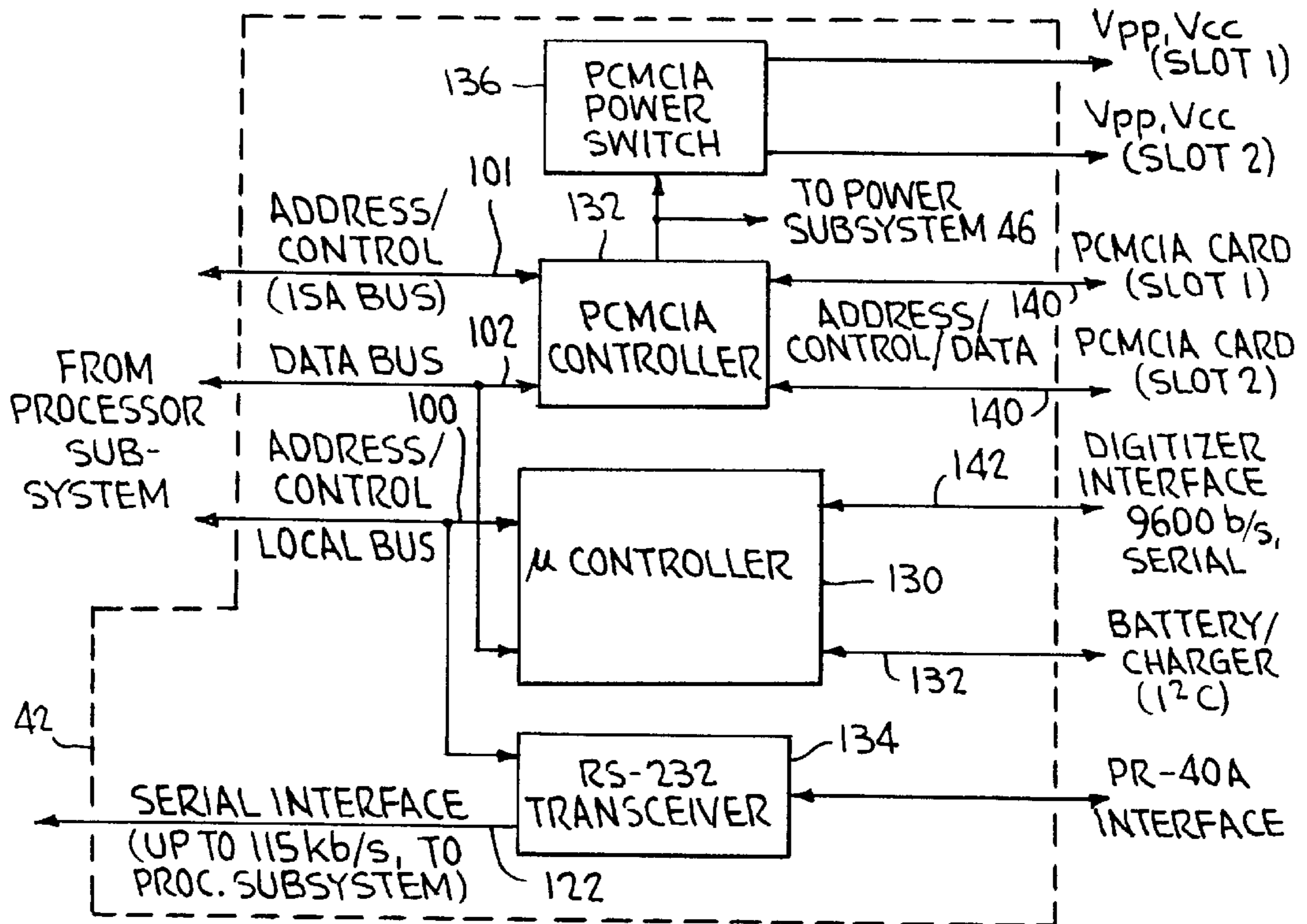
FIG. 4 COMMUNICATION SUBSYSTEM
