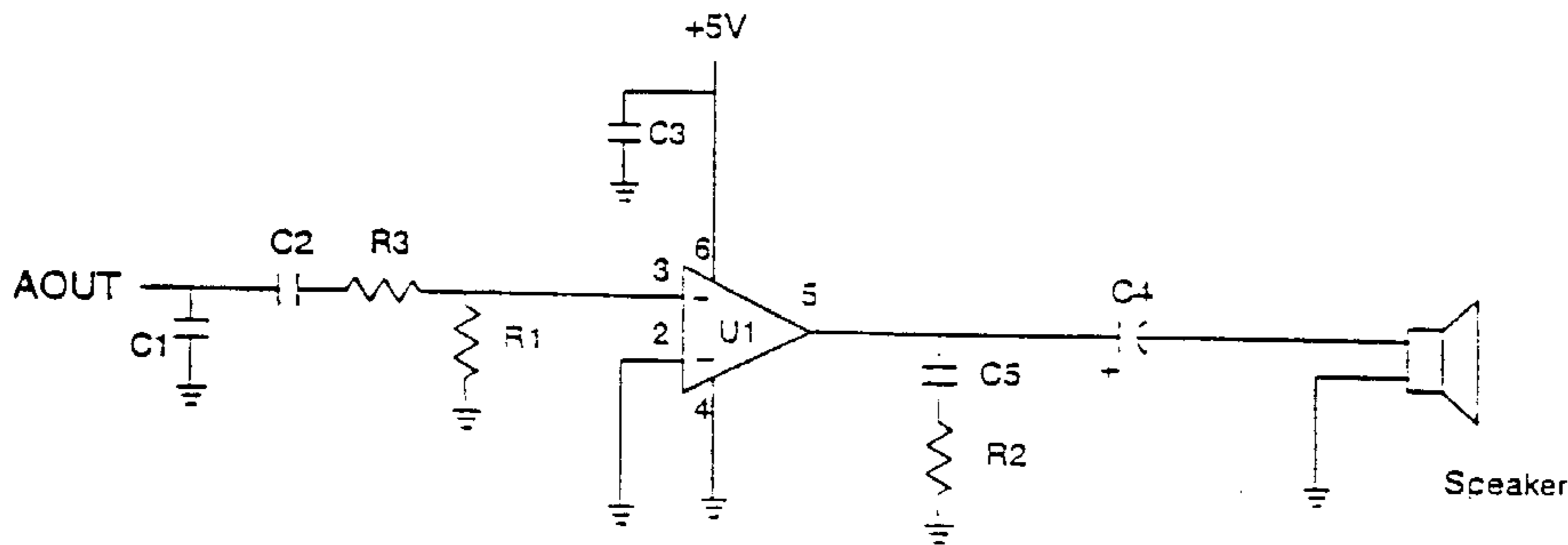
Figure 9. Optional Connection to AOOUT For a Call Progress Speaker
