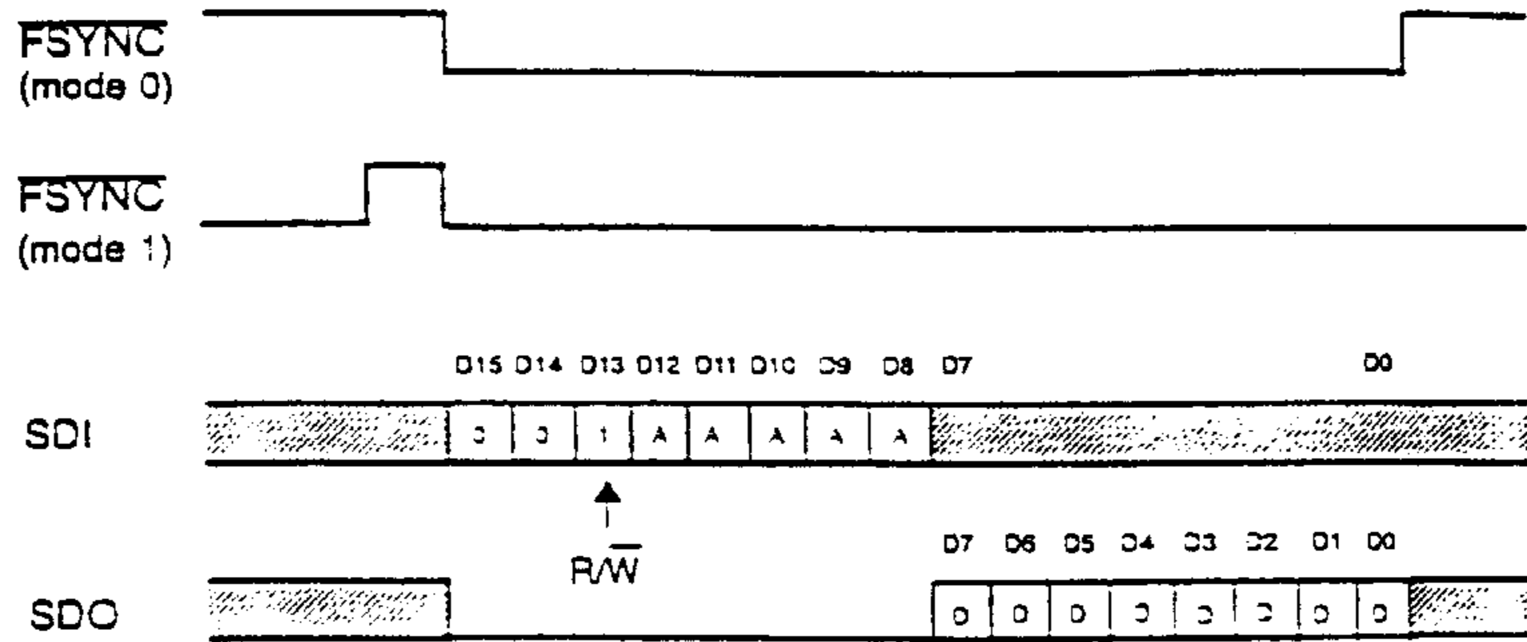
Figure 14. Secondary Communication Data Format—Read Cycle
