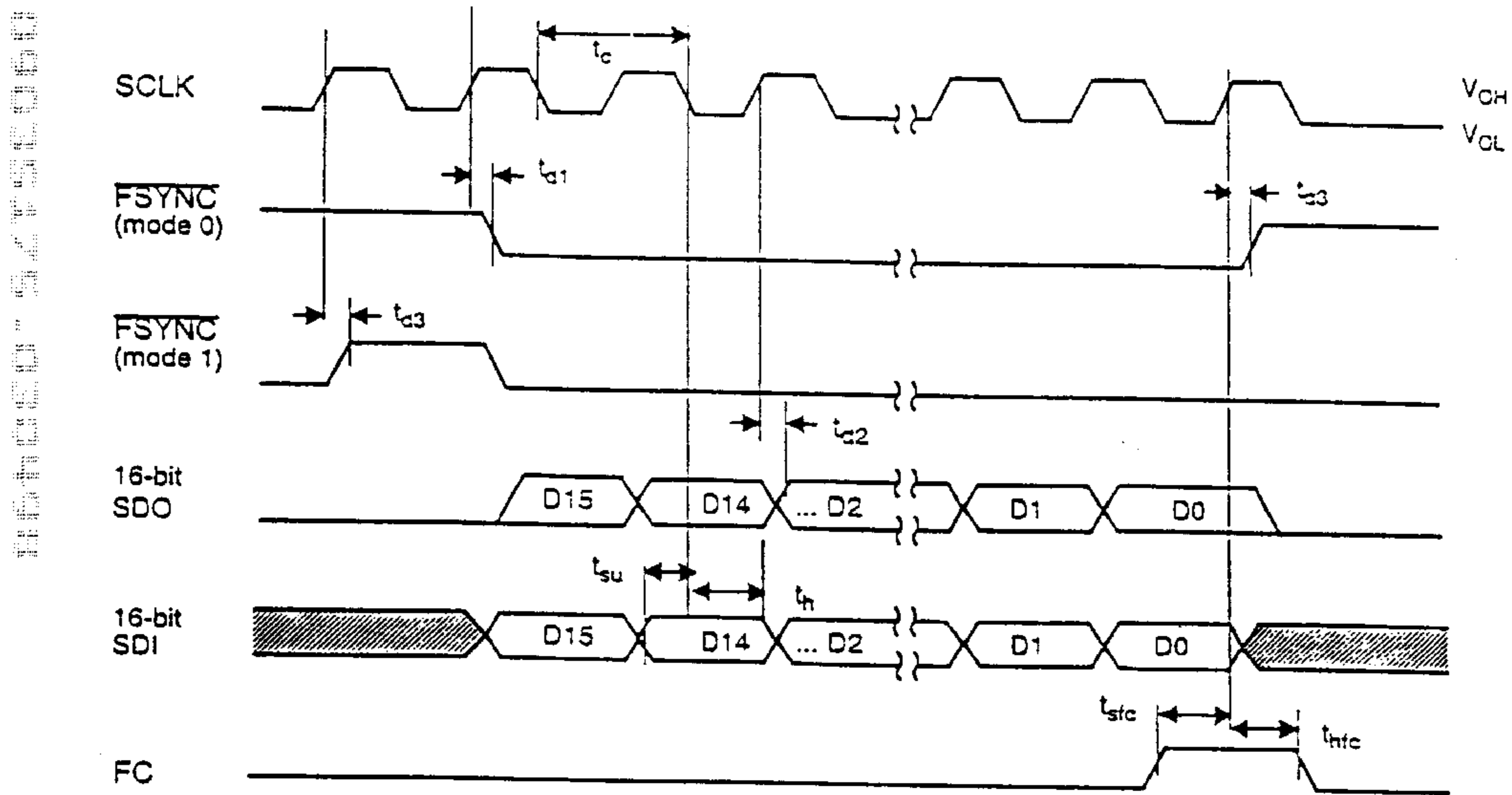
Figure 2. Serial Interface Timing Diagram
