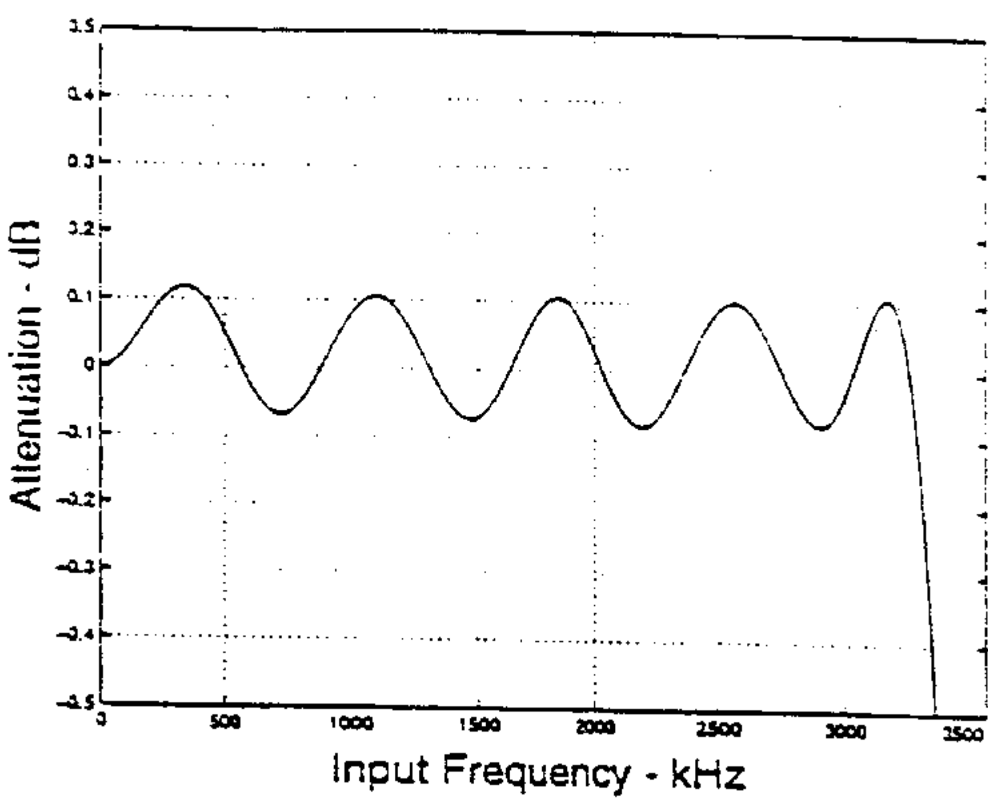
Figure 7. Interpolation Filter Passband Ripple
