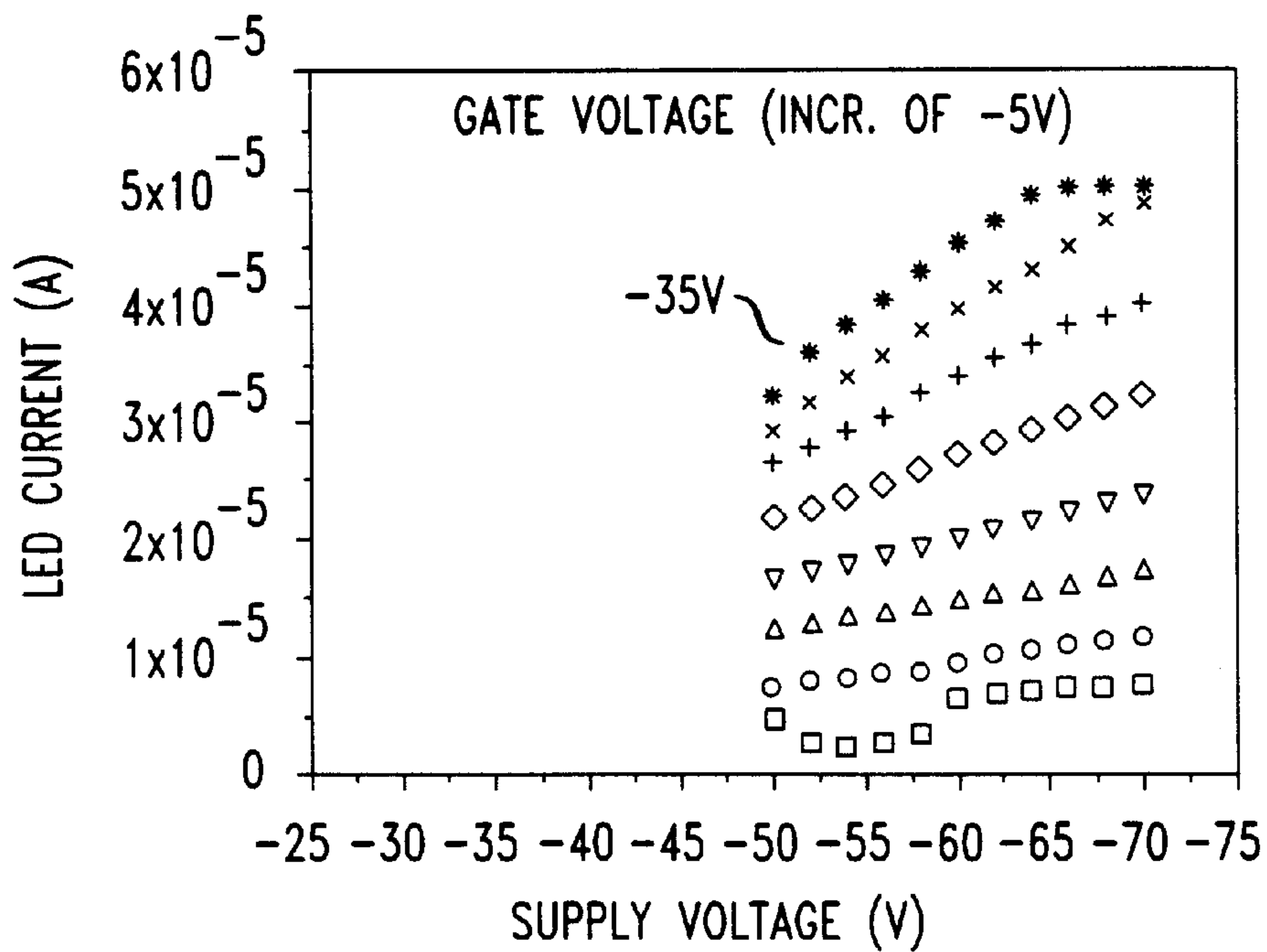
FIG. 2 (PRIOR ART)
