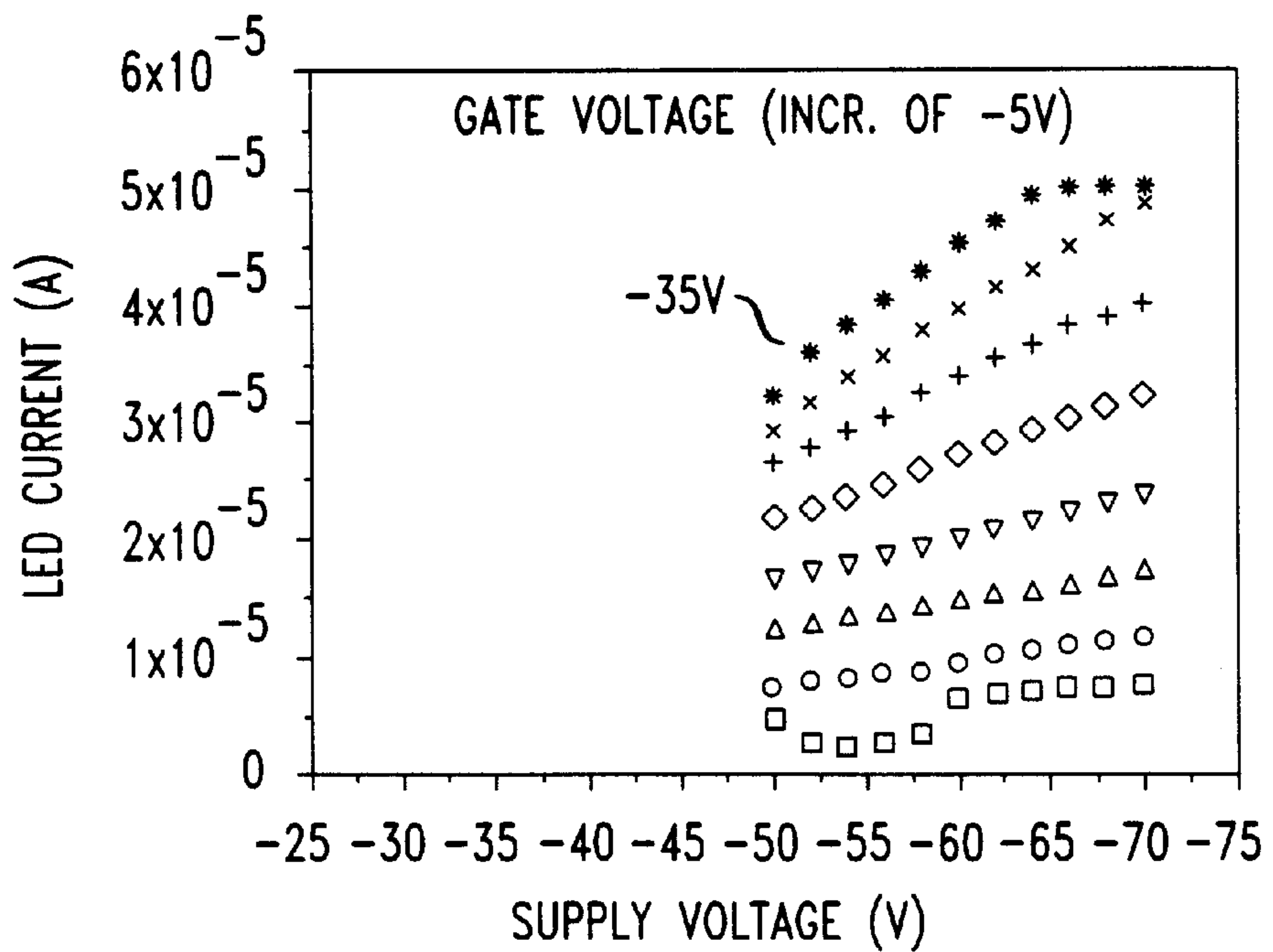
FIG. 2 (PRIOR ART)
