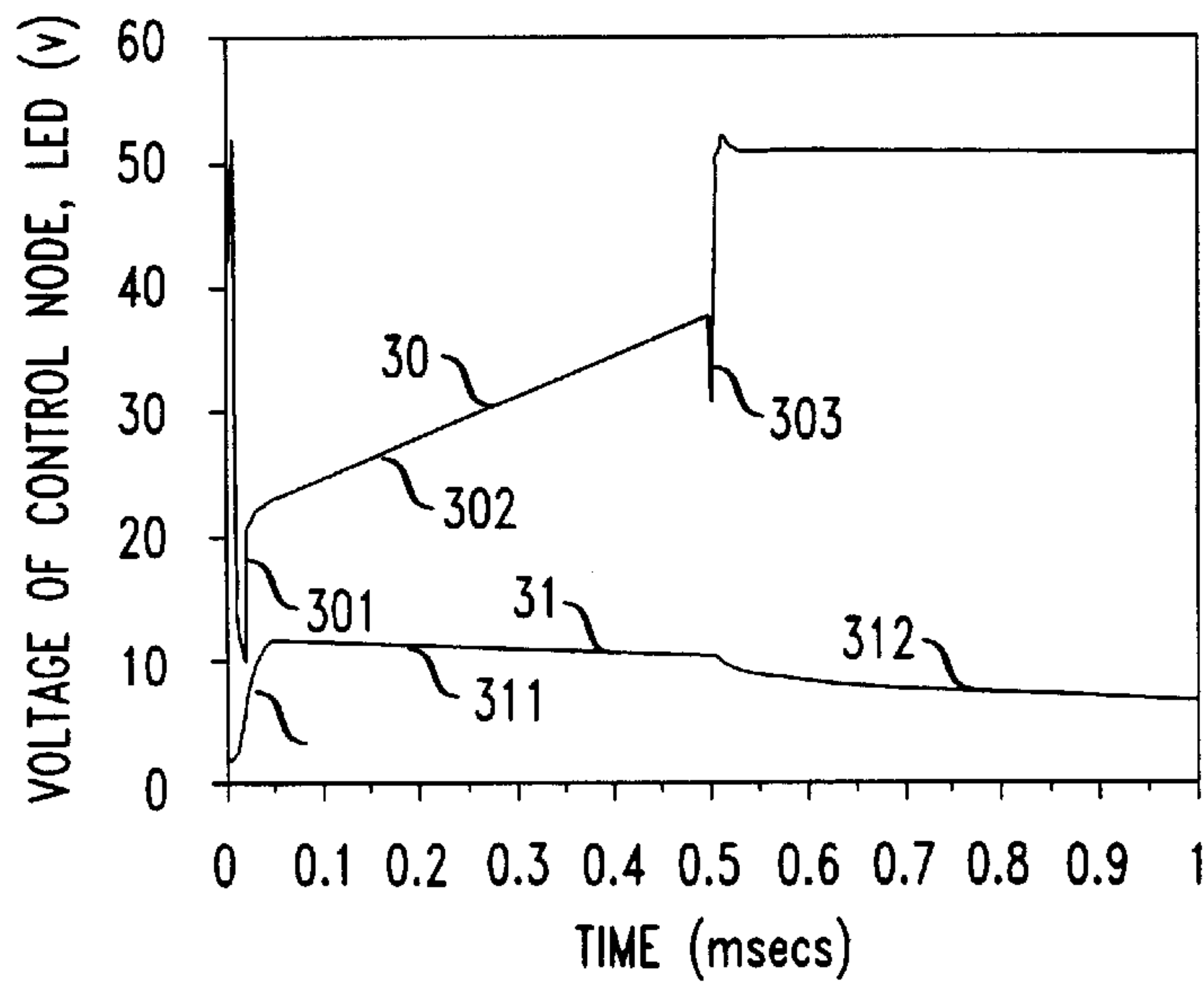
FIG. 3 (PRIOR ART)
