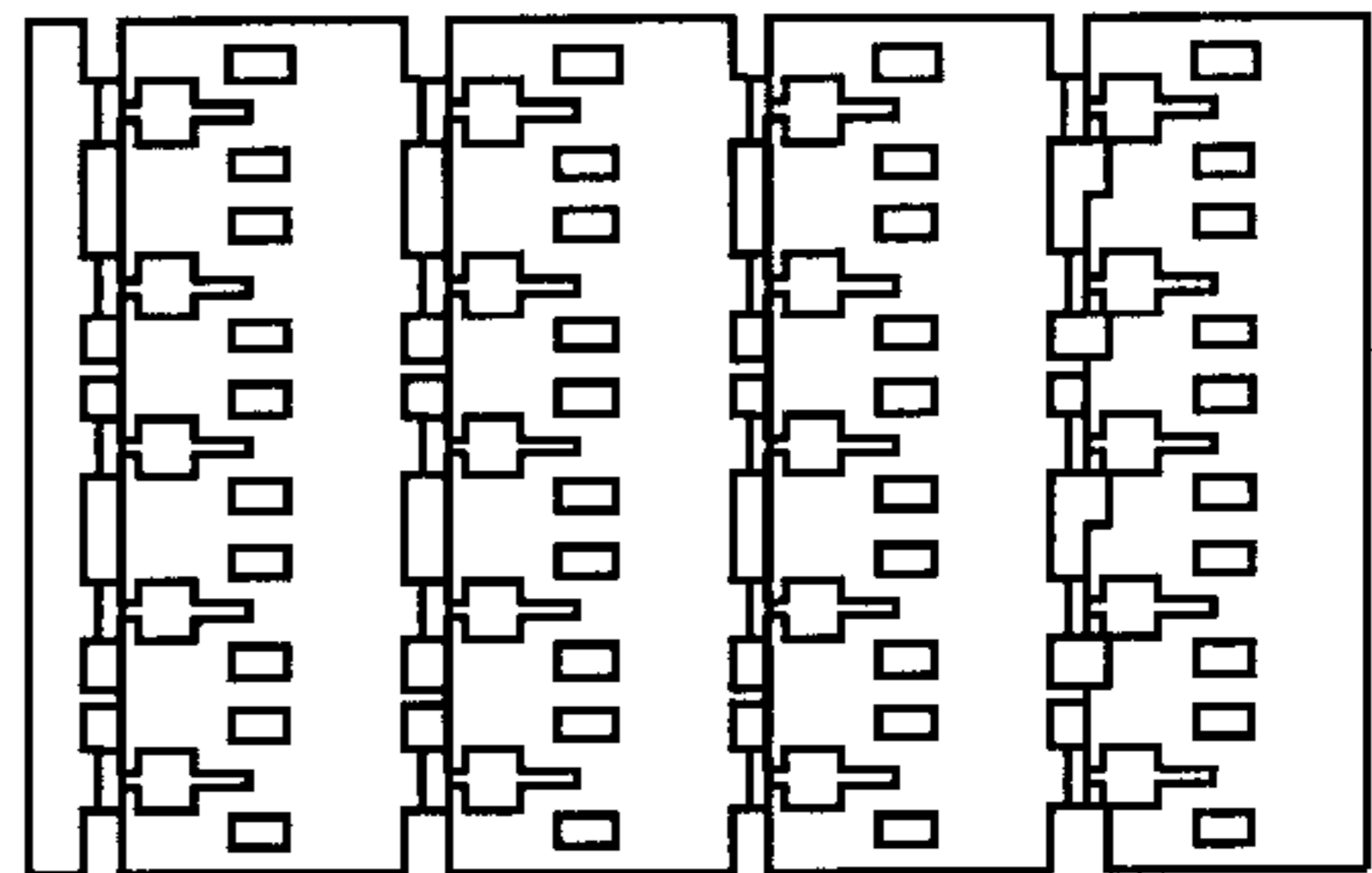
FIG. 3b 2-D BEAM STEERING BEAM STEERING ARRAY
