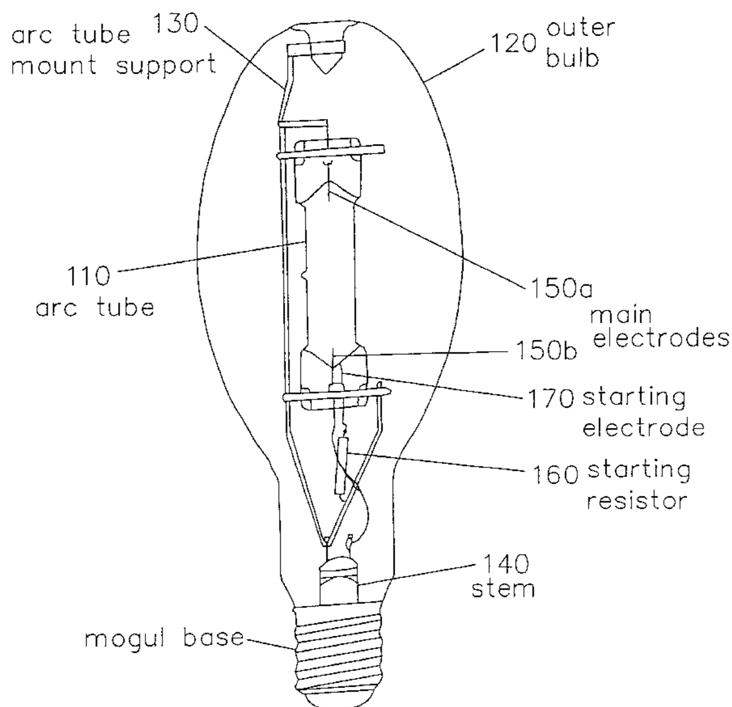
High—pressure mercury—vapor lamp
