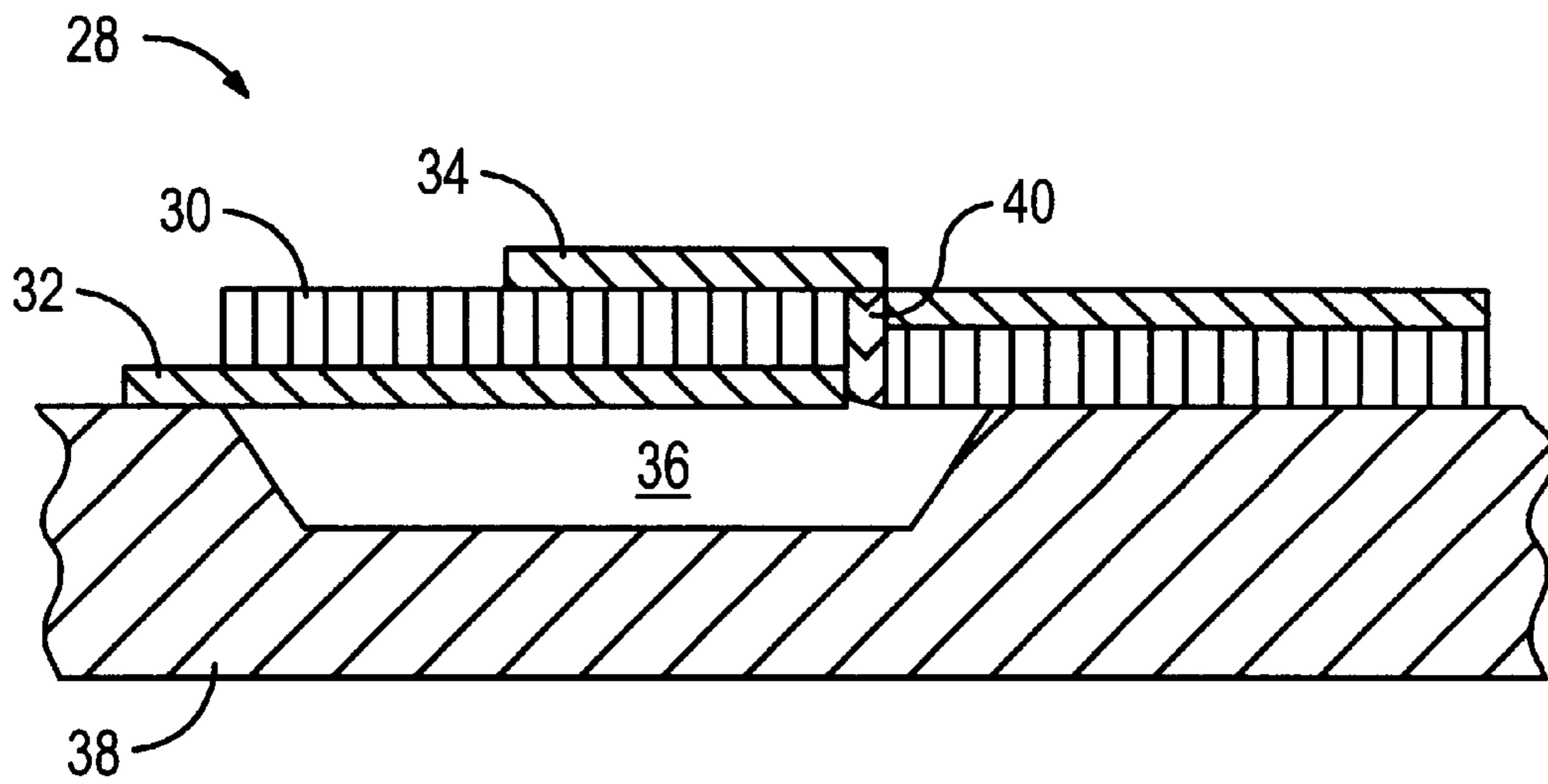
FIG. 3 (PRIOR ART)
